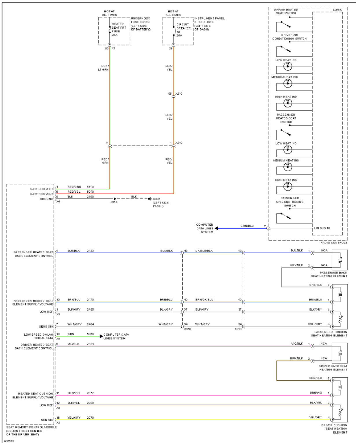
Fig. 105: Heated Seats Circuit, W/ Memory
