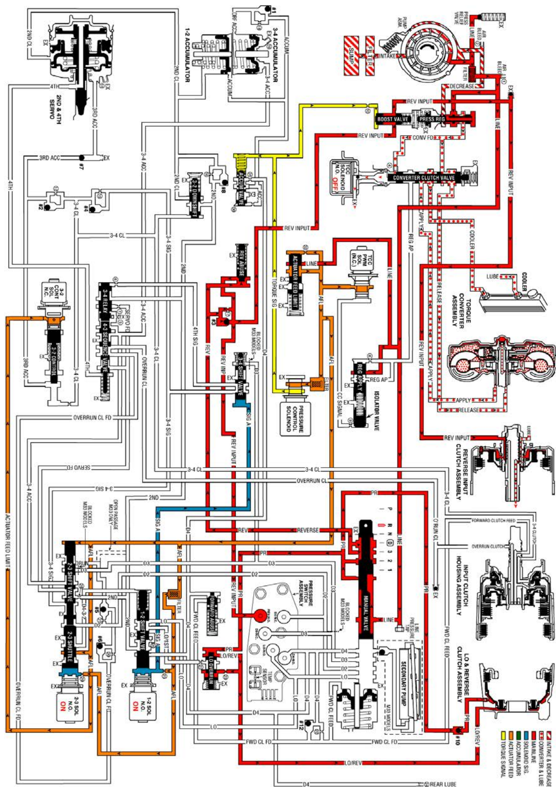
Fig. 2: Reverse Courtesy of GENERAL MOTORS CORP.
