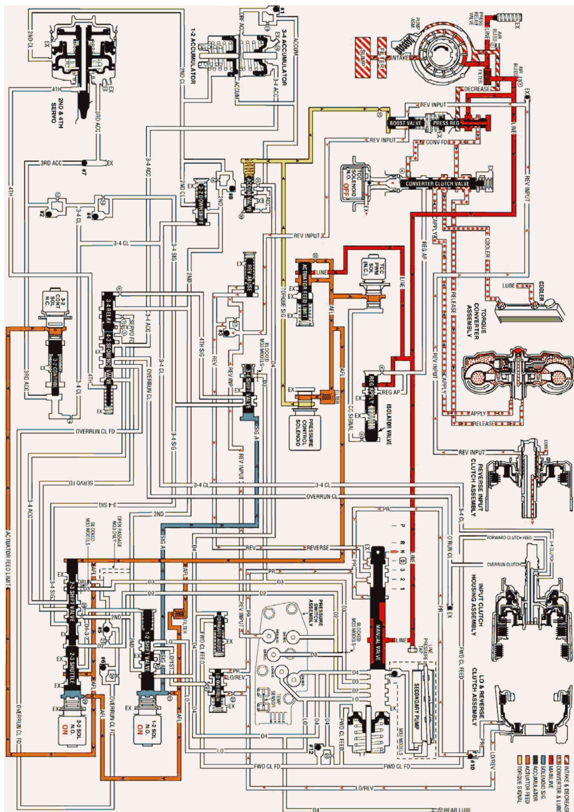
Fig. 3: Neutral - Engine Running Courtesy of GENERAL MOTORS CORP.
