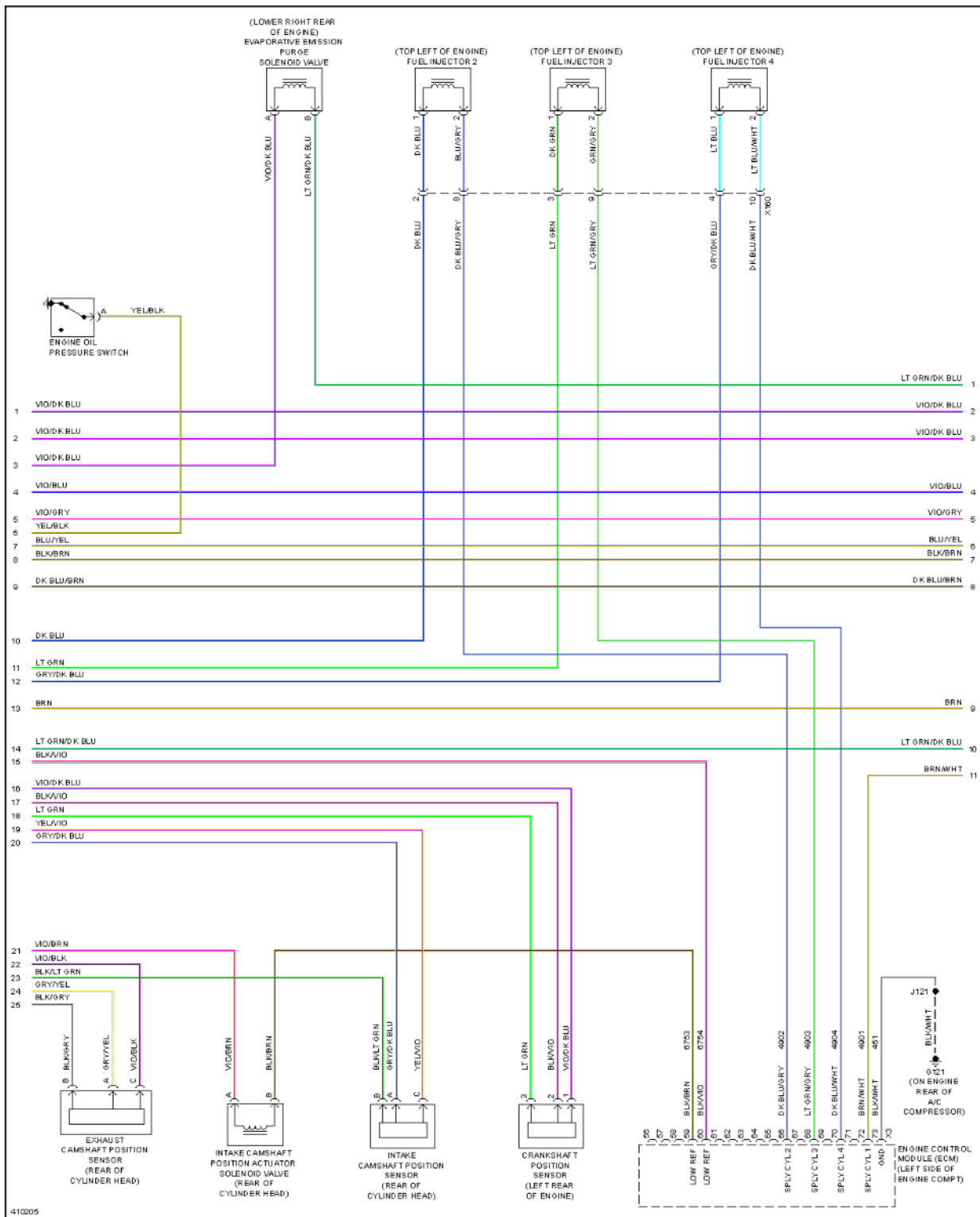
Fig. 38: 2.4L VIN R, Engine Controls Circuit (4 of 6)
