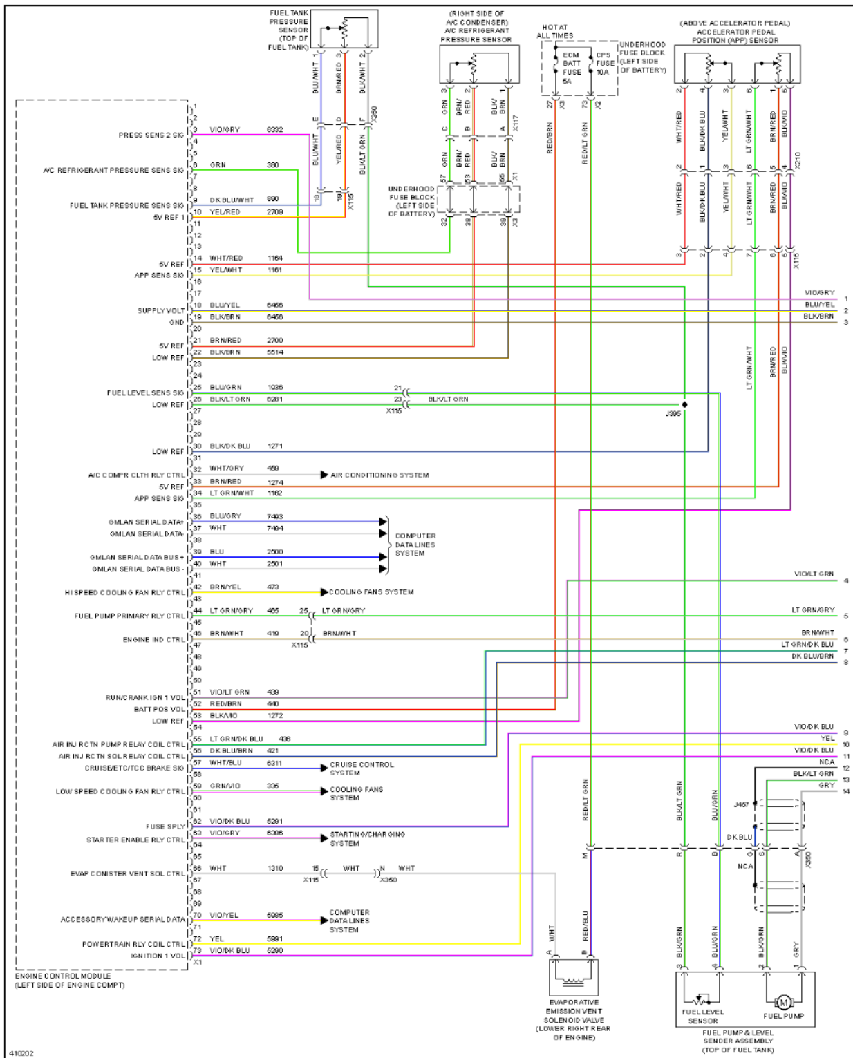
Fig. 35: 2.4L VIN R, Engine Controls Circuit (1 of 6)
