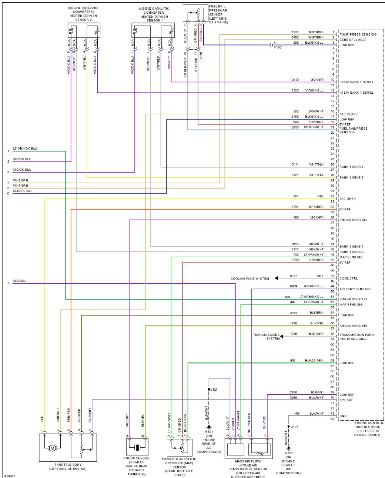
Fig. 40: 2.4L VIN R, Engine Controls Circuit (6 of 6)
