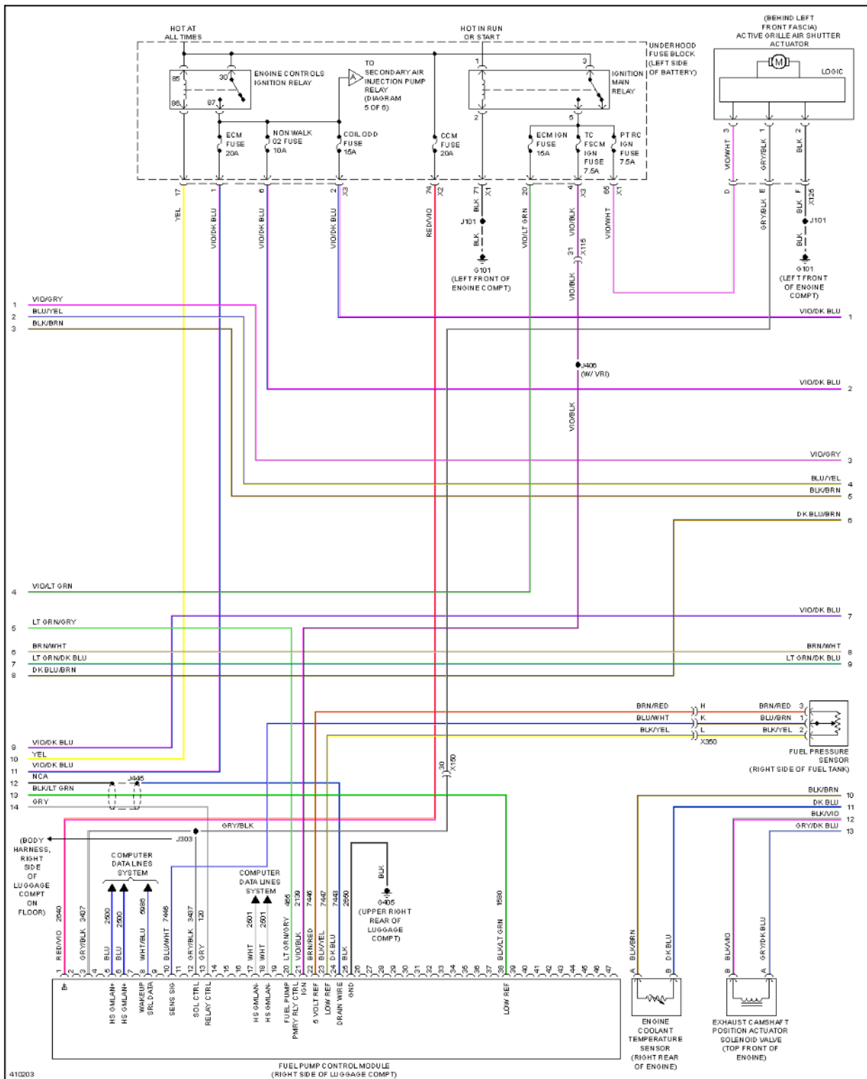
Fig. 36: 2.4L VIN R, Engine Controls Circuit (2 of 6)
