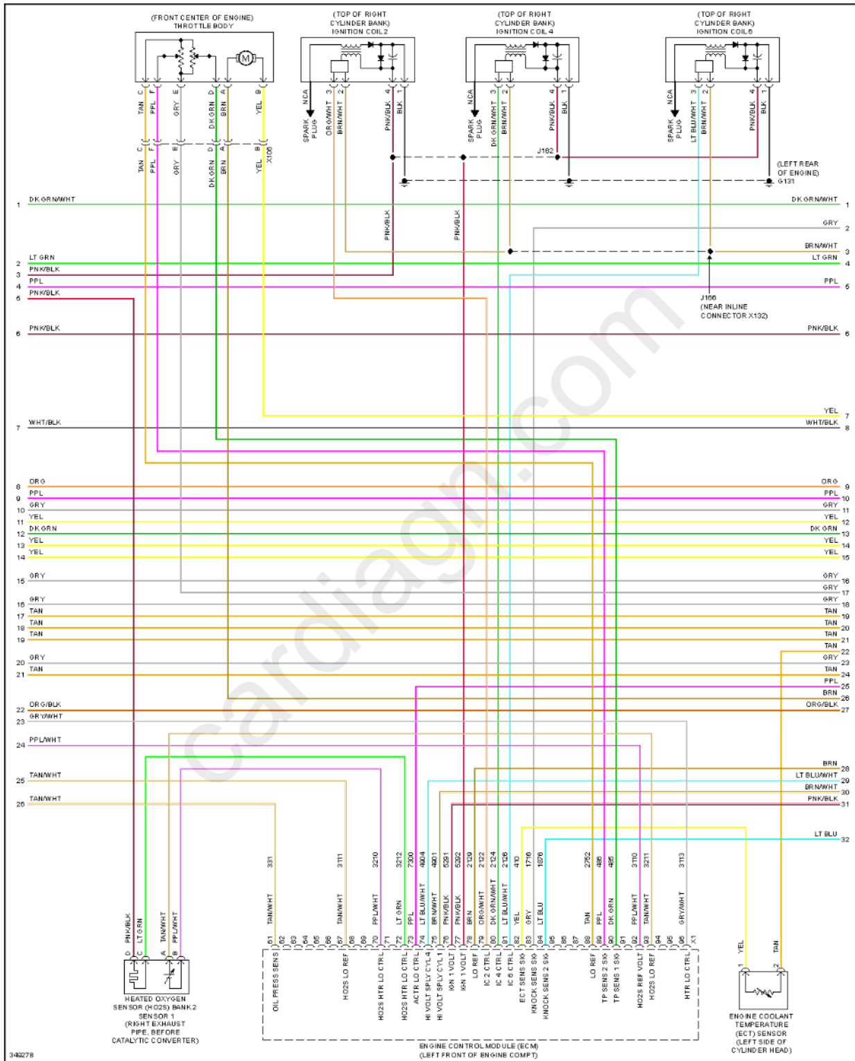
Fig. 34: 3.6L VIN D, Engine Performance Circuit (4 of 5)
