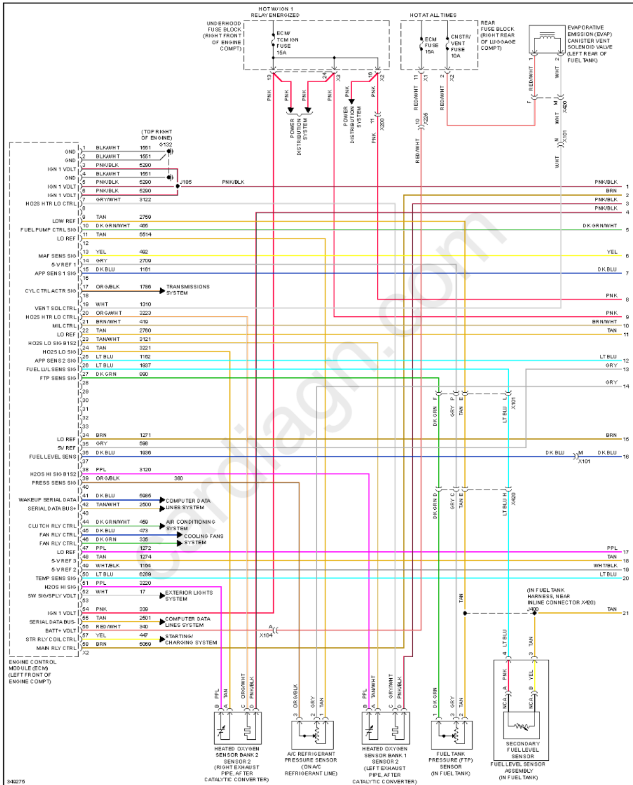
Fig. 31: 3.6L VIN D, Engine Performance Circuit (1 of 5)
