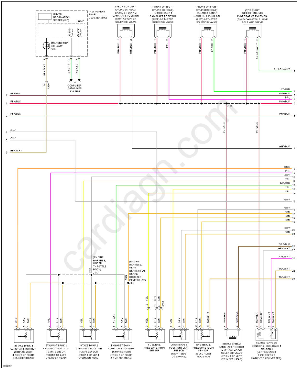
Fig. 33: 3.6L VIN D, Engine Performance Circuit (3 of 5)
