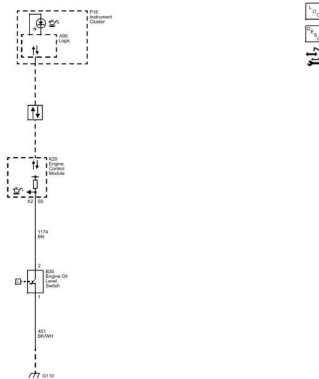
Fig. 1: Oil Level Sensor Wiring Schematics Courtesy of GENERAL MOTORS COMPANY
