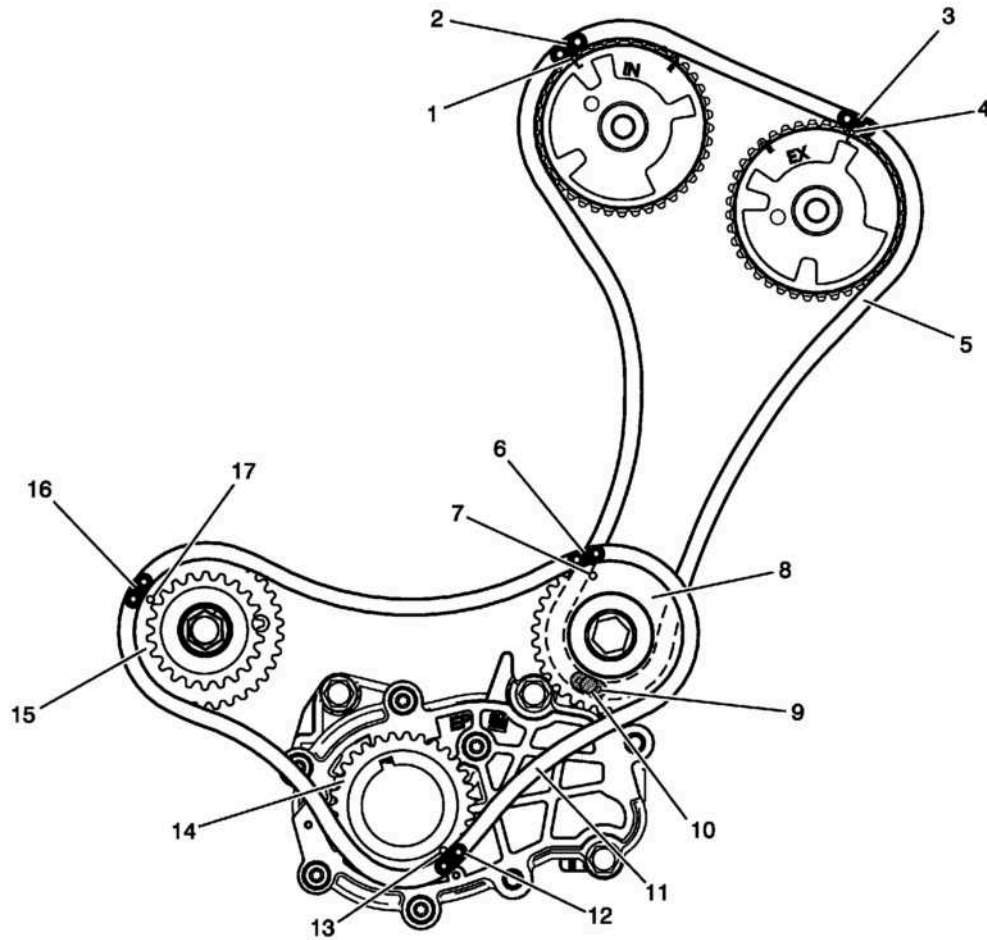
Fig. 3: Locating Stage One Timing Marks Courtesy of GENERAL MOTORS COMPANY
