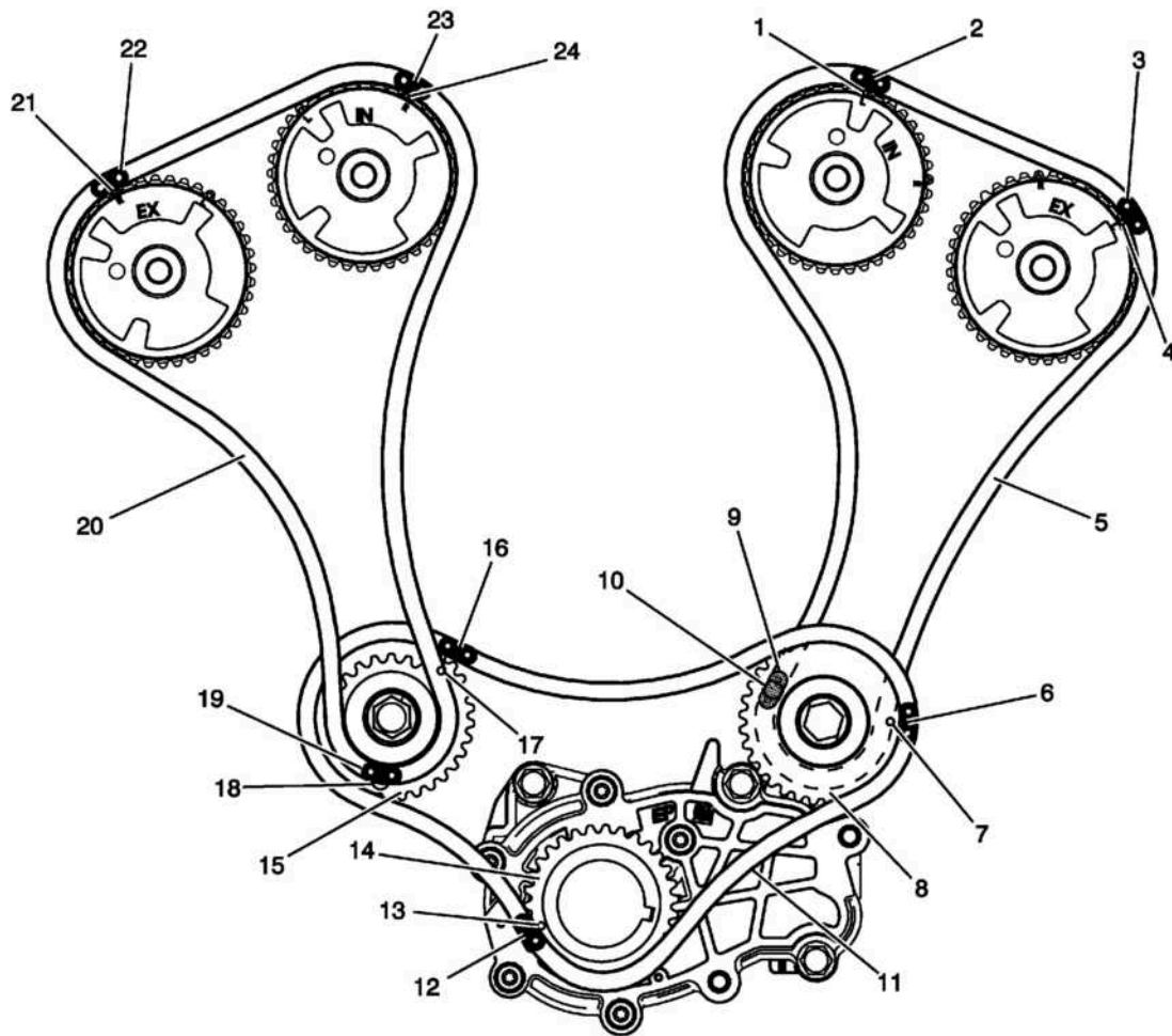
Fig. 4: Locating Stage Two Timing Marks Courtesy of GENERAL MOTORS COMPANY
