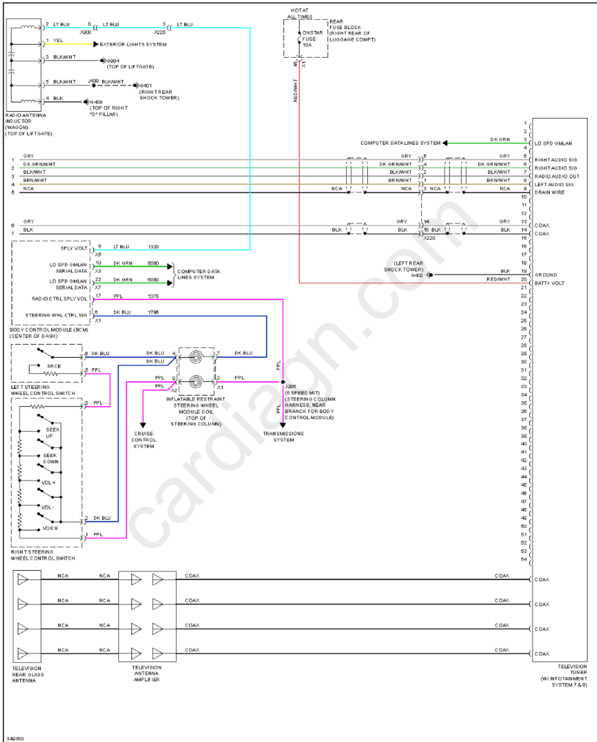
Fig. 70: Navigation Circuit, W/O Surround Amplifier (4 of 4)
