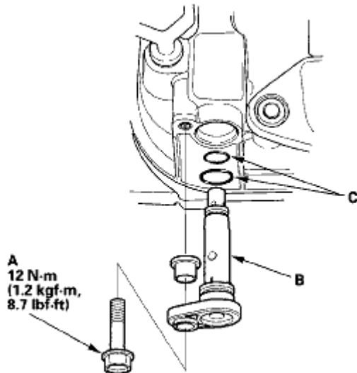
Fig. 4: Identifying PCV Valve And Bolt With Torque Specification Courtesy of AMERICAN HONDA MOTOR CO., INC.
