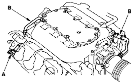
Fig. 2: Identifying PCV Valve And Hoses Courtesy of AMERICAN HONDA MOTOR CO., INC.
