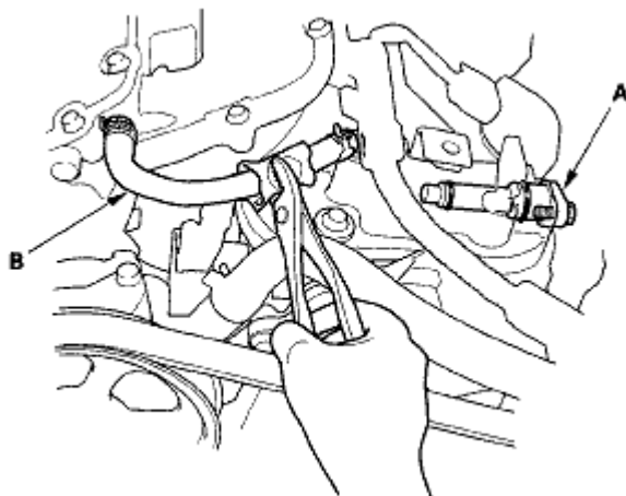
Fig. 3: Pinching PCV Hose Courtesy of AMERICAN HONDA MOTOR CO., INC.
