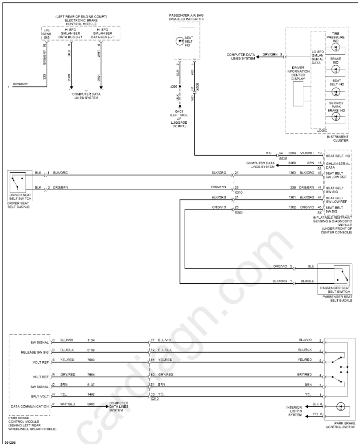
Fig. 133: Warning Systems Circuit (2 of 2)
