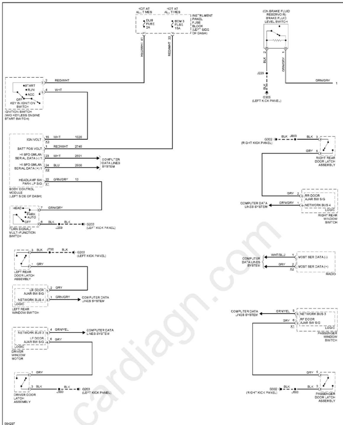
Fig. 132: Warning Systems Circuit (1 of 2)
