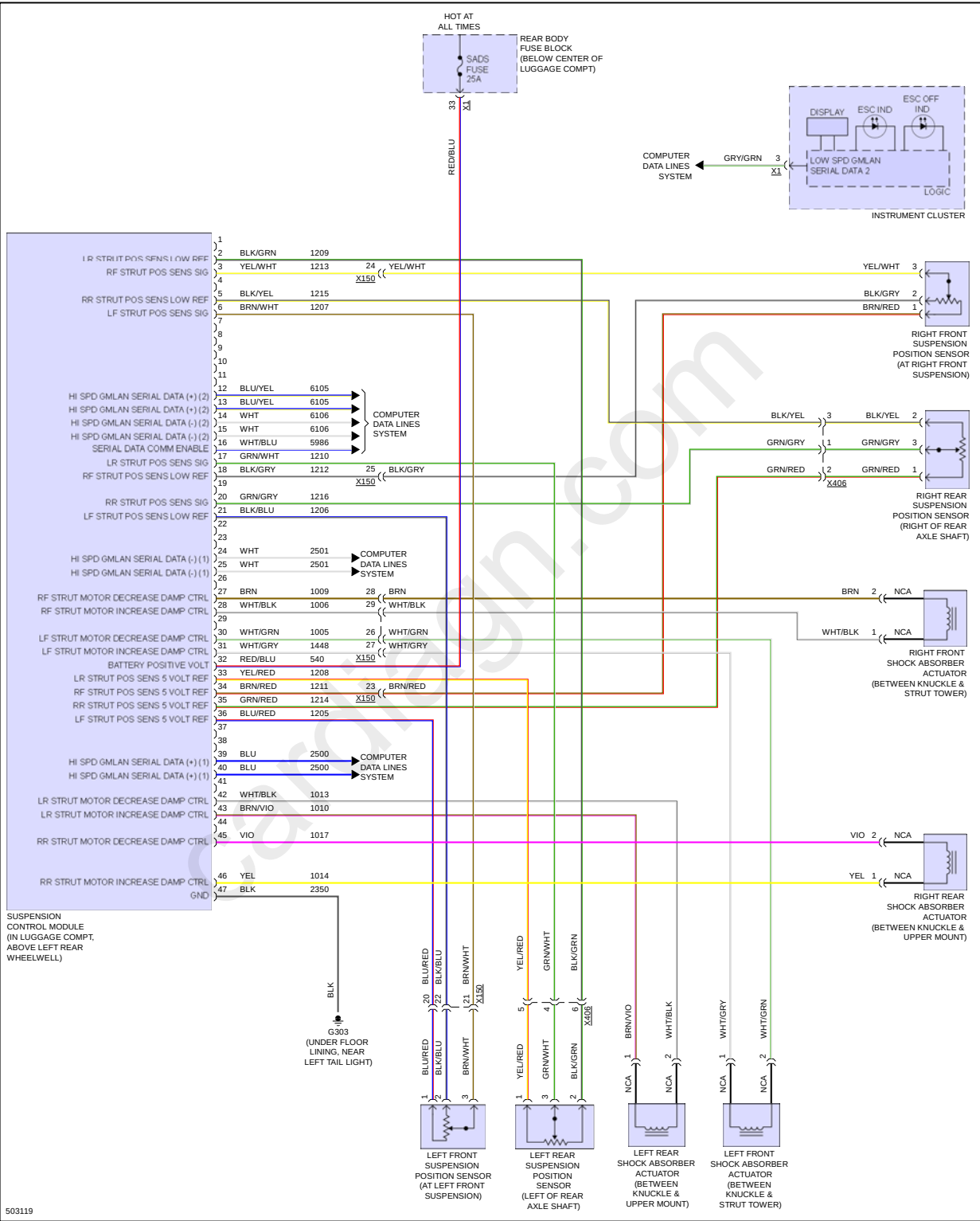
Fig 1: Electronic Suspension Circuit
