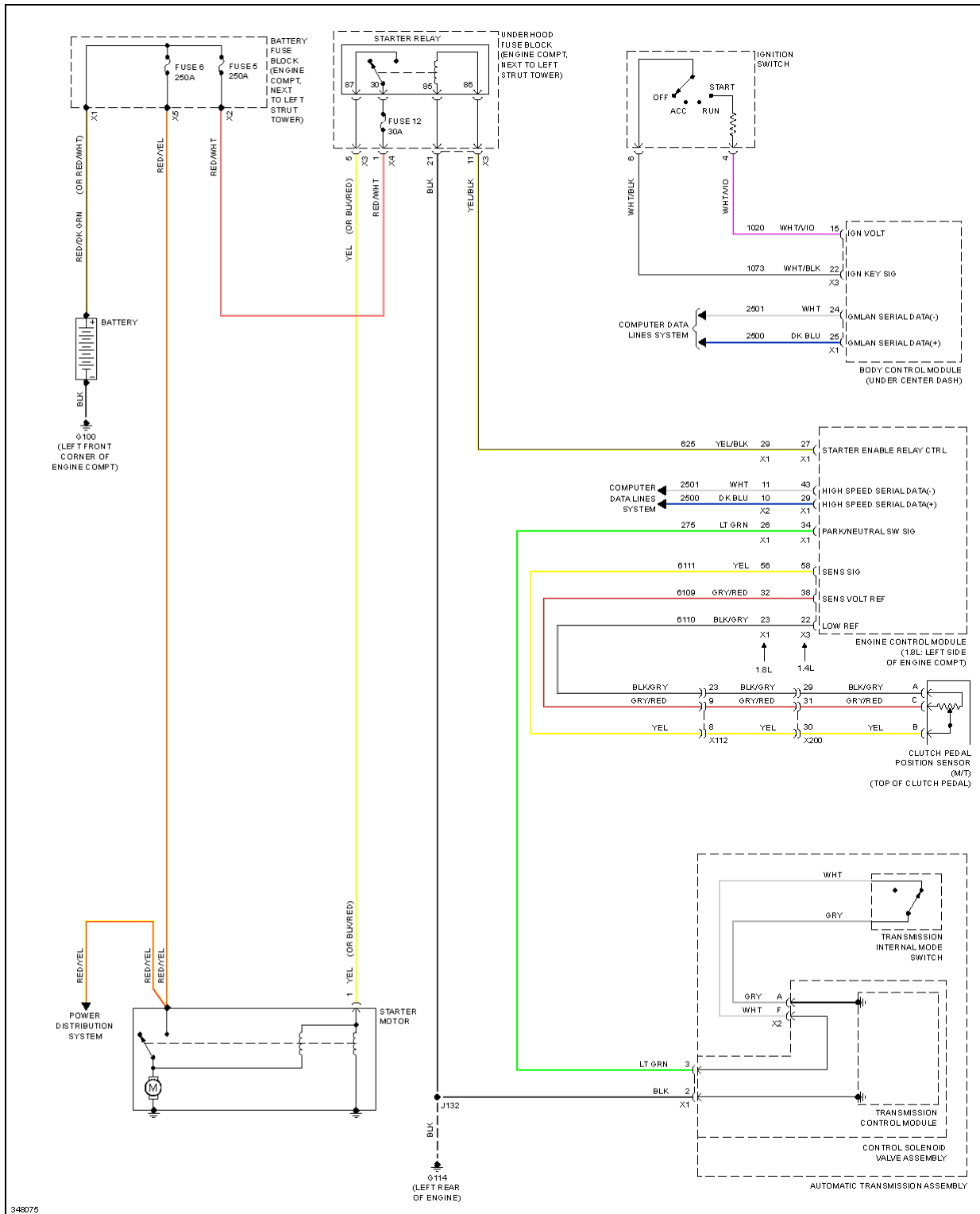
Fig. 70: Starting Circuit
