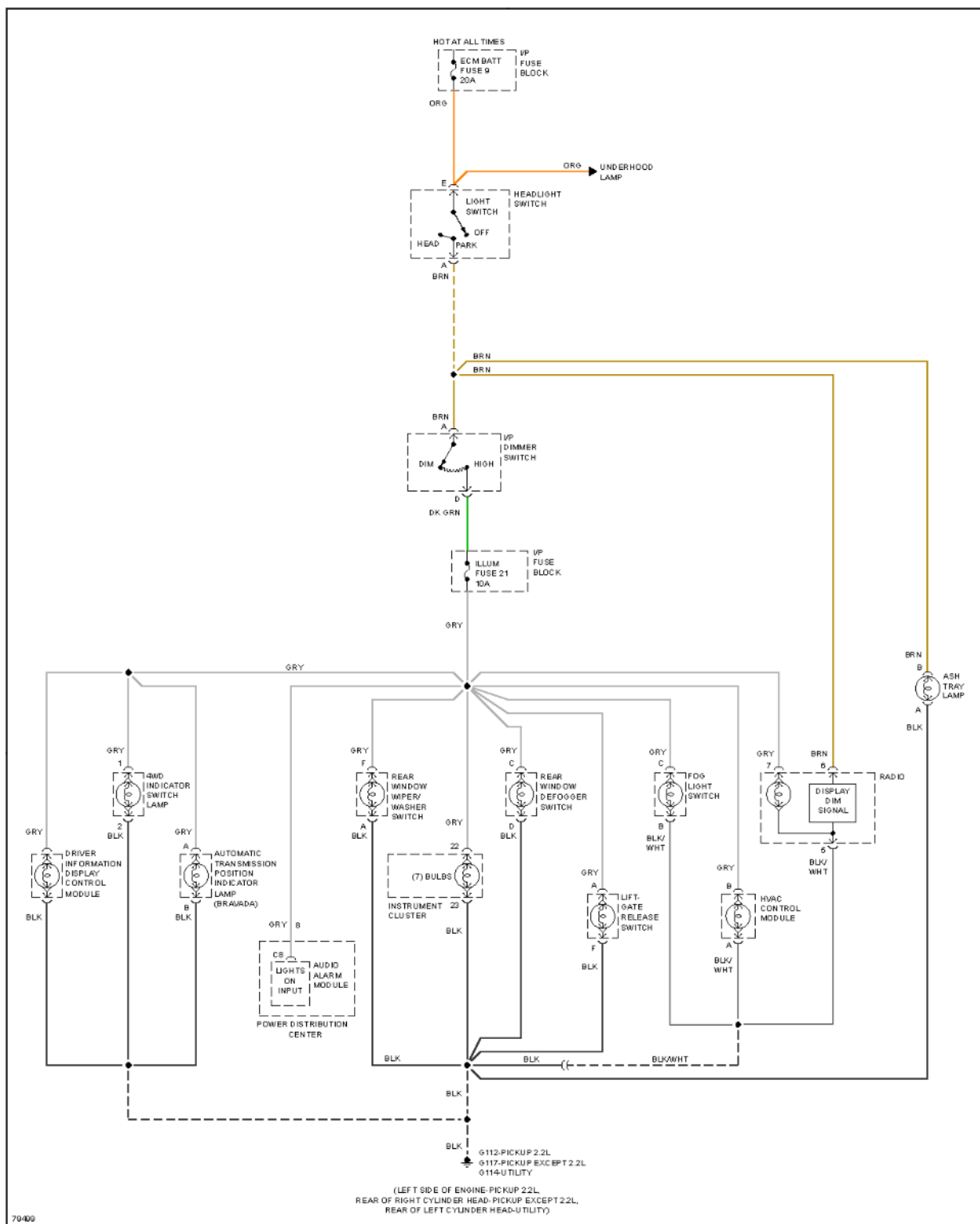
Fig. 18: Instrument Illumination Circuit
