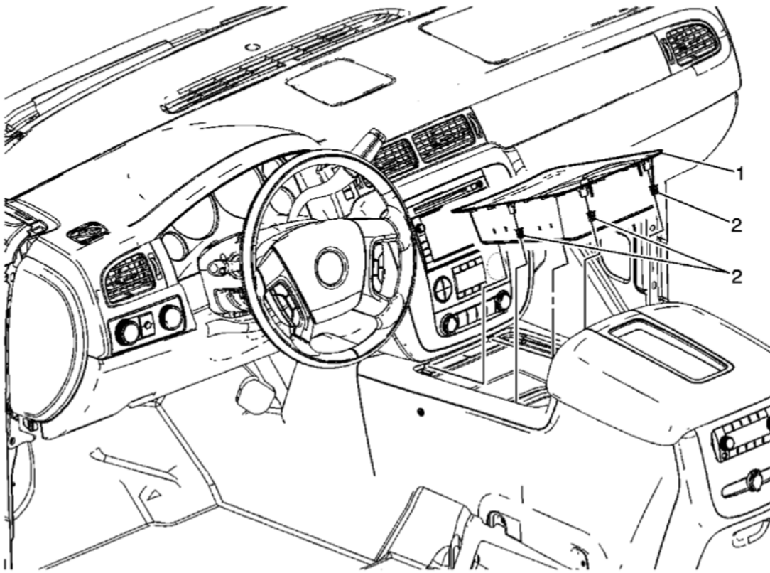
Fig. 46: View Of Front Floor Console Bezel Assembly & Clips Courtesy of GENERAL MOTORS CORP.
