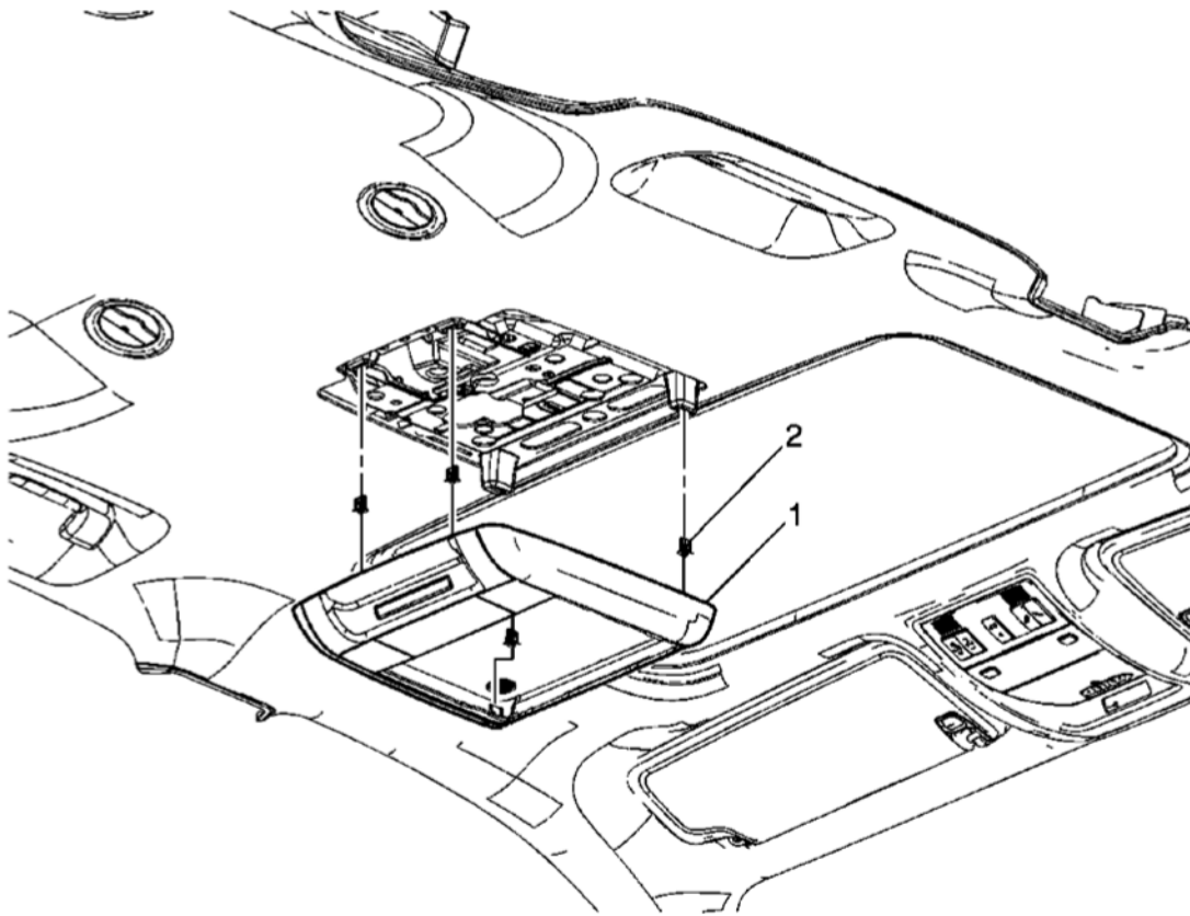
Fig. 56: View Of Roof Console Assembly & Retainers Courtesy of GENERAL MOTORS CORP.
