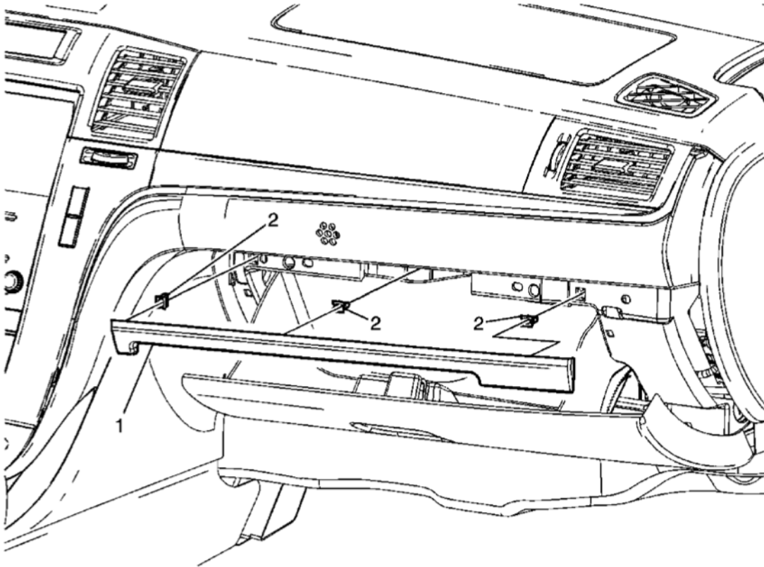
Fig. 24: View Of Instrument Panel Access Hole Cover & Clips Courtesy of GENERAL MOTORS CORP.
