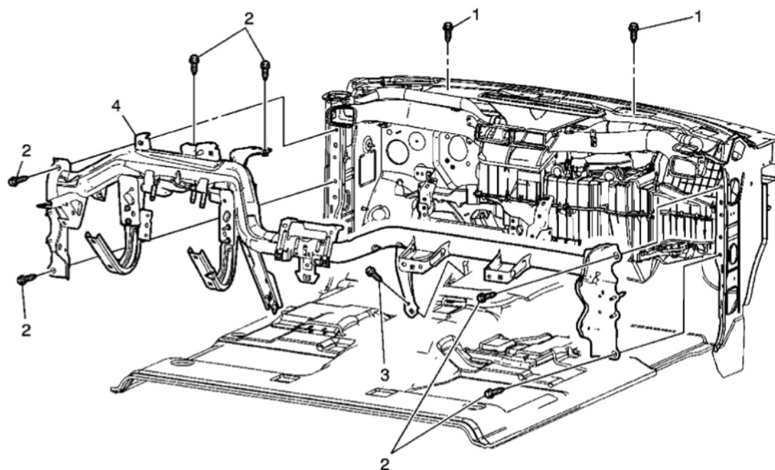
Fig. 36: View Of Instrument Panel Carrier Support Assembly & Bolts Courtesy of GENERAL MOTORS CORP.
