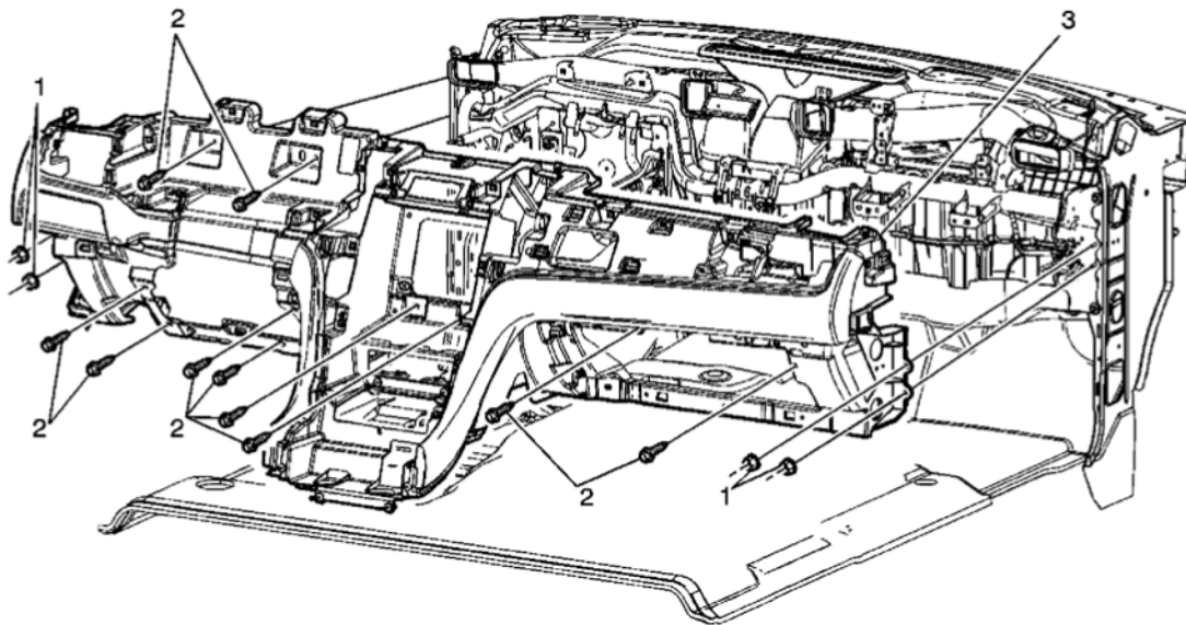
Fig. 32: View Of Instrument Panel Lower Trim Panel Assembly & Components Courtesy of GENERAL MOTORS CORP.
