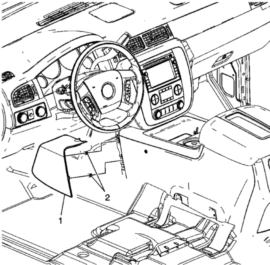
Fig. 44: View Of Console Side Trim Panel & Clips Courtesy of GENERAL MOTORS CORP.
