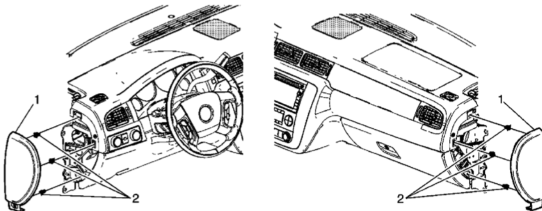
Fig. 18: View Of Instrument Panel Outer Trim Cover & Clips Courtesy of GENERAL MOTORS CORP.
