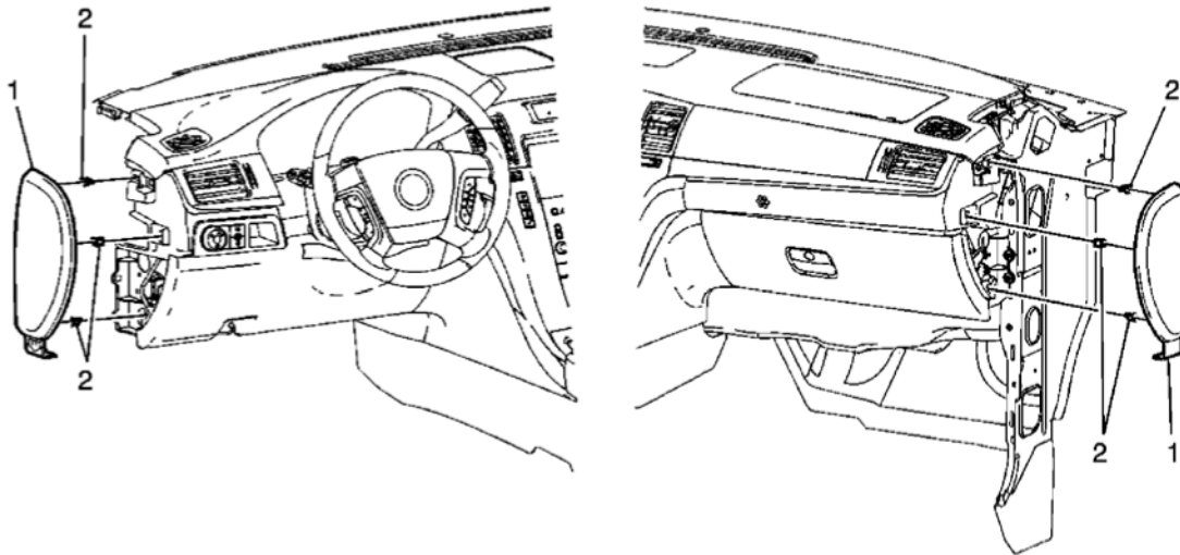
Fig. 17: View Of Instrument Panel Outer Trim Cover & Clips Courtesy of GENERAL MOTORS CORP.
