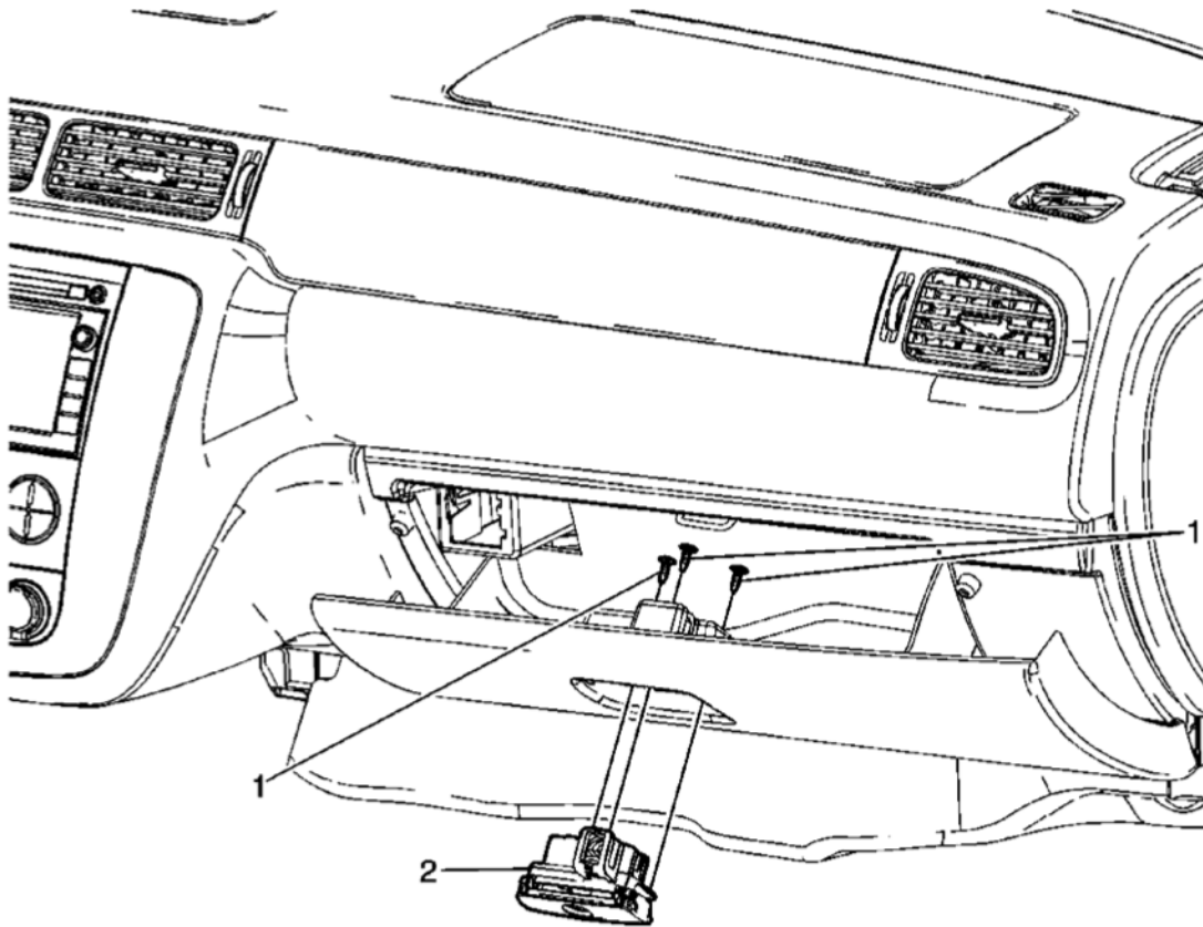
Fig. 27: View Of Instrument Panel Compartment Latch Assembly & Screws Courtesy of GENERAL MOTORS CORP.
