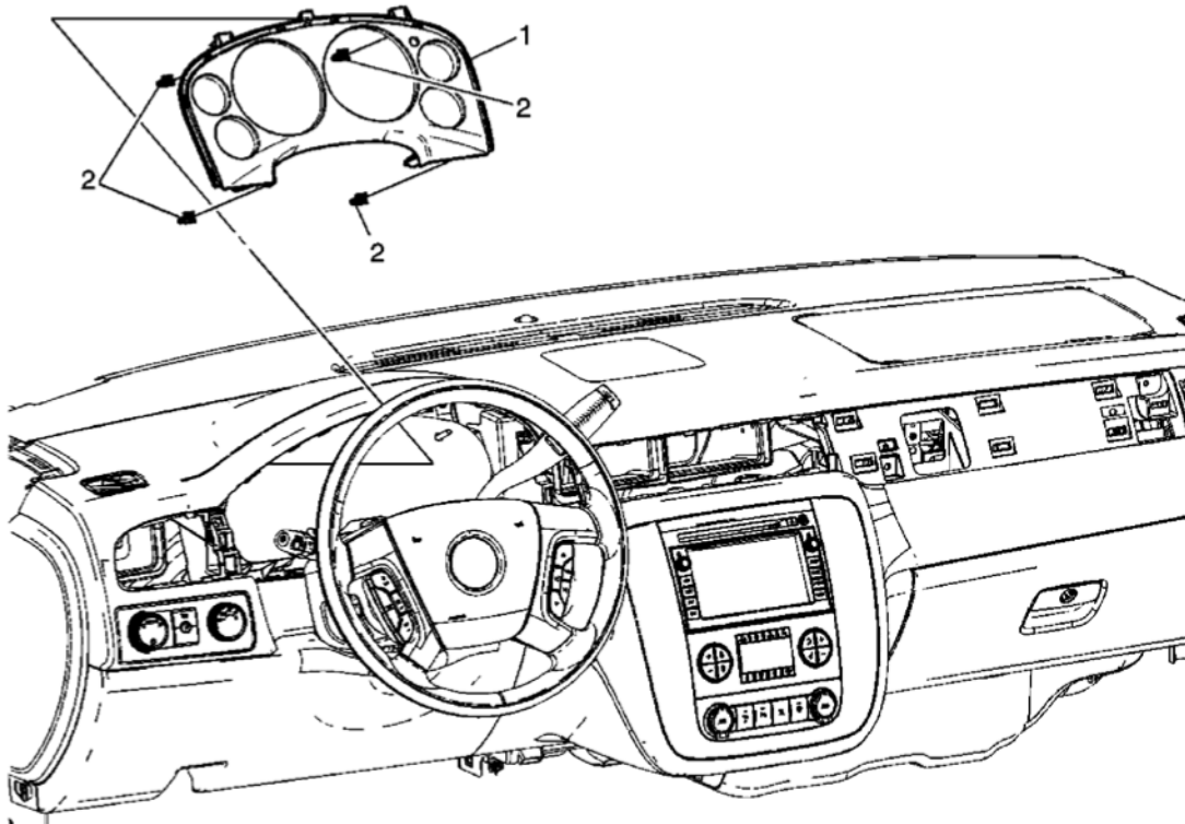
Fig. 16: View Of Instrument Panel Cluster Trim Plate Bezel & Clips Courtesy of GENERAL MOTORS CORP.
