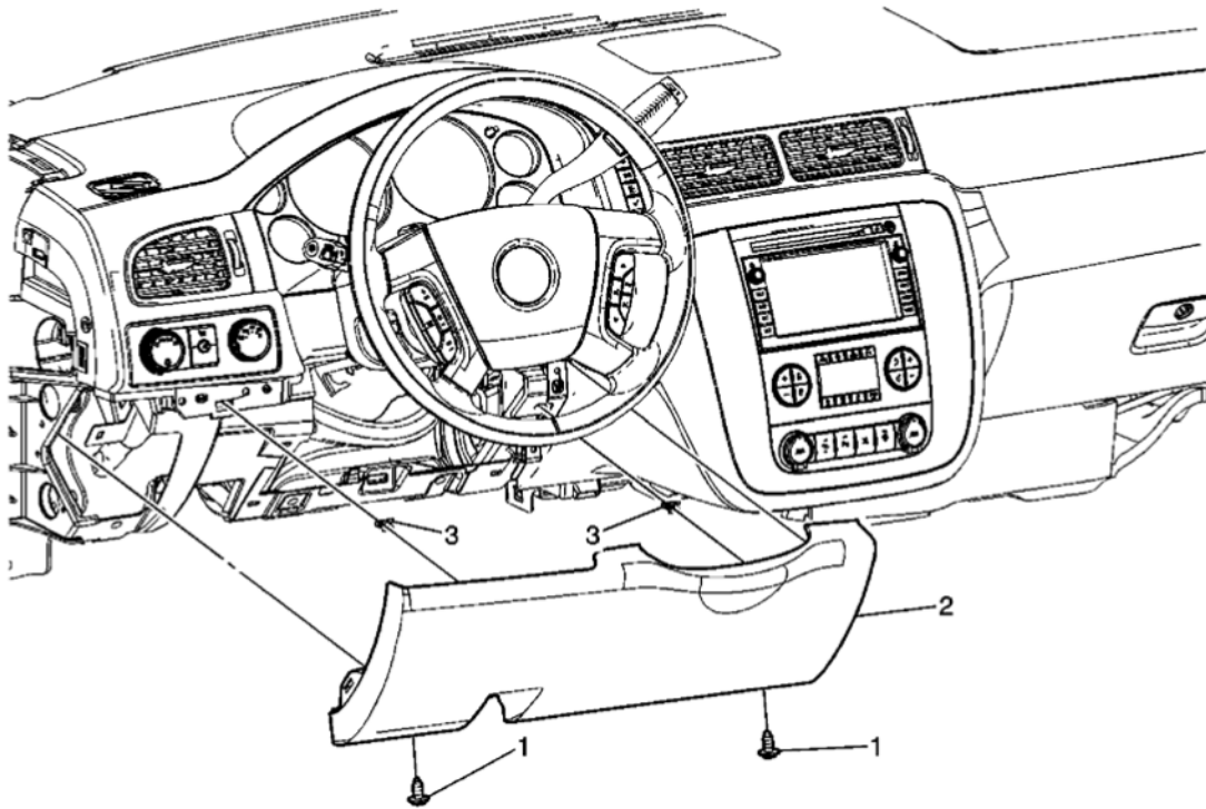
Fig. 5: View Of Knee Bolster Assembly & Components Courtesy of GENERAL MOTORS CORP.
