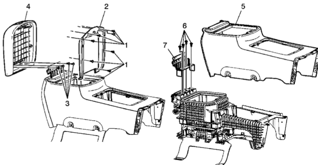
Fig. 50: View Of Front Floor Console Armrest Assembly & Components Courtesy of GENERAL MOTORS CORP.
