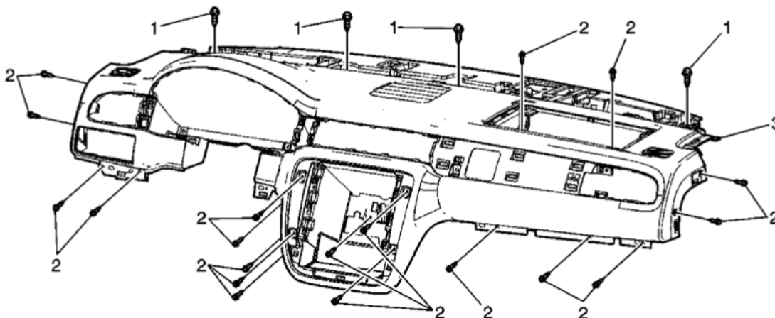
Fig. 12: View Of Instrument Panel Upper Trim Panel Assembly & Components Courtesy of GENERAL MOTORS CORP.
