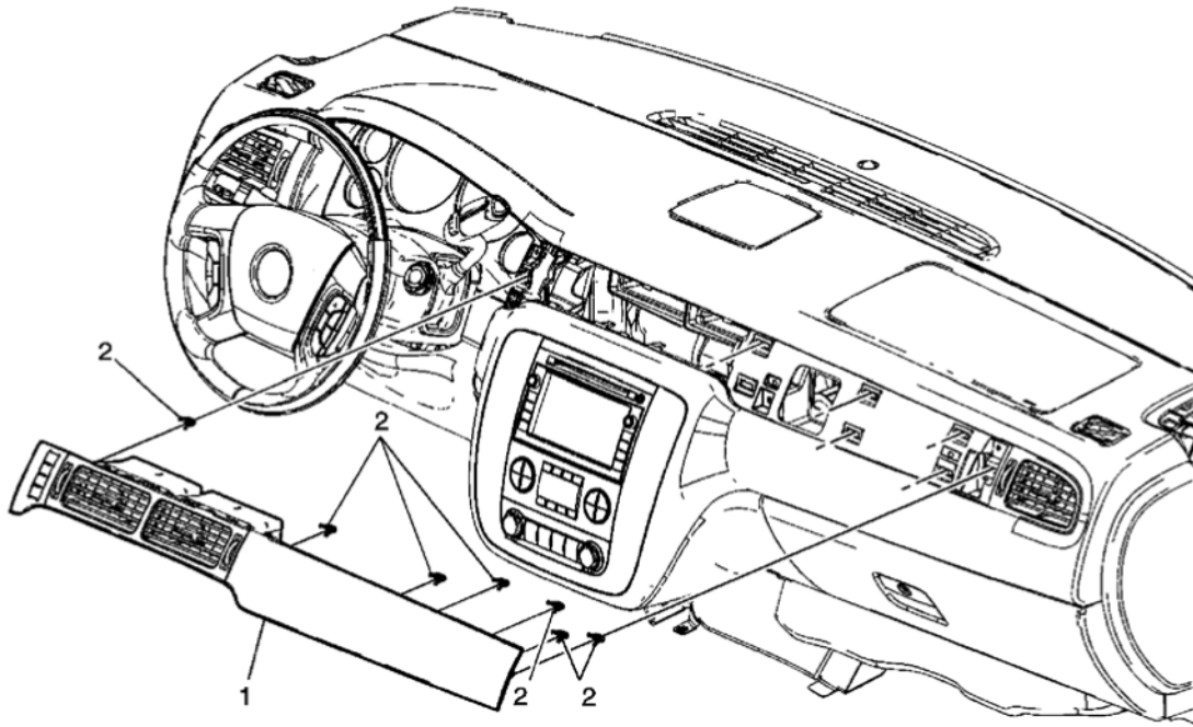
Fig. 10: Instrument Panel Center Trim Plate & Clips Courtesy of GENERAL MOTORS CORP.
