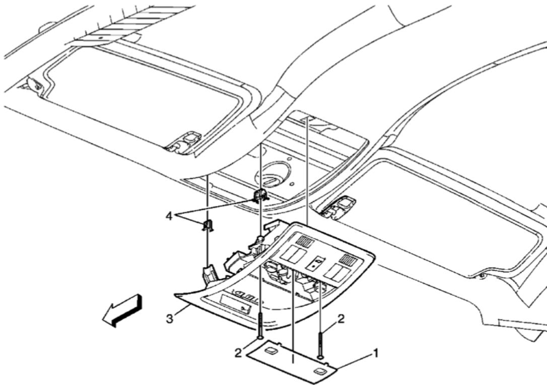
Fig. 54: View Of Roof Console Assembly & Components Courtesy of GENERAL MOTORS CORP.
