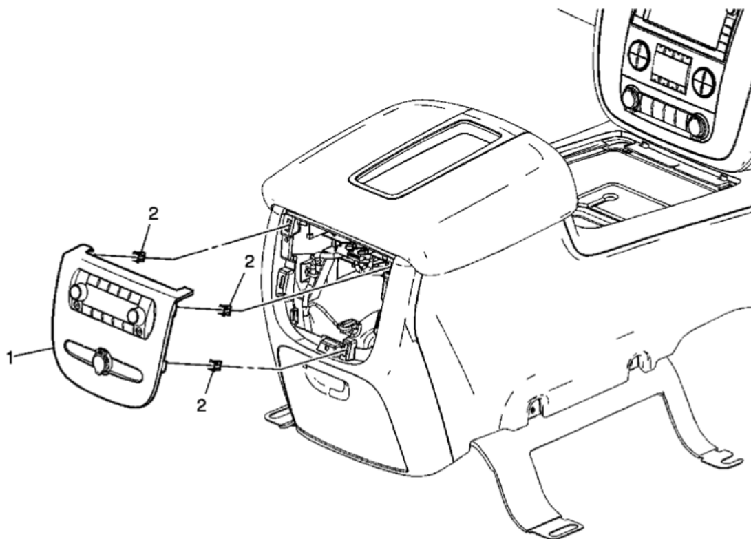
Fig. 39: View Of Front Floor Console Compartment Bezel Assembly & Clips Courtesy of GENERAL MOTORS CORP.
