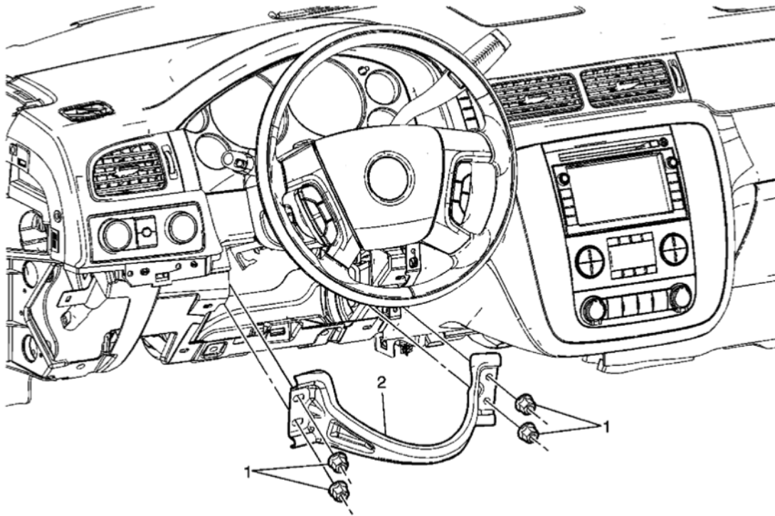
Fig. 6: View Of Knee Bolster Deflector & Nuts Courtesy of GENERAL MOTORS CORP.
