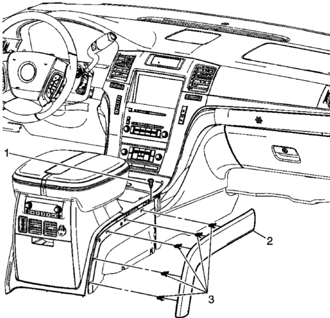
Fig. 41: View Of Front Floor Console Side Trim Panel & Components Courtesy of GENERAL MOTORS CORP.
