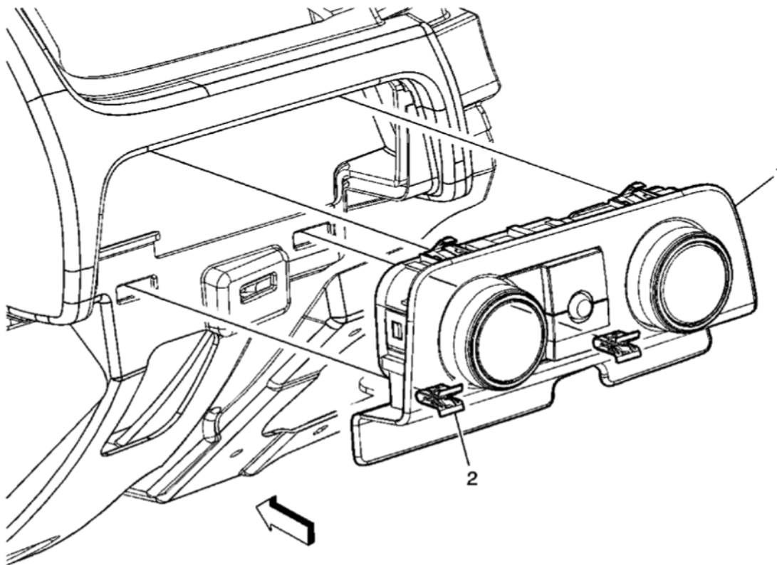
Fig. 13: View Of Headlamp Switch Trim Plate Assembly & Retainers Courtesy of GENERAL MOTORS CORP.
