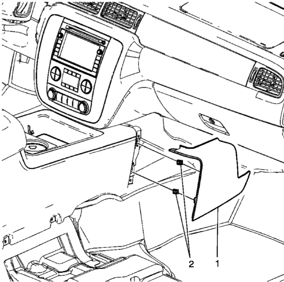
Fig. 42: View Of Console Side Trim Panel & Clips Courtesy of GENERAL MOTORS CORP.
