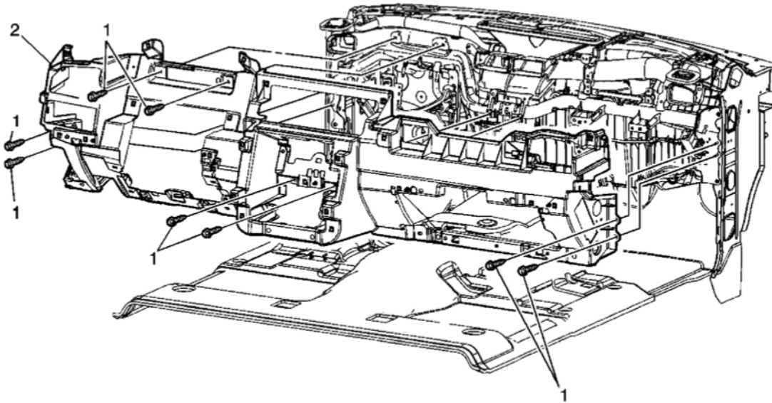
Fig. 35: View Of Instrument Panel Carrier Assembly & Bolts Courtesy of GENERAL MOTORS CORP.
