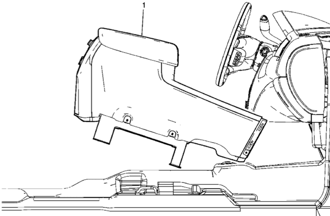
Fig. 49: View Of Front Floor Console Assembly Courtesy of GENERAL MOTORS CORP.
