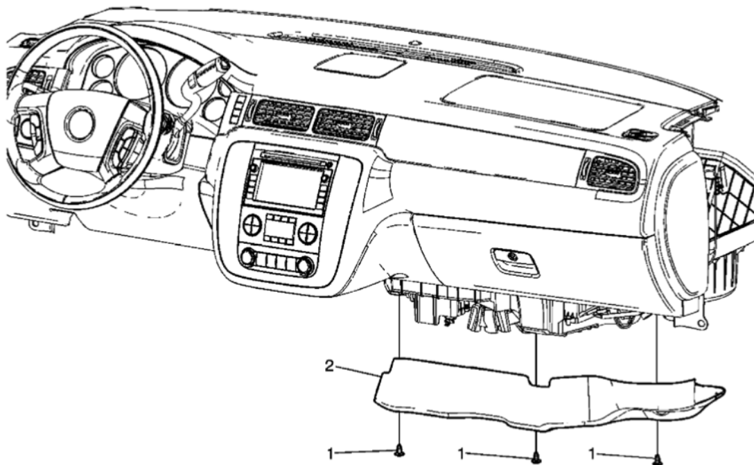
Fig. 2: View Of Instrument Panel Lower Trim Panel Insulator & Screws Courtesy of GENERAL MOTORS CORP.
