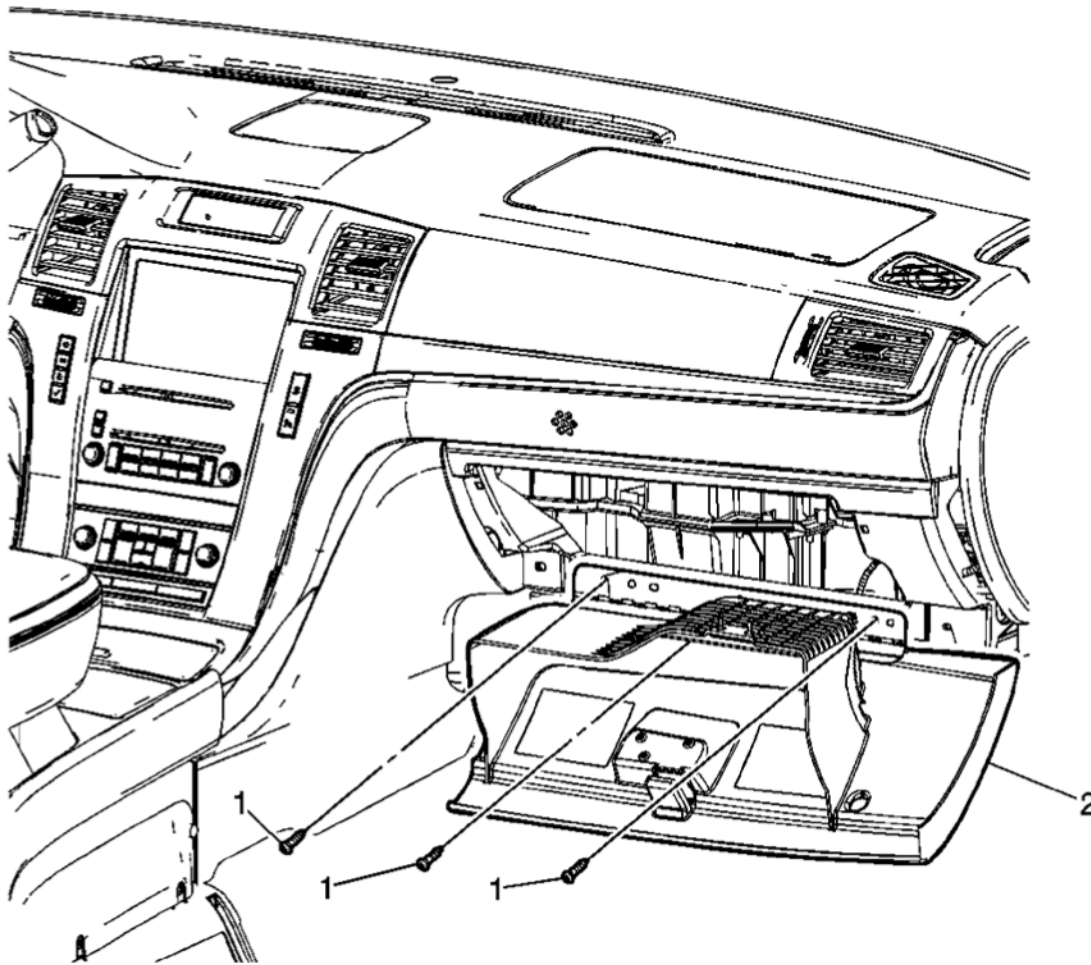
Fig. 21: View Of Instrument Panel Compartment Assembly & Screws Courtesy of GENERAL MOTORS CORP.
