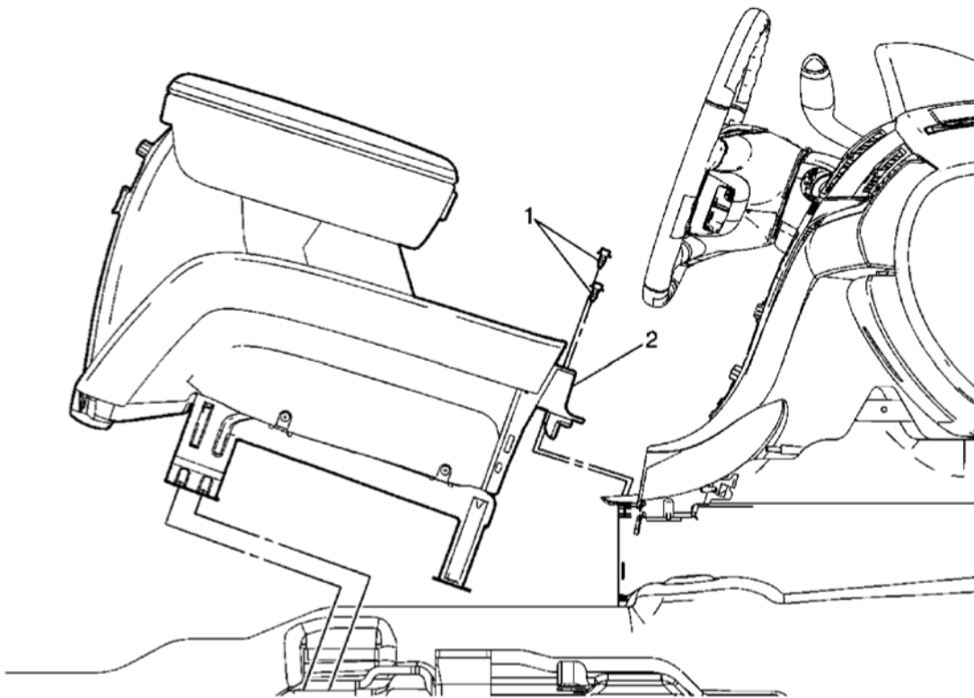
Fig. 48: View Of Front Floor Console Assembly & Bolts Courtesy of GENERAL MOTORS CORP.
