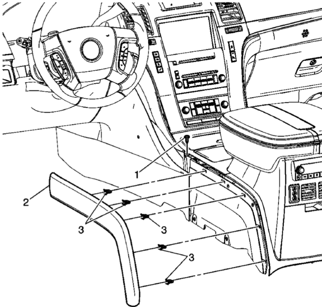
Fig. 43: View Of Console Side Trim Panel & Components Courtesy of GENERAL MOTORS CORP.
