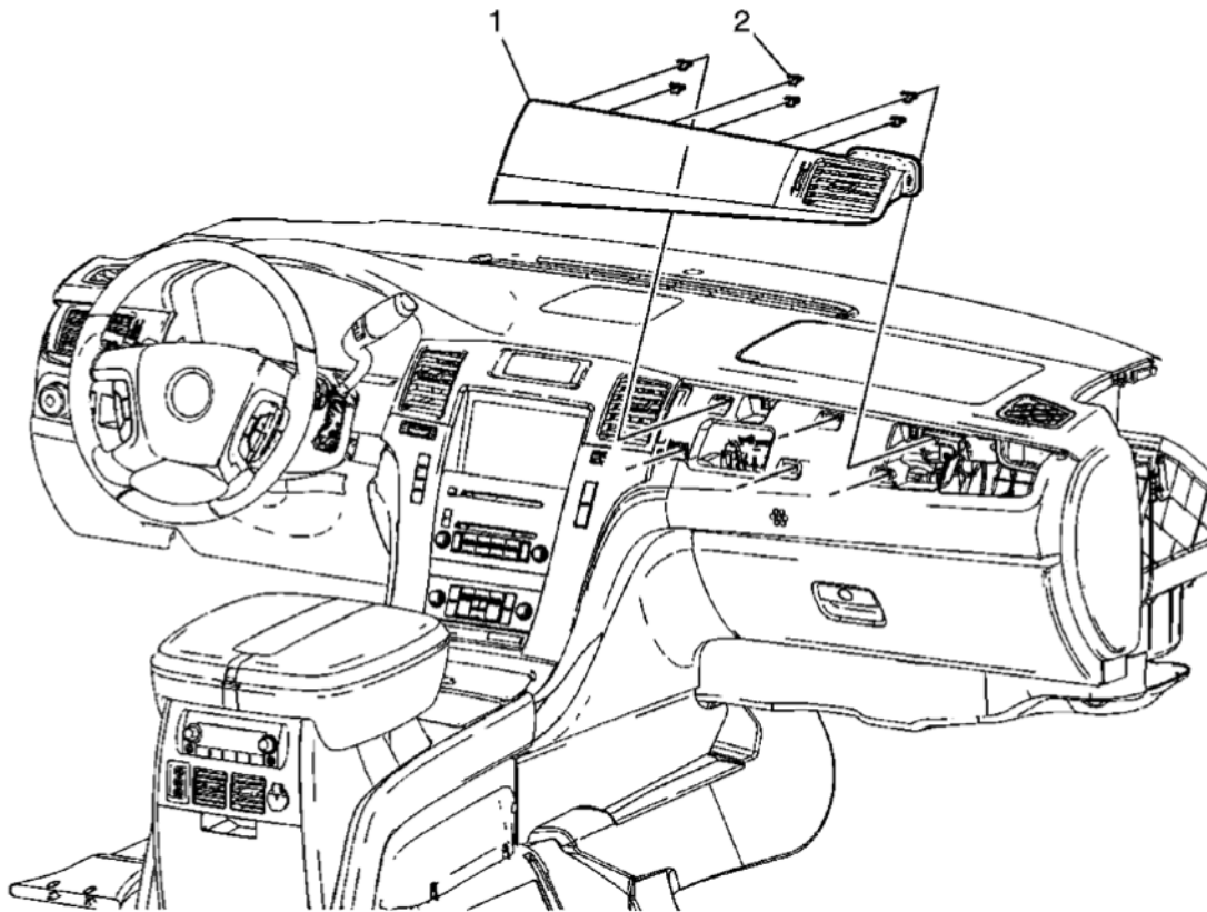
Fig. 9: Instrument Panel Center Trim Plate & Clips Courtesy of GENERAL MOTORS CORP.
