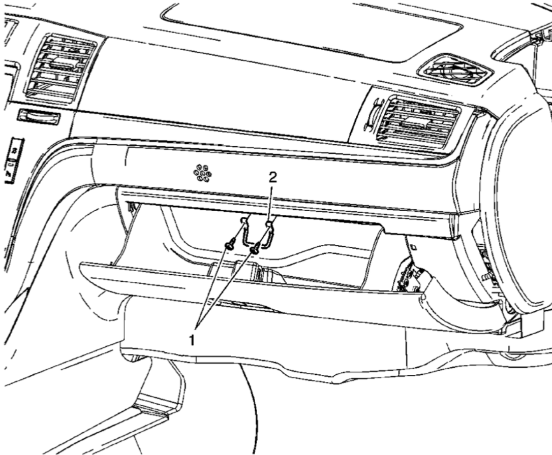
Fig. 19: View Of Instrument Panel Compartment Striker & Screws Courtesy of GENERAL MOTORS CORP.
