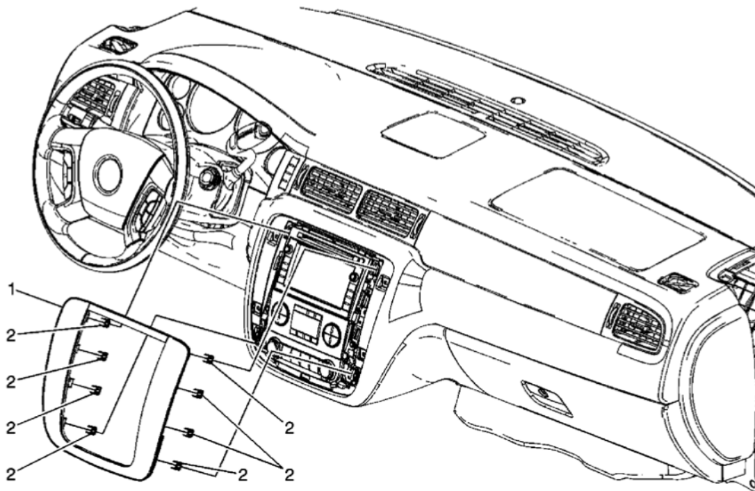
Fig. 8: View Of Instrument Panel Accessory Trim Panel & Clips Courtesy of GENERAL MOTORS CORP.
