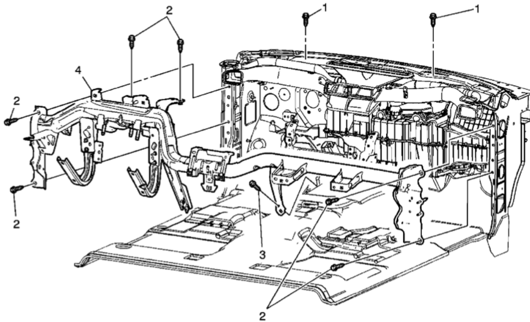
Fig. 37: View Of Instrument Panel Carrier Support Assembly & Bolts Courtesy of GENERAL MOTORS CORP.
