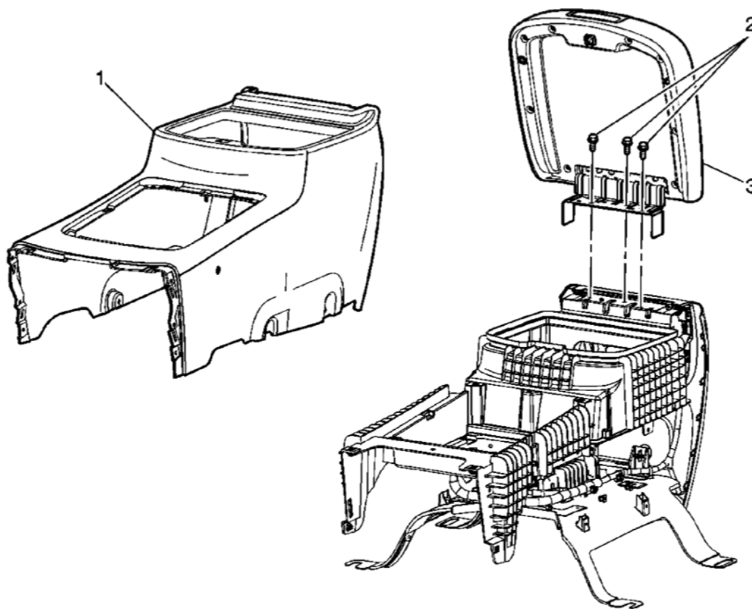
Fig. 53: View Of Front Floor Console Lid Assembly & Components Courtesy of GENERAL MOTORS CORP.
