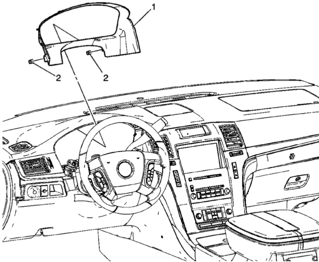
Fig. 15: View Of Instrument Panel Cluster Trim Plate Bezel & Clips Courtesy of GENERAL MOTORS CORP.
