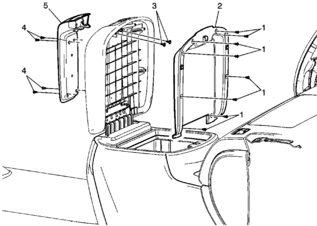
Fig. 40: View Of Front Floor Console Cover Latch Assembly & Components Courtesy of GENERAL MOTORS CORP.
