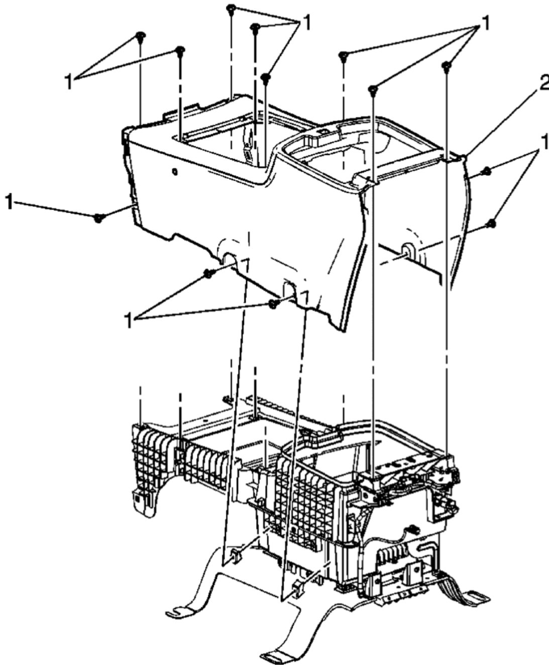
Fig. 47: View Of Front Floor Console Compartment Assembly & Screws Courtesy of GENERAL MOTORS CORP.
