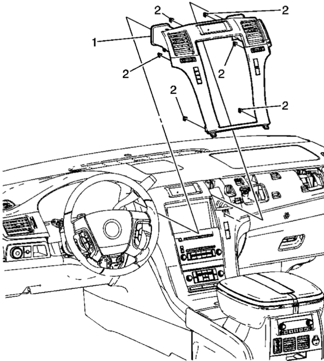
Fig. 7: View Of Instrument Panel Accessory Trim Panel & Clips Courtesy of GENERAL MOTORS CORP.
