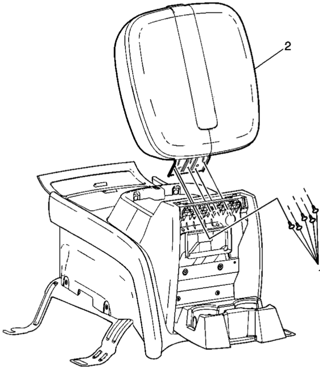
Fig. 52: View Of Front Top Storage Compartment Lid Assembly & Screws Courtesy of GENERAL MOTORS CORP.
