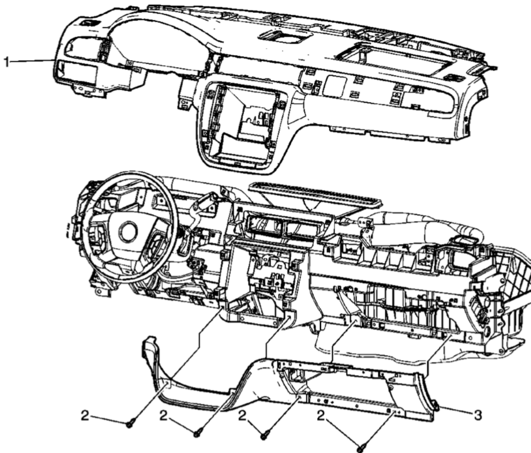
Fig. 23: View Of Instrument Panel Compartment Assembly & Components Courtesy of GENERAL MOTORS CORP.
