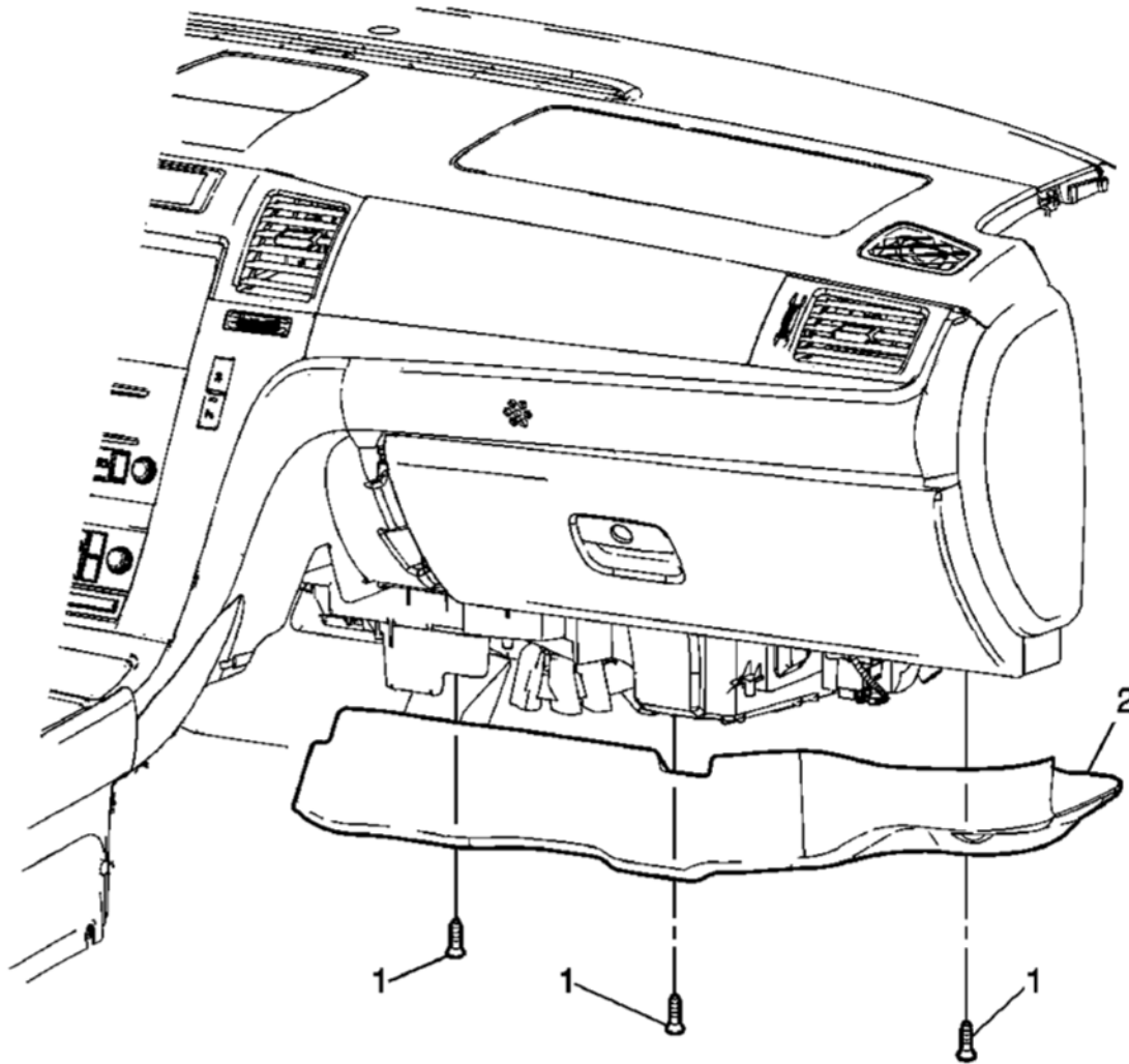
Fig. 1: View Of Instrument Panel Lower Trim Panel Insulator & Screws Courtesy of GENERAL MOTORS CORP.
