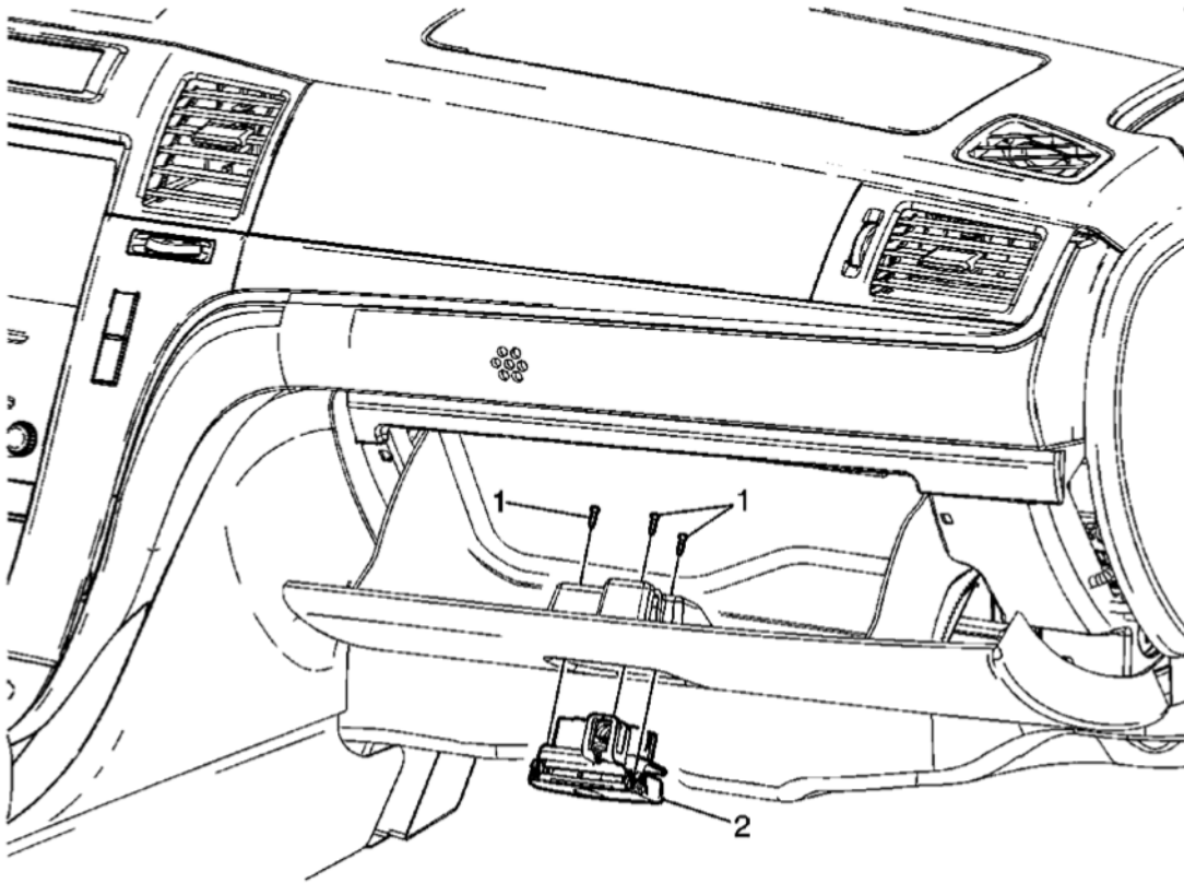
Fig. 26: View Of Instrument Panel Compartment Latch Assembly & Screws Courtesy of GENERAL MOTORS CORP.
