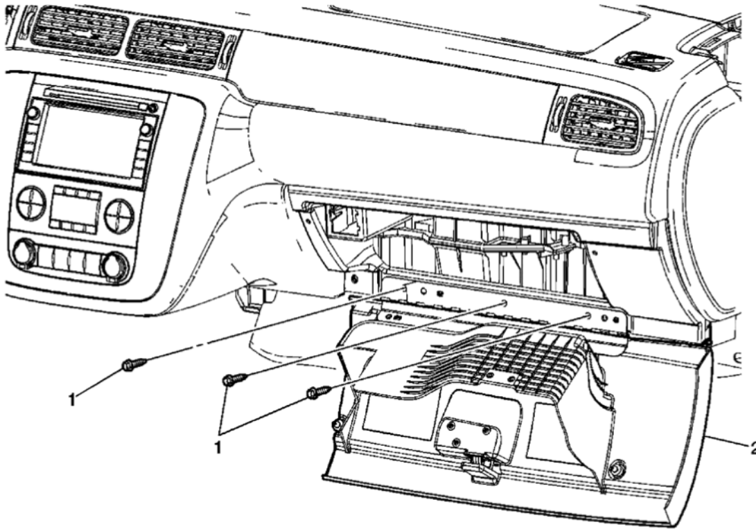
Fig. 22: View Of Instrument Panel Compartment Door Assembly & Screws Courtesy of GENERAL MOTORS CORP.
