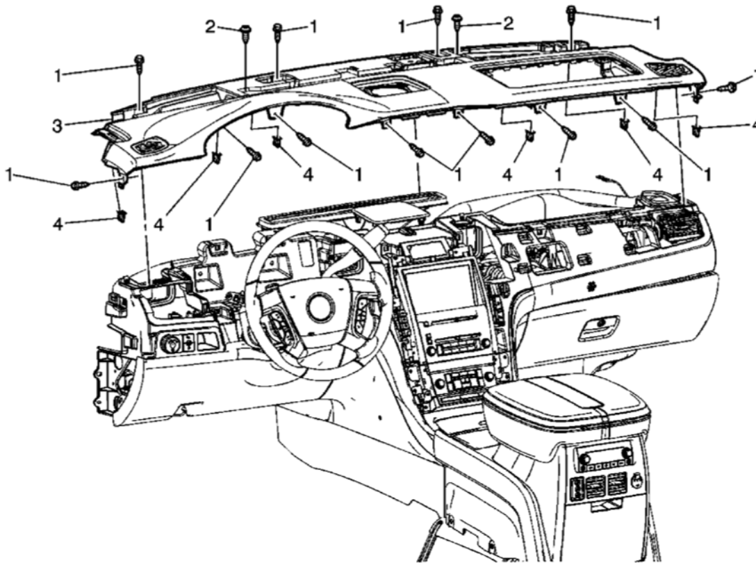
Fig. 11: View Of Instrument Panel Upper Trim Panel Assembly & Components Courtesy of GENERAL MOTORS CORP.
