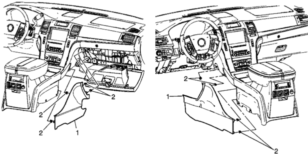
Fig. 3: View Of Instrument Panel Lower Center Trim & Clips Courtesy of GENERAL MOTORS CORP.
