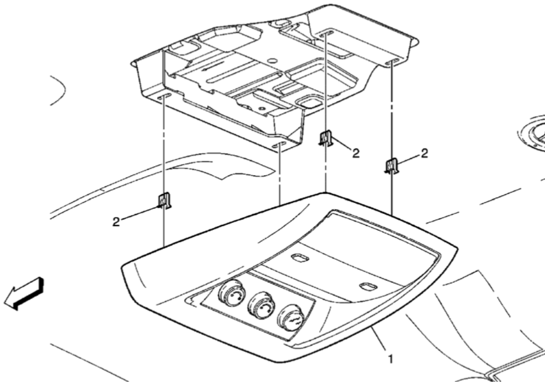
Fig. 55: View Of Rear Overhead Console Assembly & Retainers Courtesy of GENERAL MOTORS CORP.
