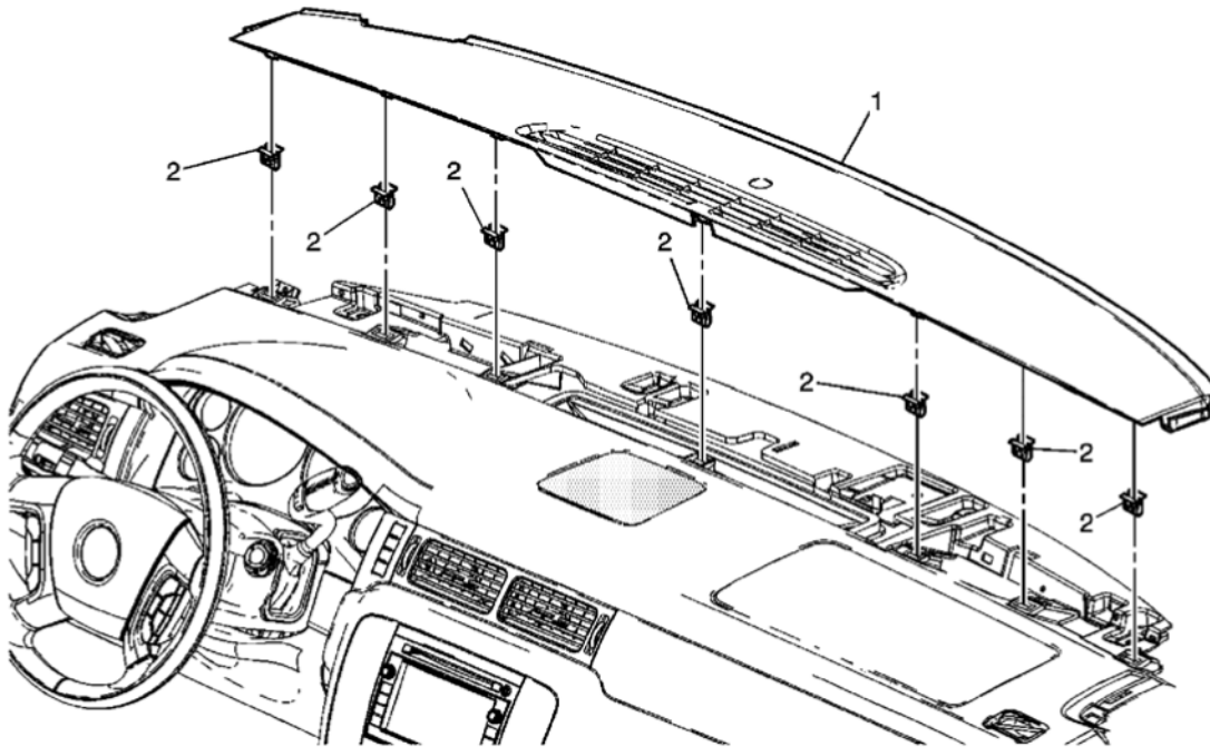
Fig. 34: View Of Instrument Panel Upper Trim Panel with Windshield Defroster Nozzle & Clips Courtesy of GENERAL MOTORS CORP.
