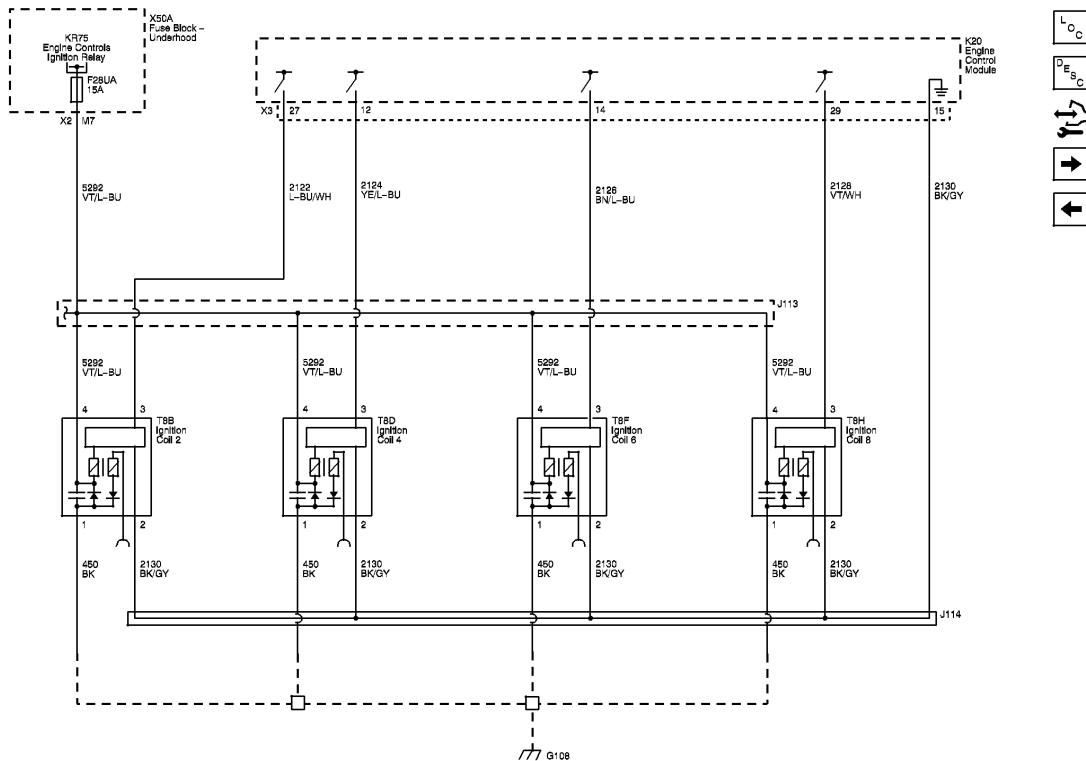
Fig. 8: Ignition Controls - Ignition Coils 2, 4, 6, and 8 Wiring Schematic Courtesy of GENERAL MOTORS COMPANY
