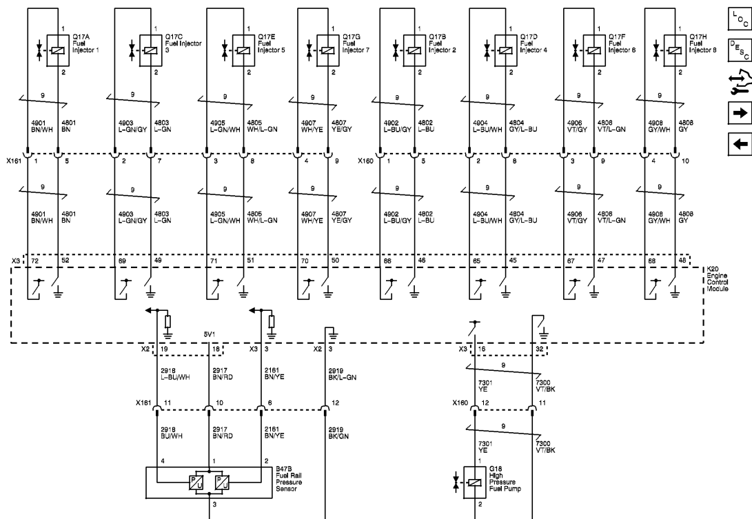
Fig. 11: Fuel Controls - Fuel Injectors, FRP Sensor, High Pressure Fuel Pump Wiring Schematic
