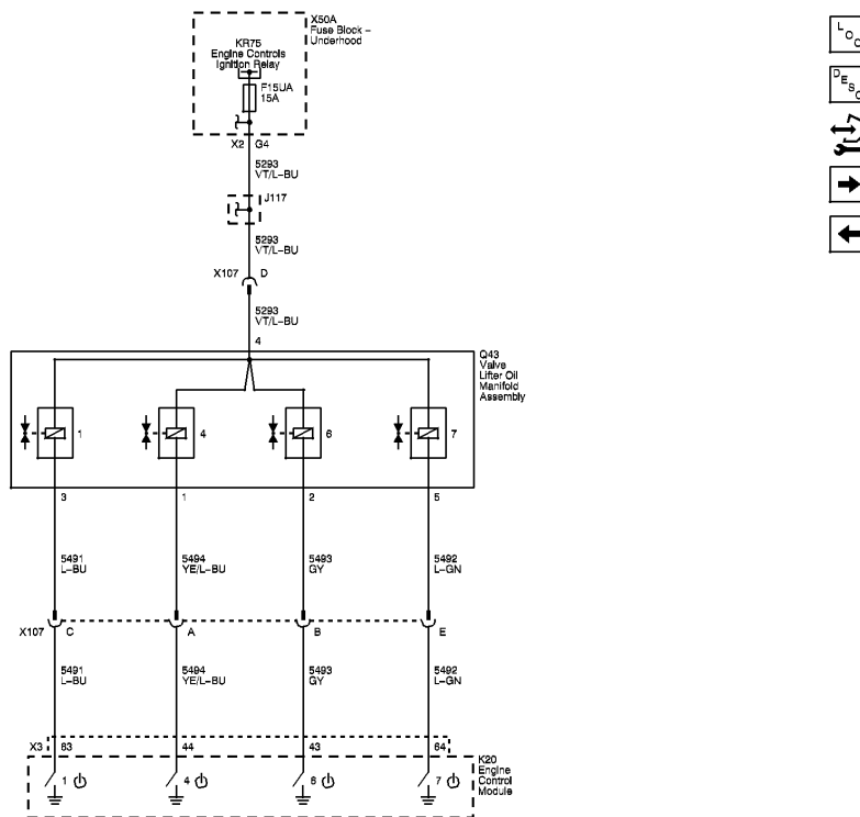
Fig. 10: Device Controls - Displacement on Demand (LT1) Wiring Schematic Courtesy of GENERAL MOTORS COMPANY
