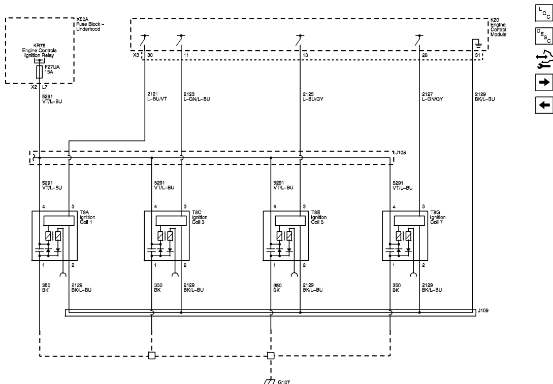
Fig. 7: Ignition Controls - Ignition Coils 1, 3, 5, and 7 Wiring Schematic Courtesy of GENERAL MOTORS COMPANY
