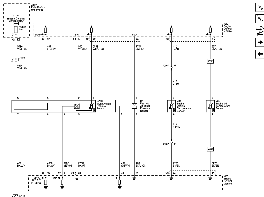
Fig. 4: Engine Data Sensors - Pressure, and Temperature Wiring Schematic Courtesy of GENERAL MOTORS COMPANY
