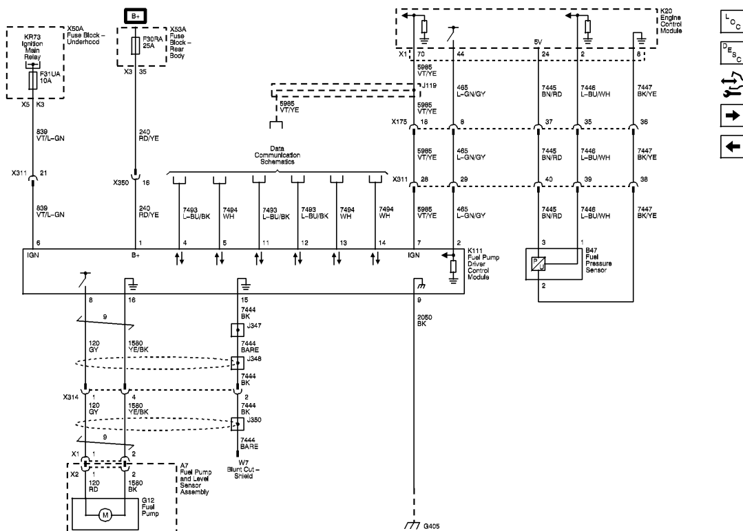
Fig. 12: Fuel Controls - Fuel Pump Controls Wiring Schematic Courtesy of GENERAL MOTORS COMPANY
