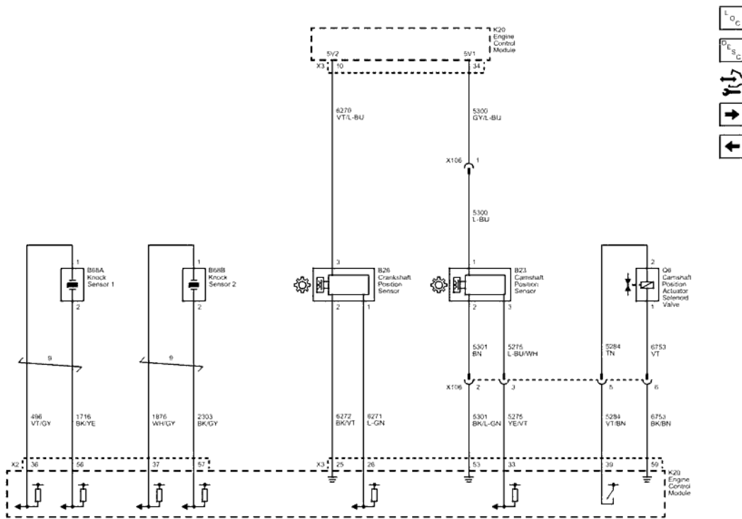
Fig. 9: Ignition Controls - Camshaft, Crankshaft and Knock Sensors, Camshaft Actuator Wiring Schematic
