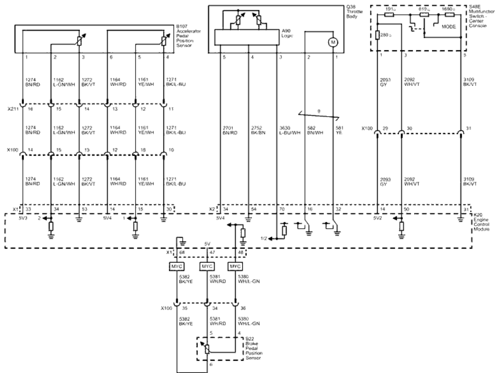
Fig. 5: Engine Data Sensors - Throttle Controls Wiring Schematic Courtesy of GENERAL MOTORS COMPANY
