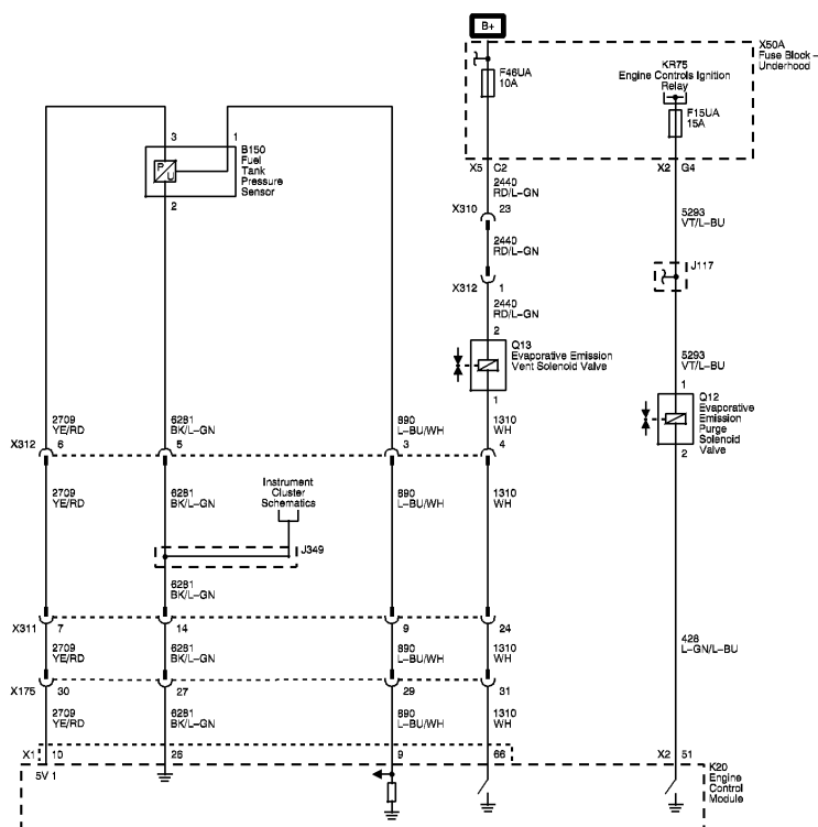
Fig. 13: Fuel Controls - Evaporative Emission Controls Wiring Schematic Courtesy of GENERAL MOTORS COMPANY
