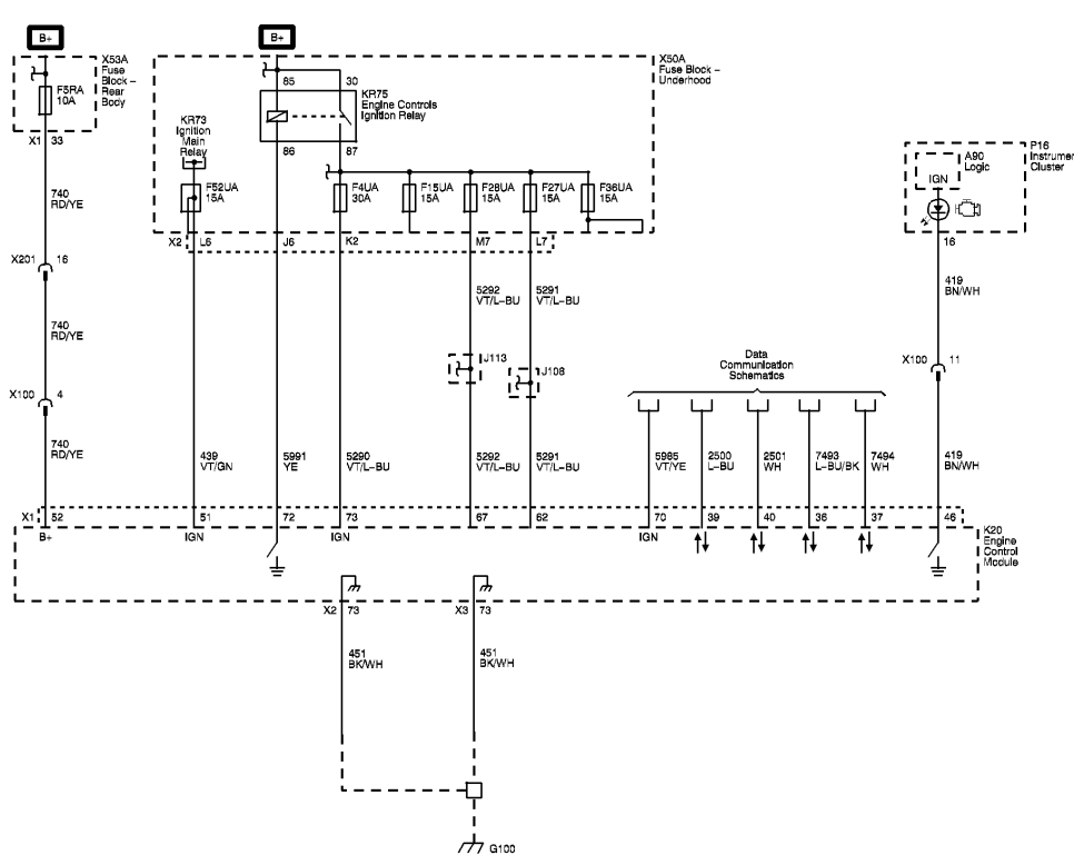
Fig. 1: Module Power, Ground, Serial Data, and MIL Wiring Schematic Courtesy of GENERAL MOTORS COMPANY
