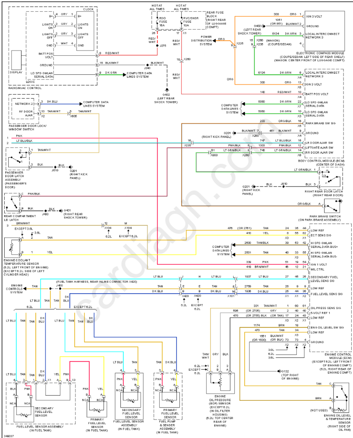
Fig. 55: Instrument Cluster Circuit (2 of 2)
