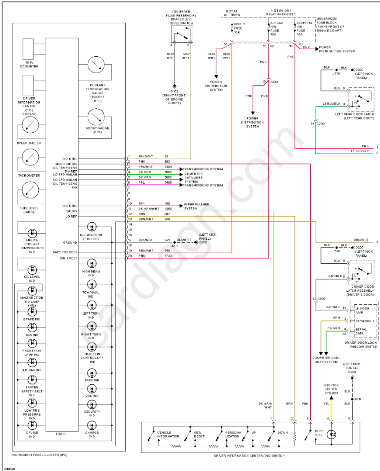
Fig. 54: Instrument Cluster Circuit (1 of 2)
