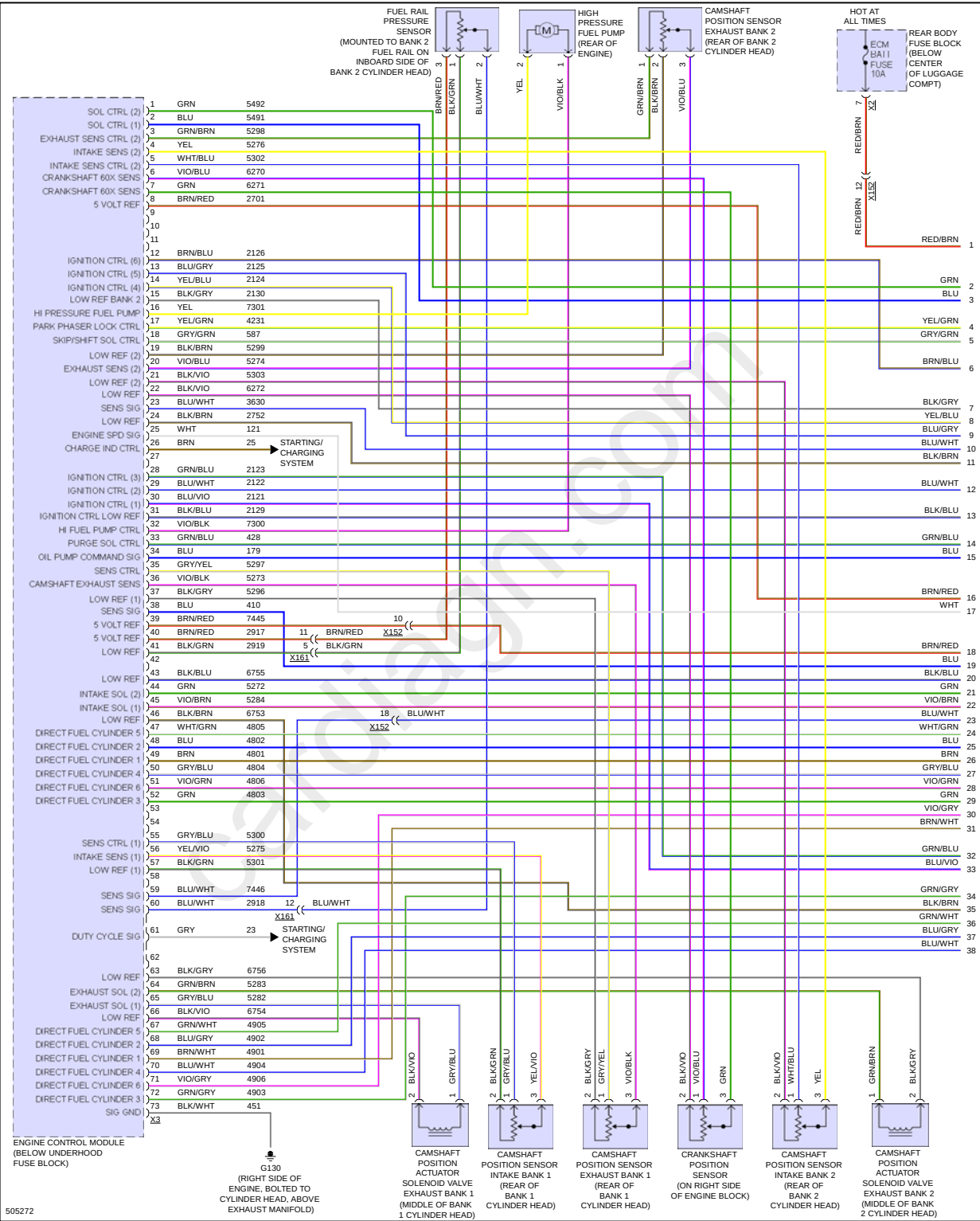
Fig 1: 3.6L VIN S, Engine Performance Circuit (1 of 8)
