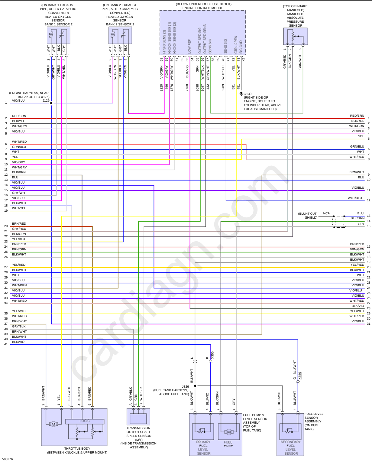
Fig 5: 3.6L VIN S, Engine Performance Circuit (5 of 8)
