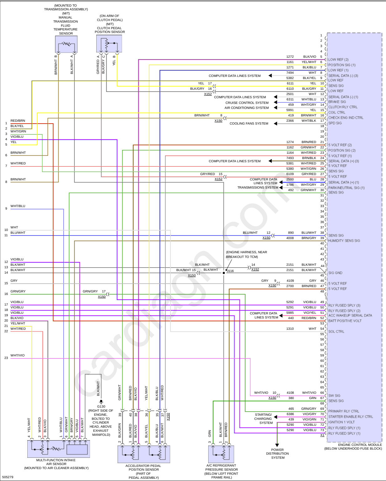
Fig 8: 3.6L VIN S, Engine Performance Circuit (8 of 8)
