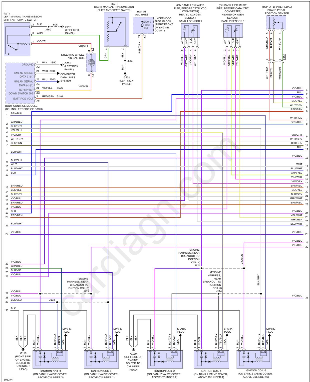
Fig 3: 3.6L VIN S, Engine Performance Circuit (3 of 8)
