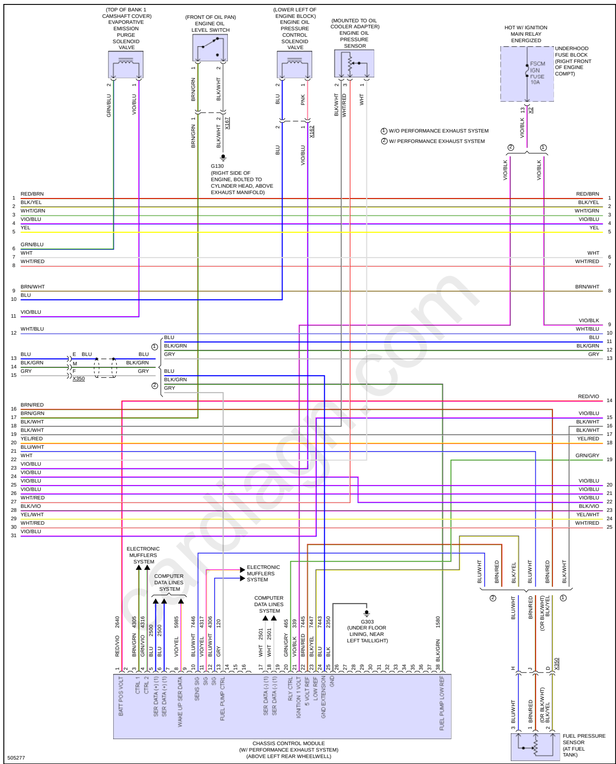
Fig 6: 3.6L VIN S, Engine Performance Circuit (6 of 8)
