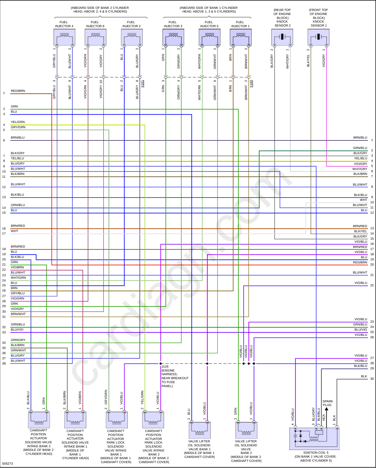
Fig 2: 3.6L VIN S, Engine Performance Circuit (2 of 8)
