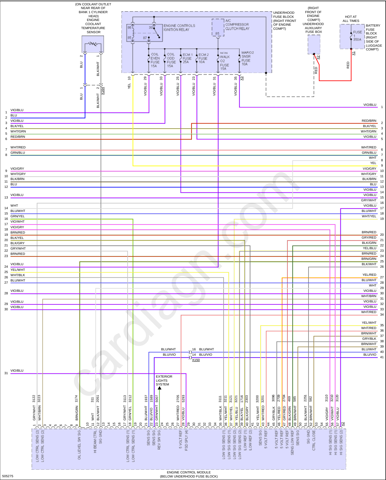
Fig 4: 3.6L VIN S, Engine Performance Circuit (4 of 8)
