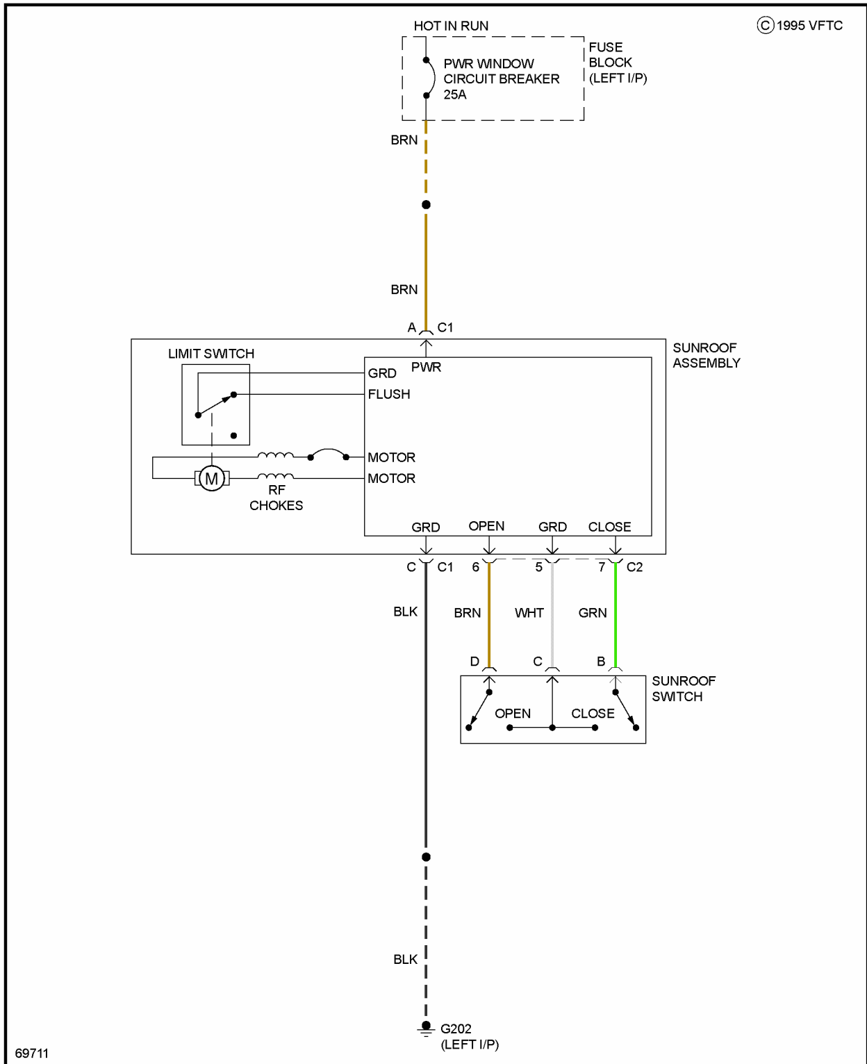
Fig. 35: Sunroof Circuit
