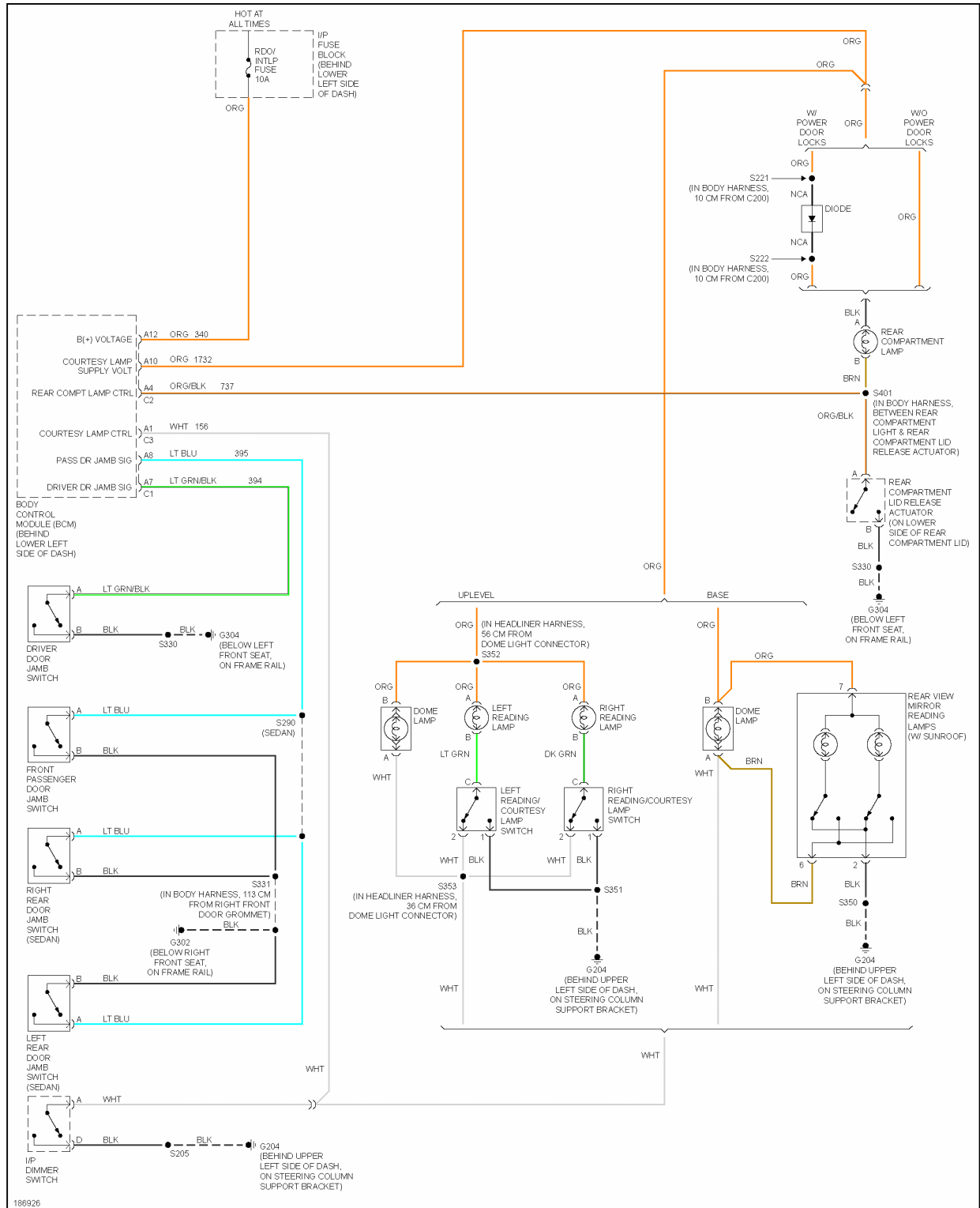
Fig. 20: Courtesy Lamps Circuit
