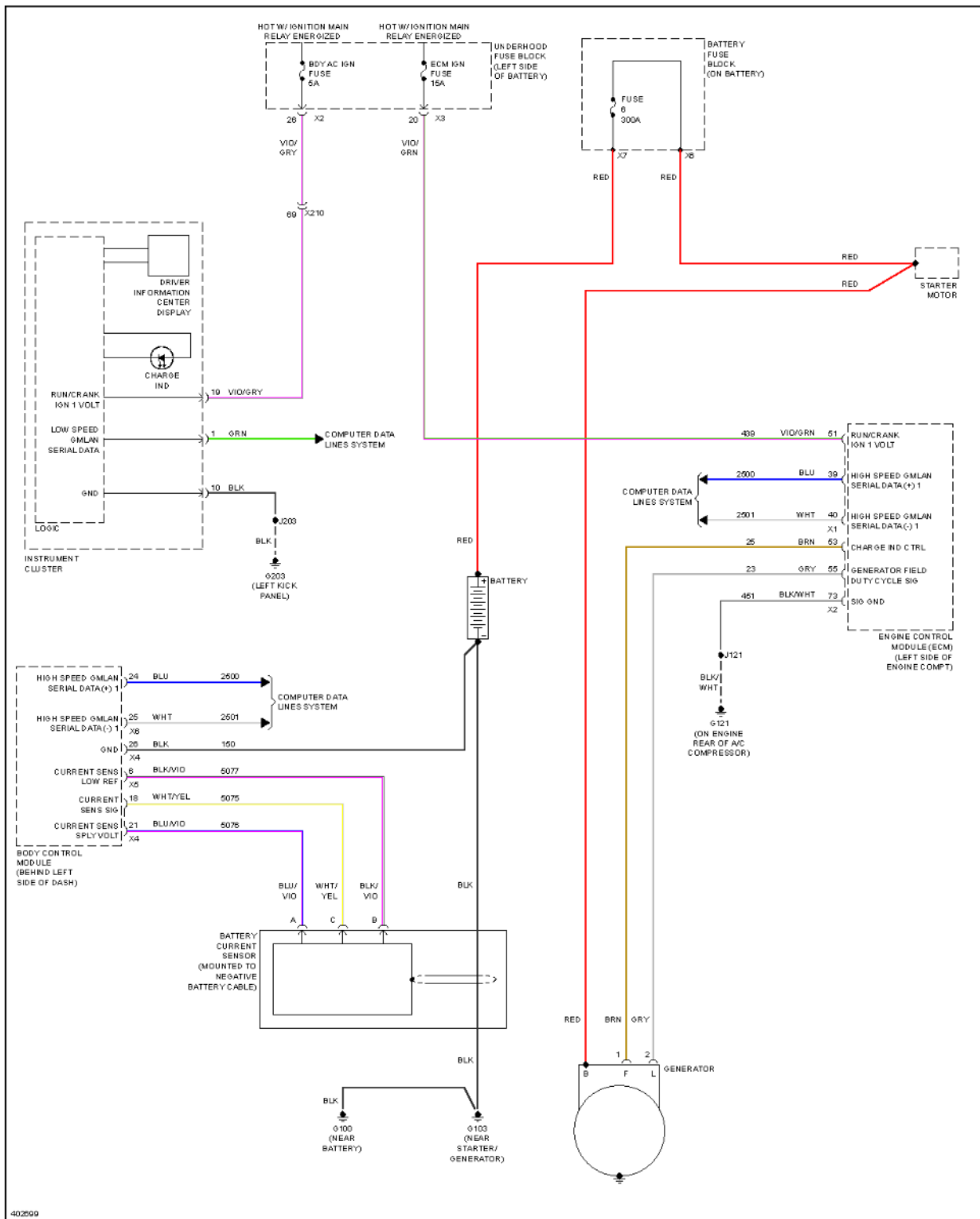
Fig. 124: Charging Circuit
