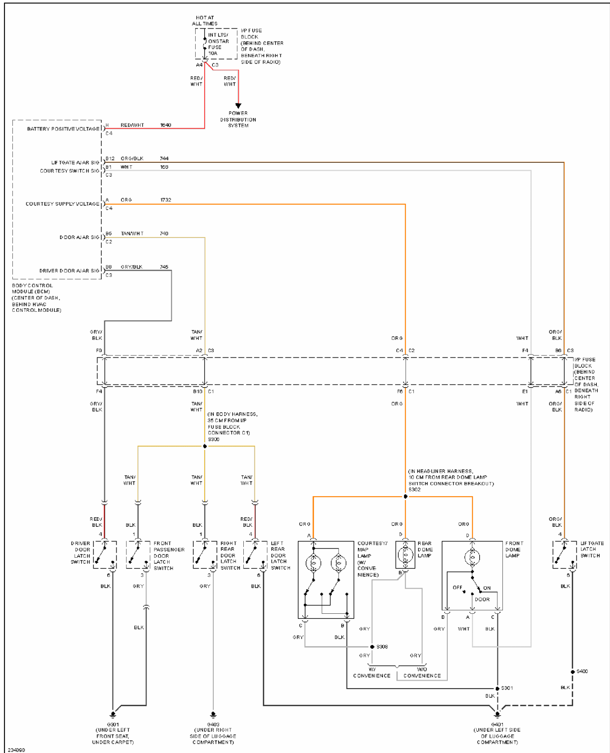
Fig. 25: Courtesy Lamps Circuit
