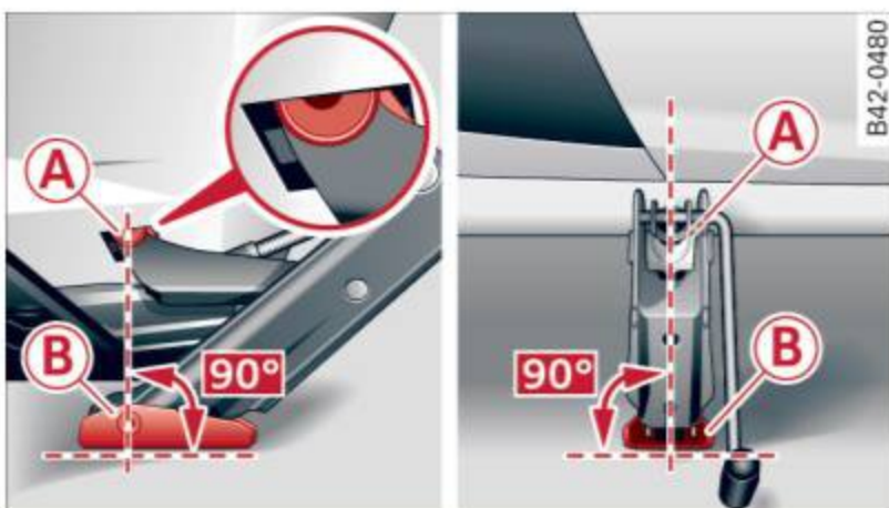
Fig. 158 Sill: positioning the vehicle jack
