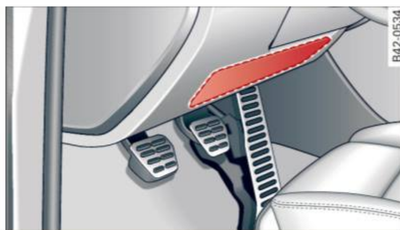
Fig. 124 Driver's airbag
