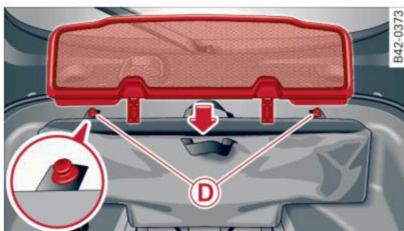
Fig. 42 Luggage compartment: storing the wind deflector
