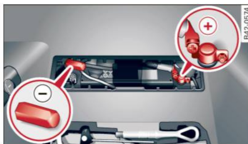
Fig. 146 Luggage compartment: connectors for a charger and jump start cables
