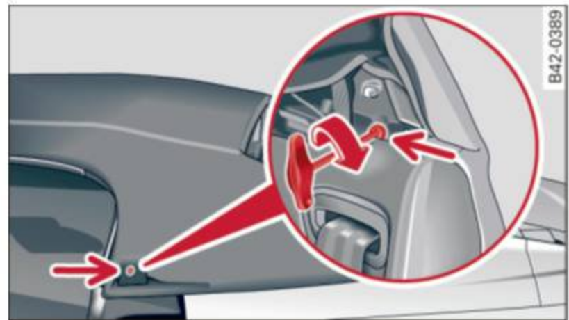
Fig. 58 Interior: tightening the bolt
