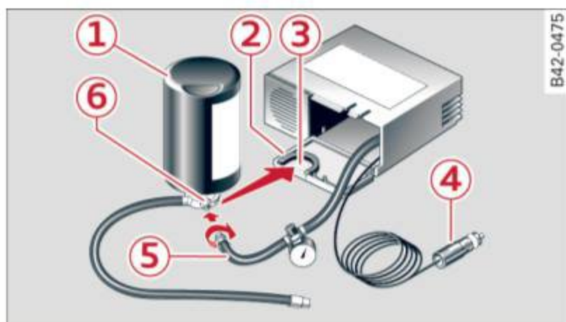
Fig. 154 Parts of the Tire Mobility System
