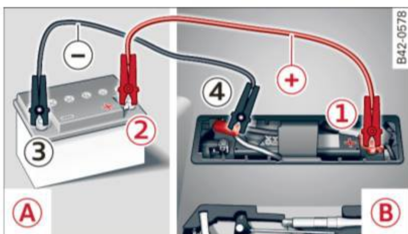
Fig. 161 Jump start using the battery in another vehicle: A - Female socket, B - Discharge
