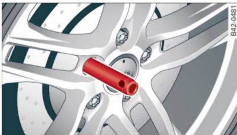
Fig. 159 Wheel change: alignment pin inside the top hole
