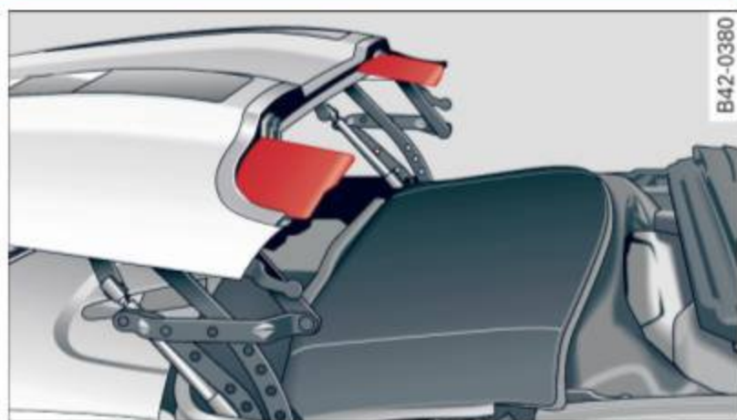
Fig. 49 Convertible top: covers marked
