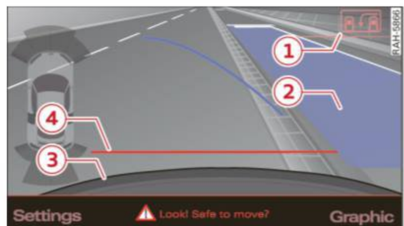
Fig. 98 Navigation system display: Blue surface aligned with parking spot
