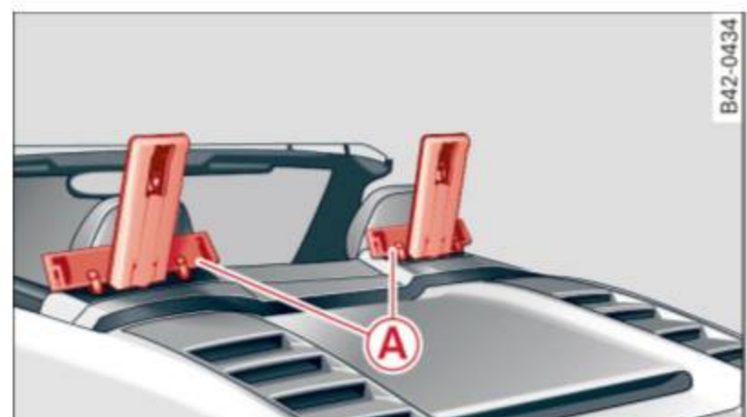
Fig. 109 Deployed rollbar with convertible top frame facing upward
