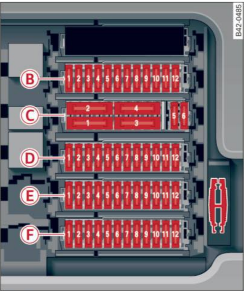
Fig. 164 Passenger footwell: Fuse assignment
