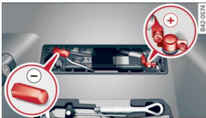
Fig. 160 Luggage compartment: connectors for a charger and jump start cables
