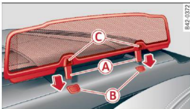
Fig. 41 Installing the wind deflector
