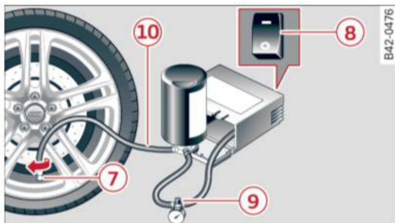
Fig. 155 Connector for the Tire Mobility System
