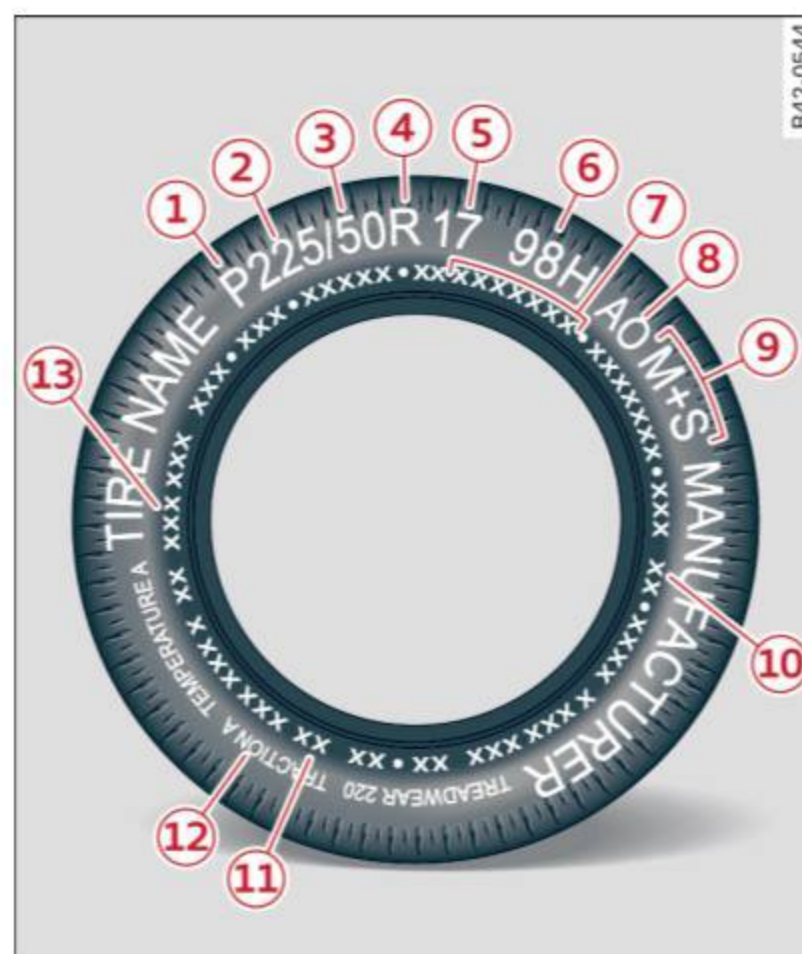
Fig. 151 Tire specification codes on the sidewall of a tire
