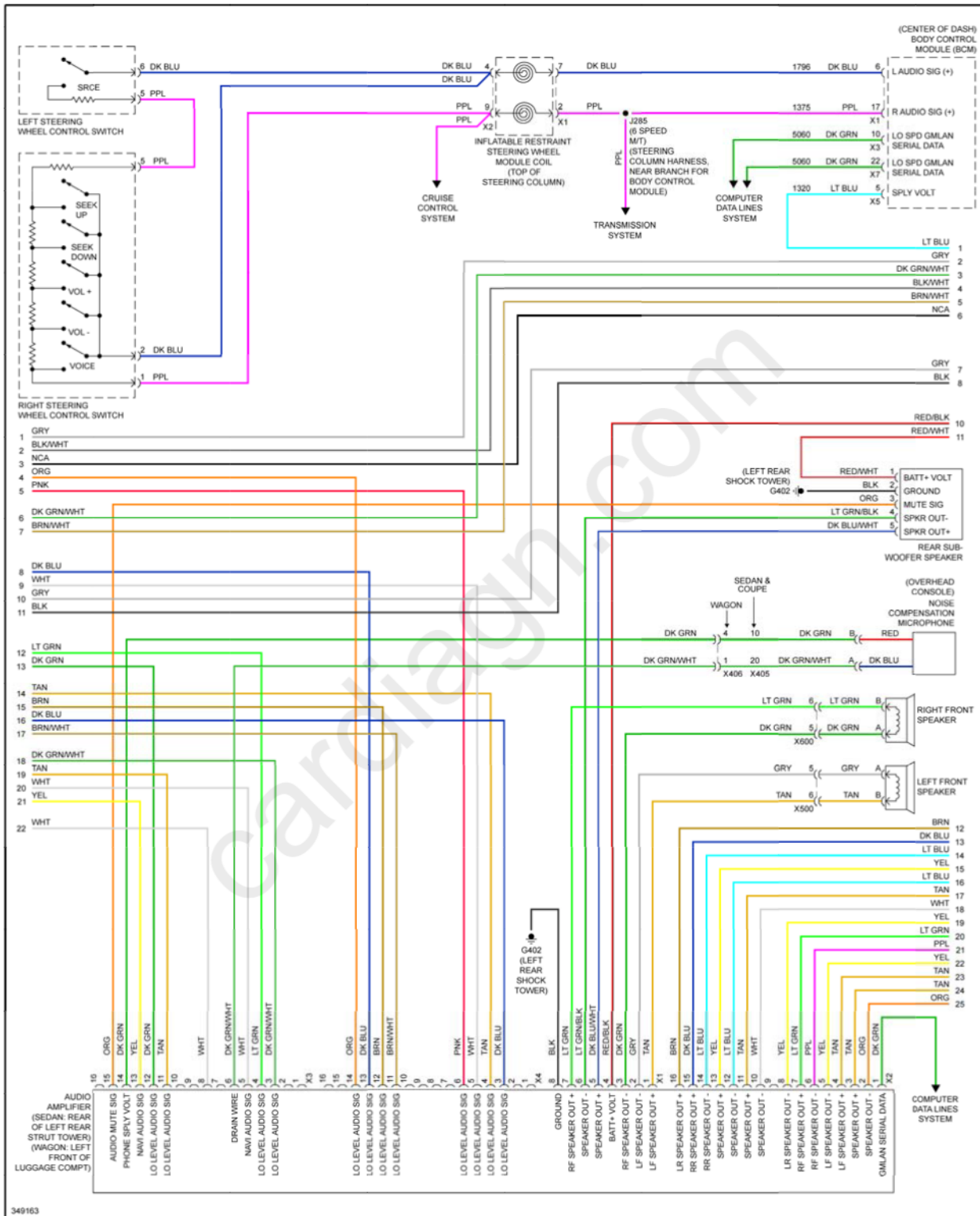
Fig. 101: Radio Circuit, W/ Surround Amplifier (3 of 4)
