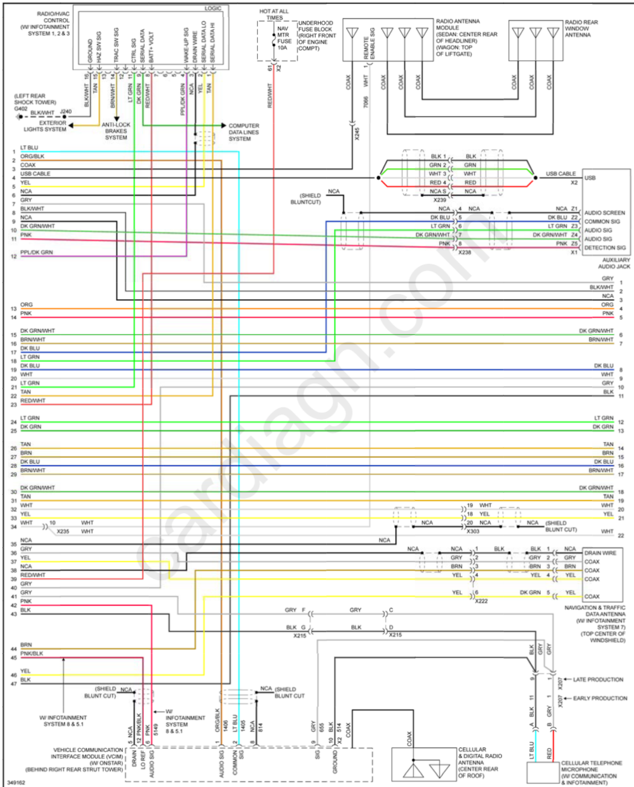
Fig. 100: Radio Circuit, W/ Surround Amplifier (2 of 4)
