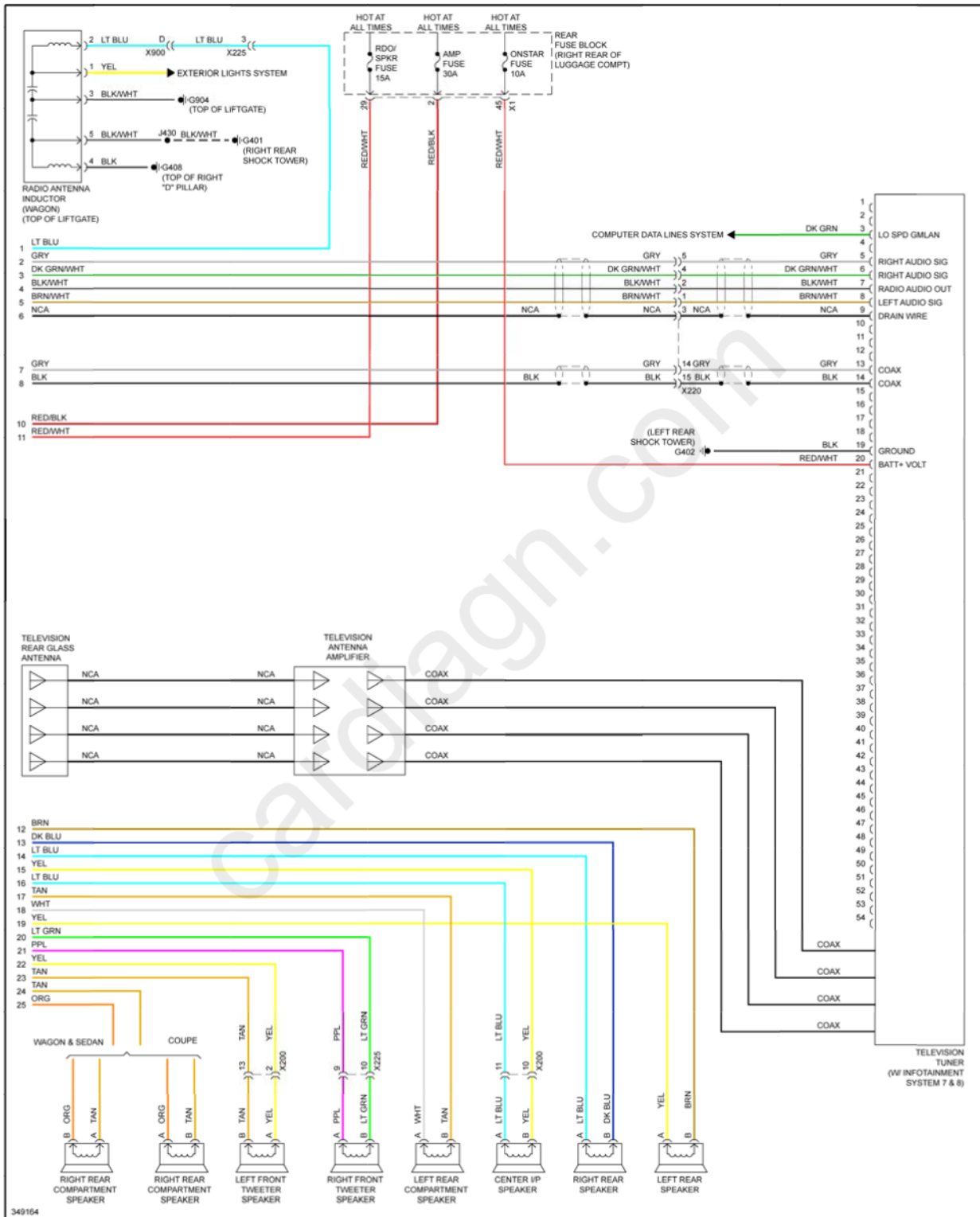
Fig. 102: Radio Circuit, W/ Surround Amplifier (4 of 4)
