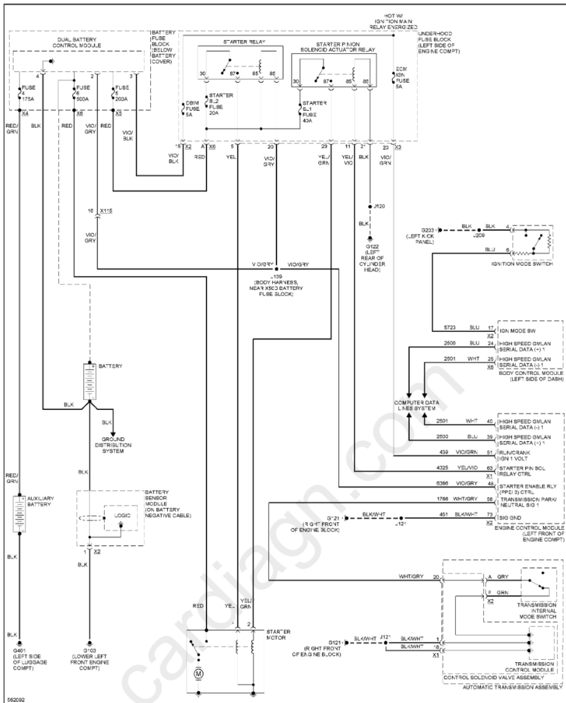
Fig. 120: Starting Circuit, W/ Start-Stop System
