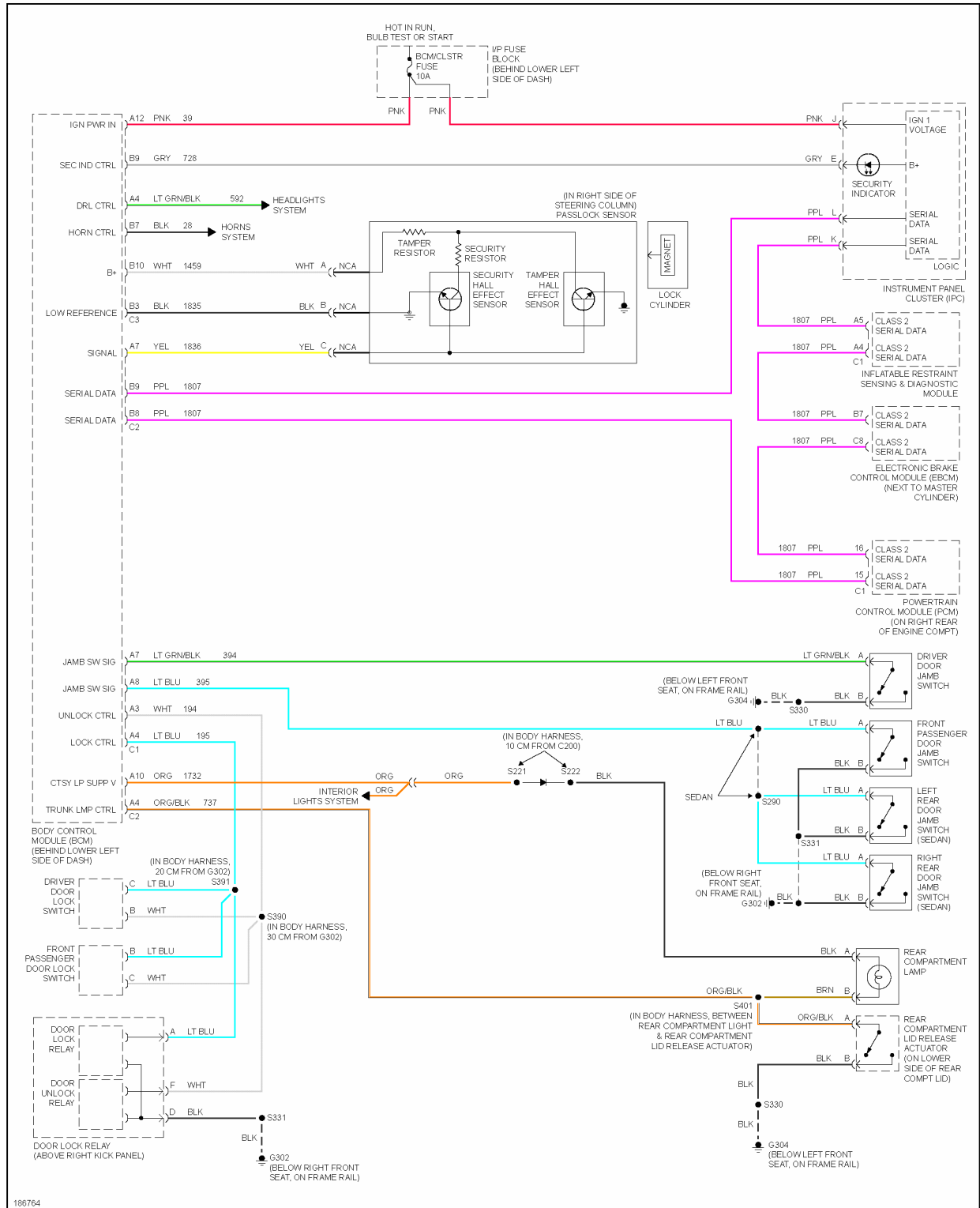
Fig. 4: Anti-theft Circuit
