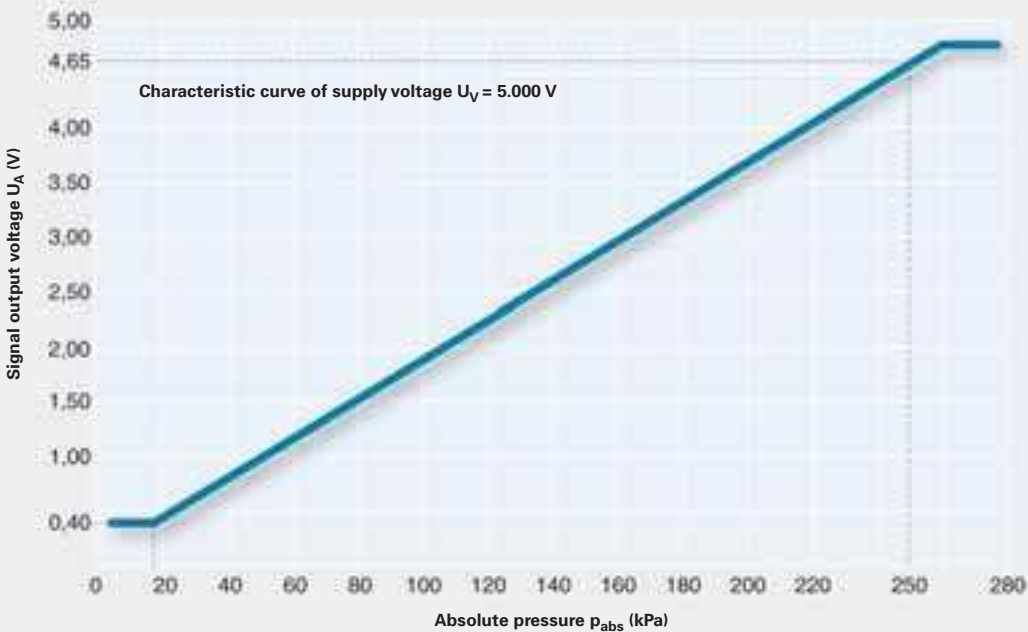
Signal pattern of intake manifold pressure sender
