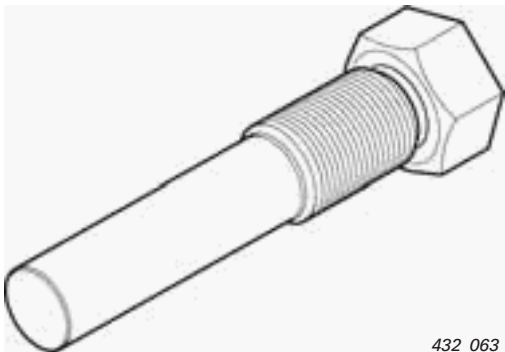
T10340 Locating screw For locating the crankshaft in order to set the valve timing
