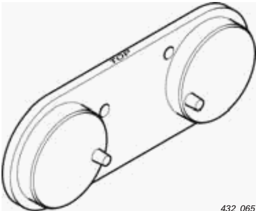
T10171 A Camshaft locating tool For locating the camshafts in position and checking and setting the valve timings
