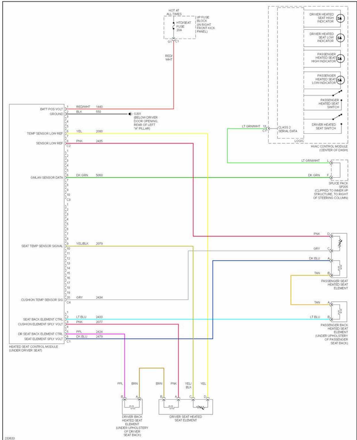
Fig. 48: Heated Seats Circuit
