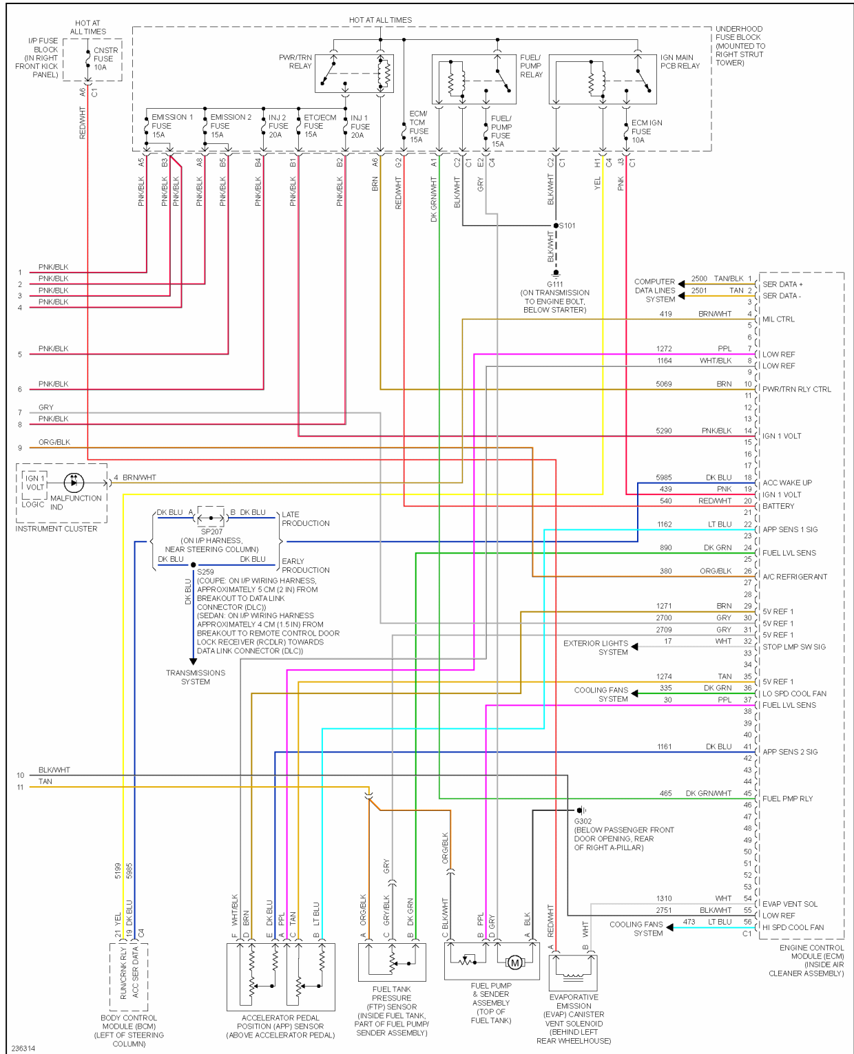
Fig. 27: 5.3L VIN C, Engine Performance Circuit (4 of 4)
