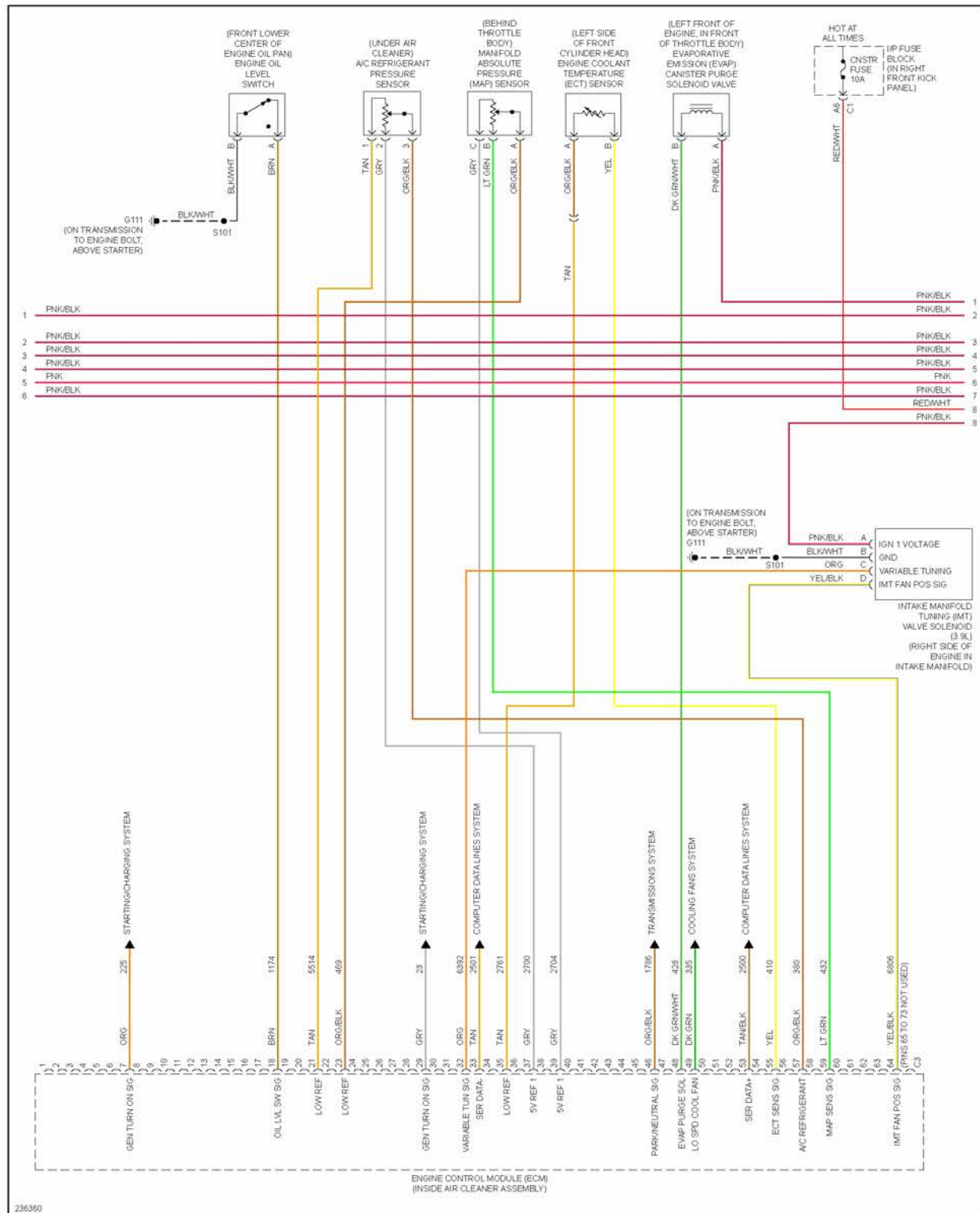
Fig. 18: 3.5L VIN K, Engine Performance Circuit (3 of 4)
