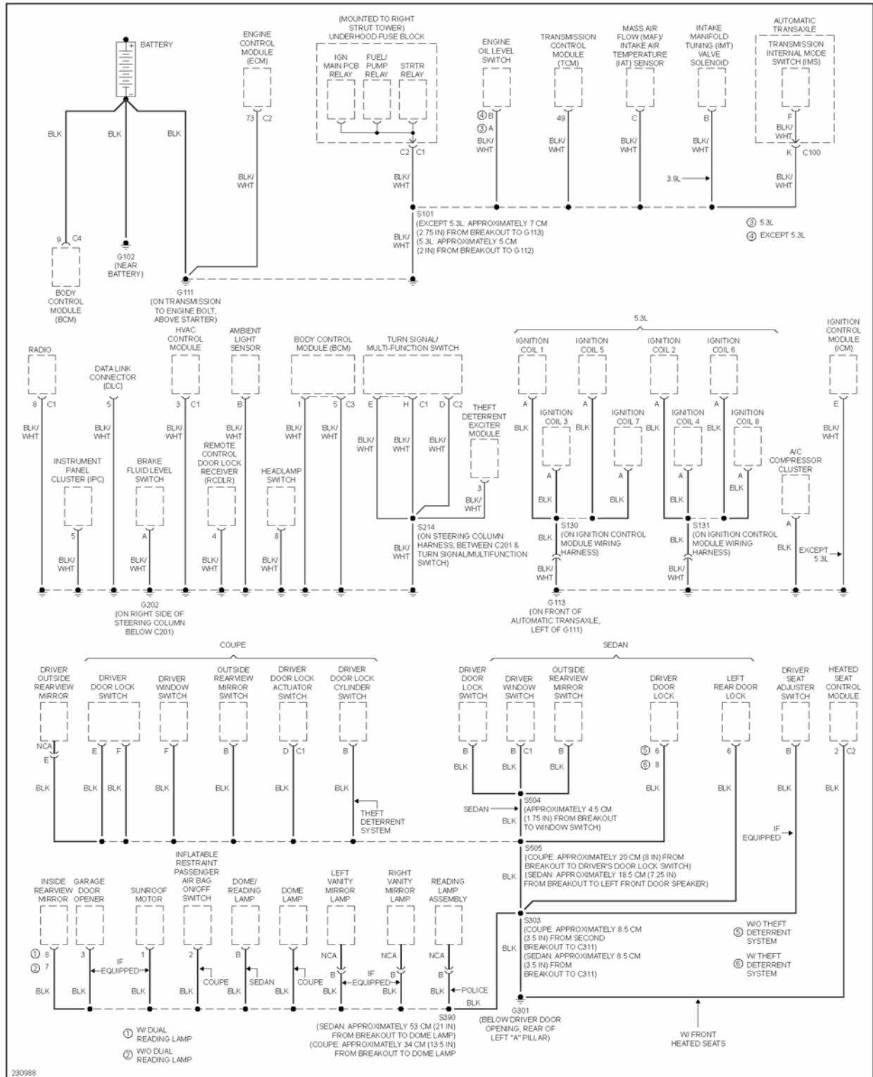
Fig. 31: Ground Distribution Circuit (1 of 3)
