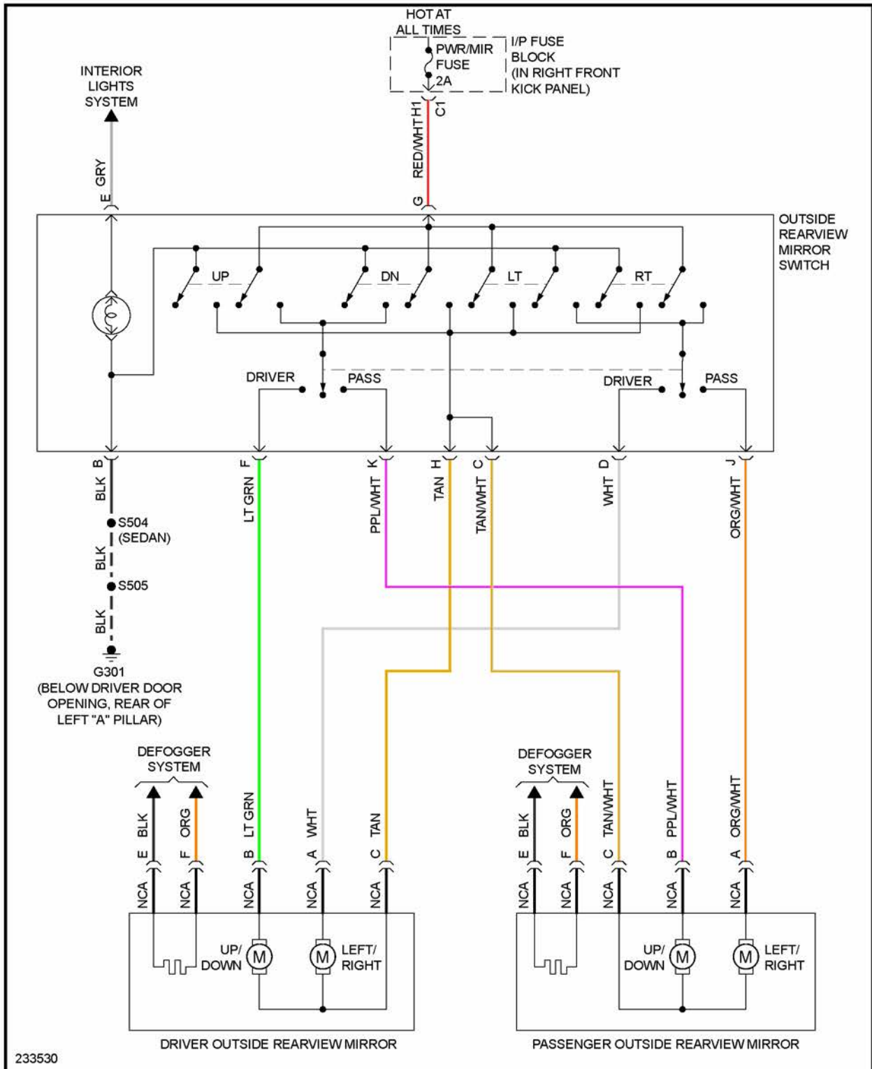
Fig. 47: Power Mirrors Circuit
