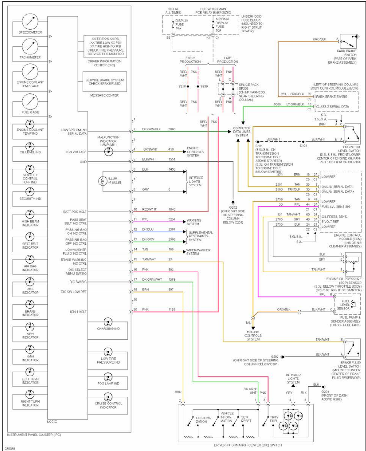
Fig. 37: Instrument Cluster Circuit
