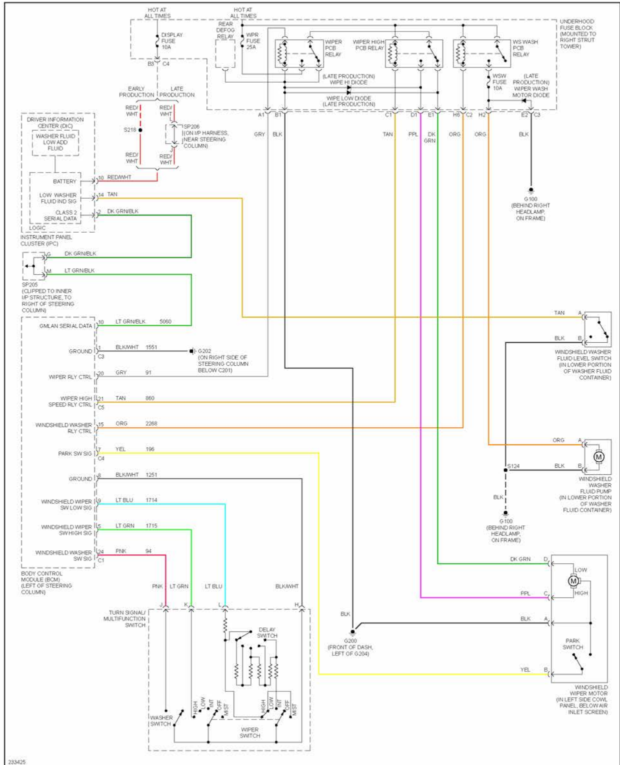
Fig. 67: Wiper/Washer Circuit
