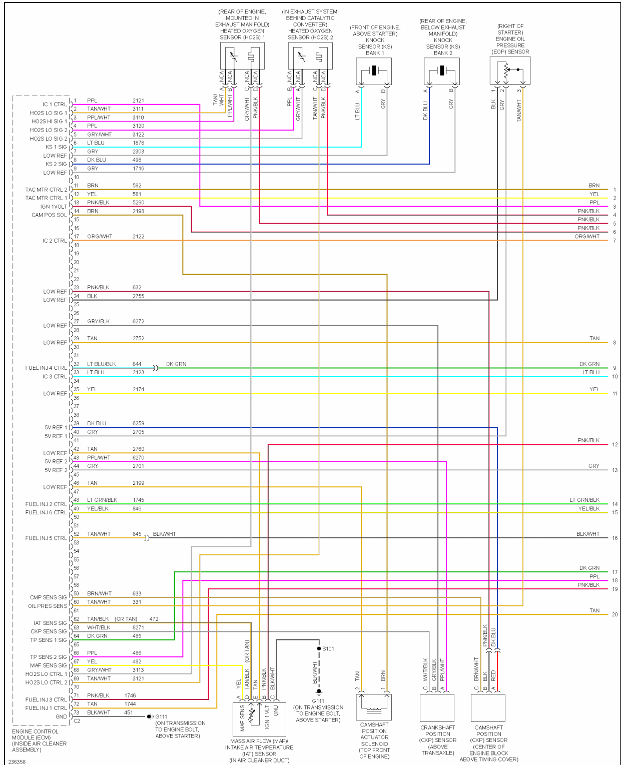
Fig. 20: 3.9L VIN 1, Engine Performance Circuit (1 of 4)
