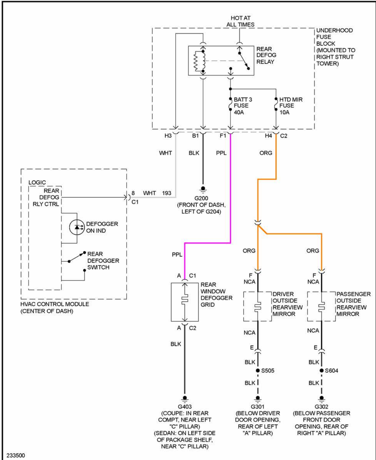
Fig. 15: Defoggers Circuit
