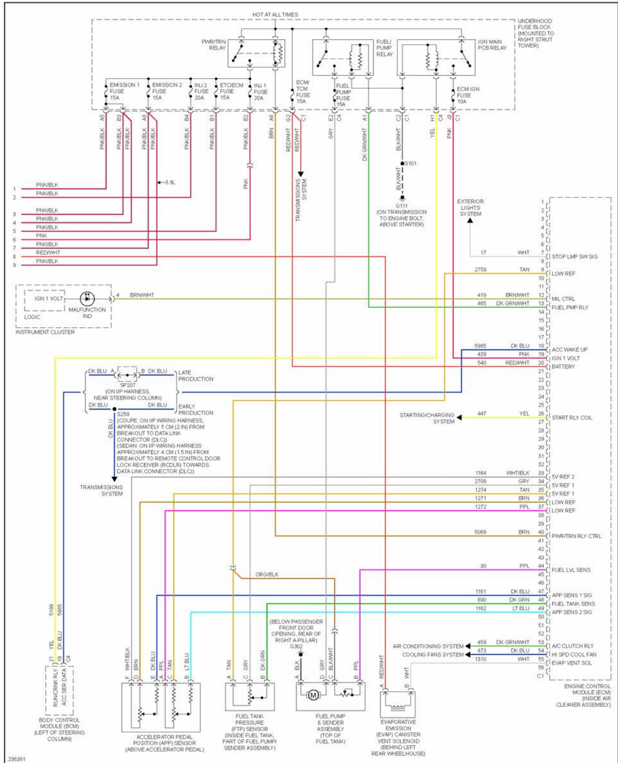
Fig. 23: 3.9L VIN 1, Engine Performance Circuit (4 of 4)
