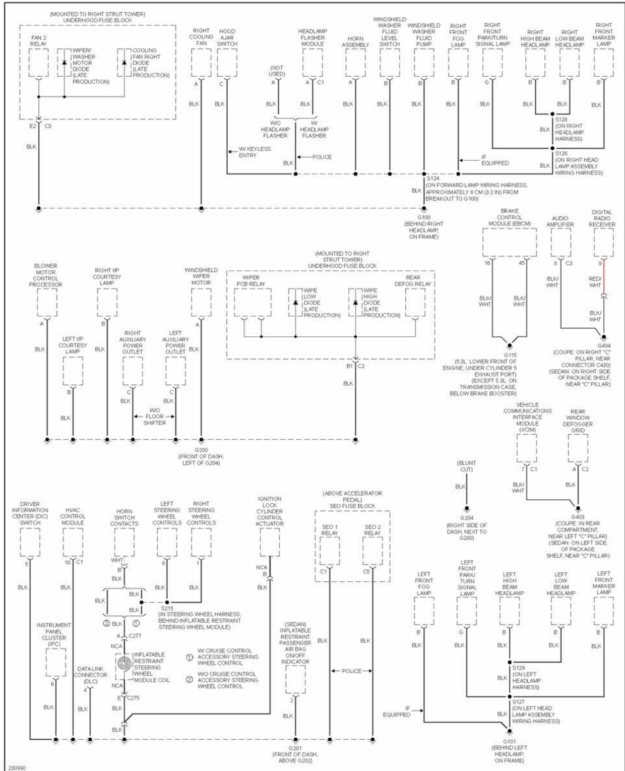
Fig. 33: Ground Distribution Circuit (3 of 3)
