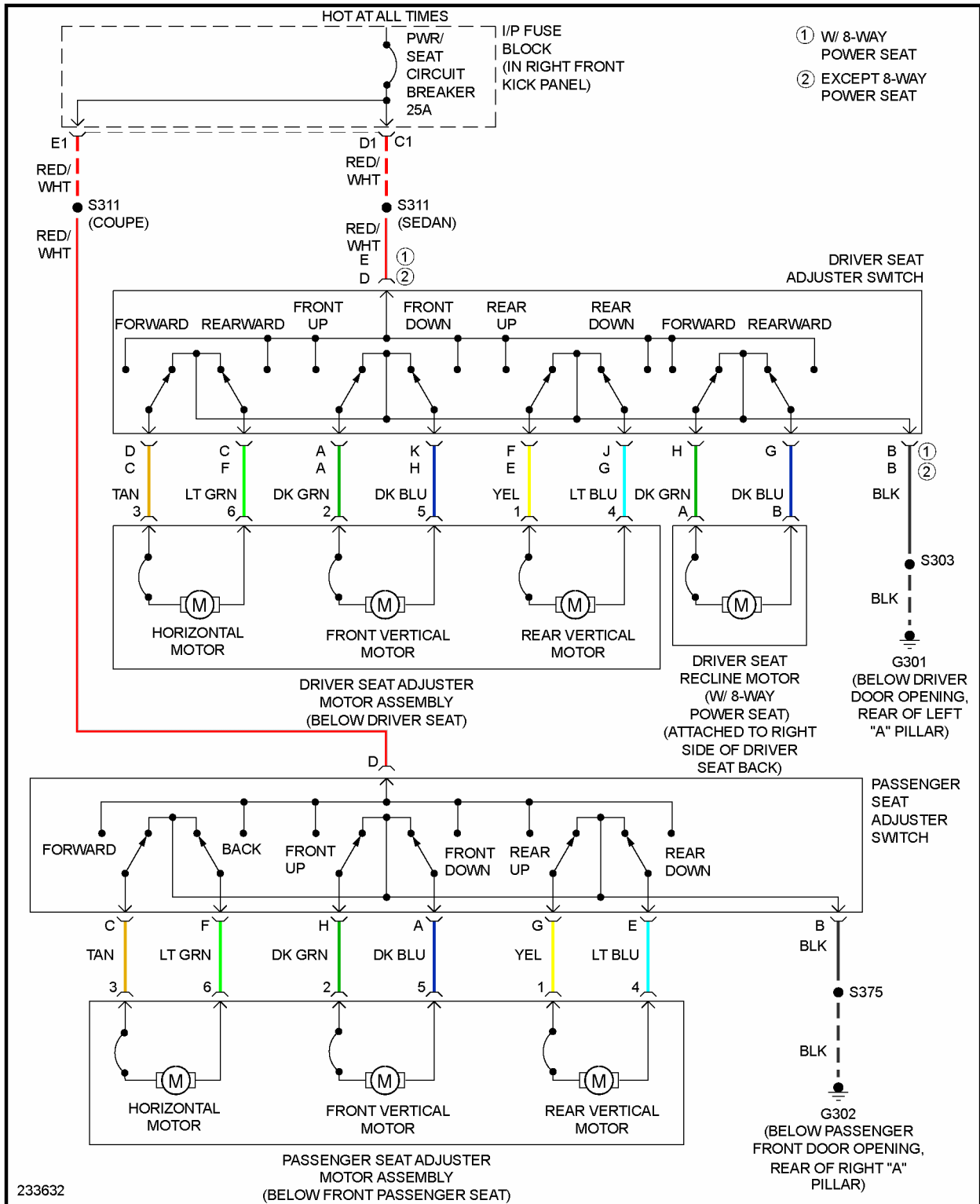
Fig. 49: Power Seat Circuit
