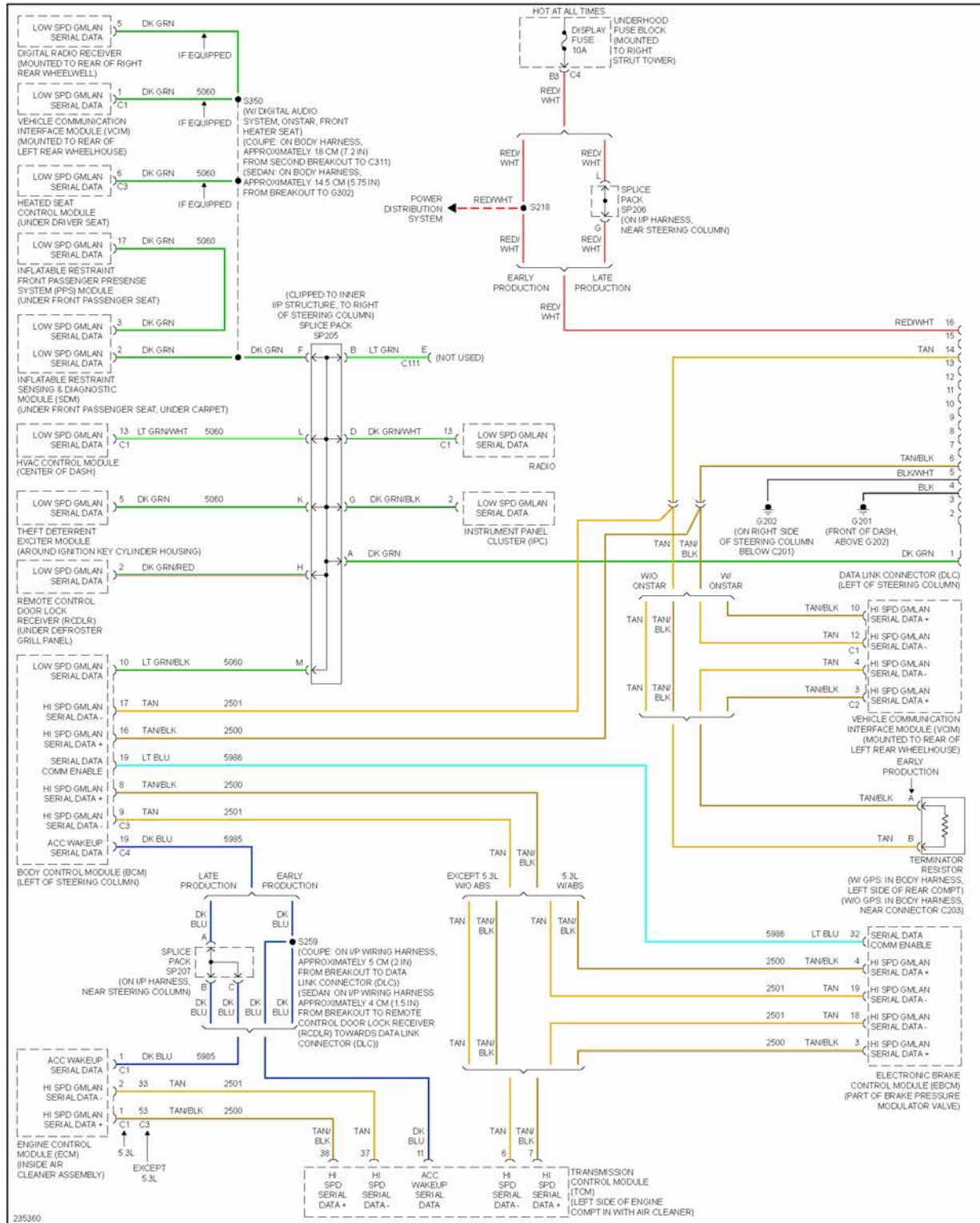
Fig. 11: Computer Data Lines Circuit
