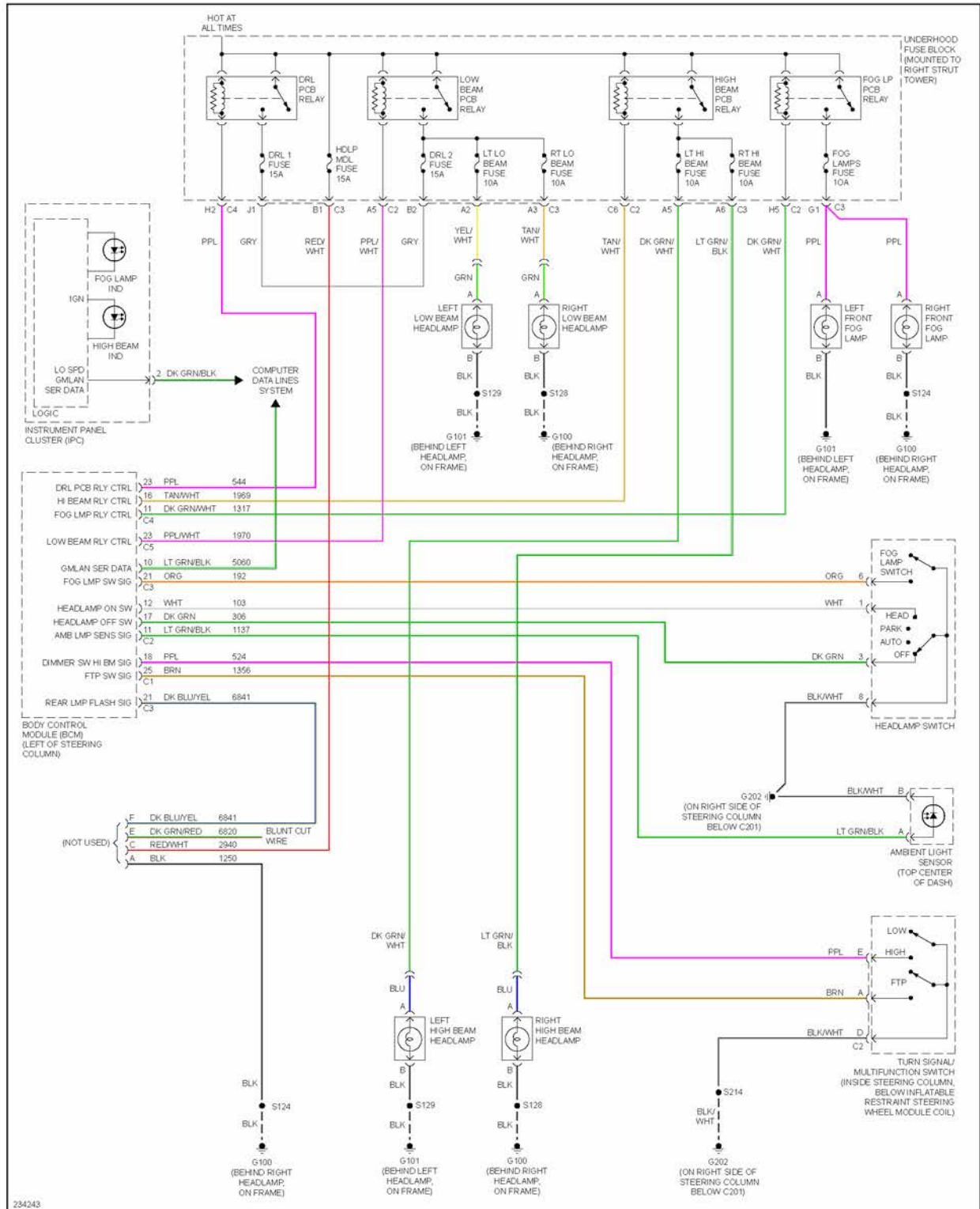
Fig. 34: Headlights Circuit, W/ Police Option
