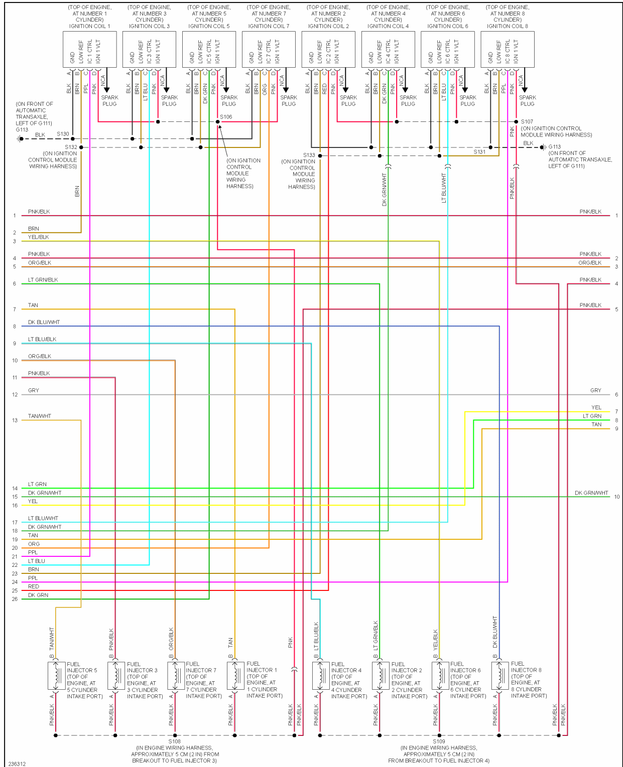
Fig. 25: 5.3L VIN C, Engine Performance Circuit (2 of 4)
