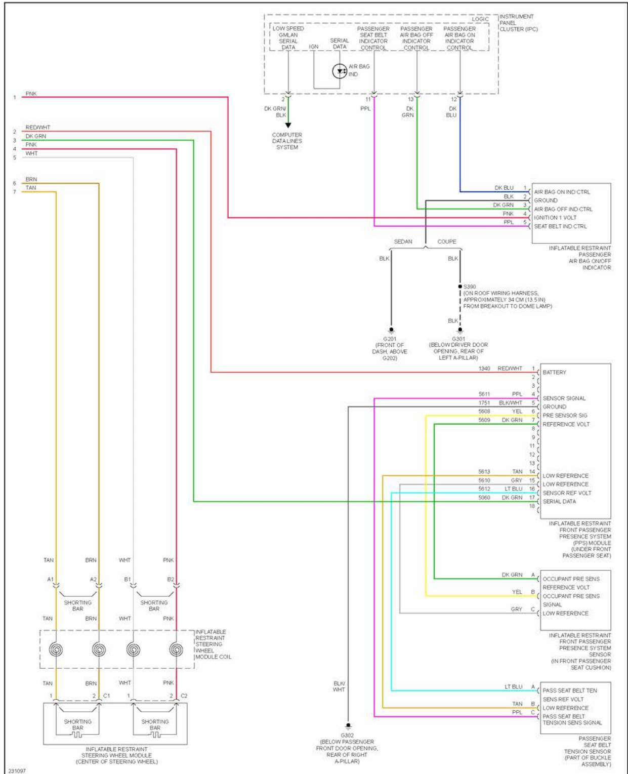
Fig. 63: Supplemental Restraints Circuit (3 of 3)
