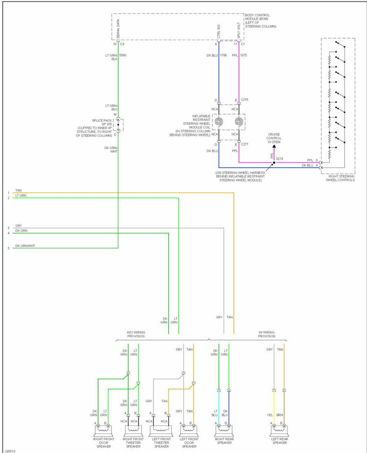
Fig. 53: Radio Circuit, Police Option (2 of 2)
