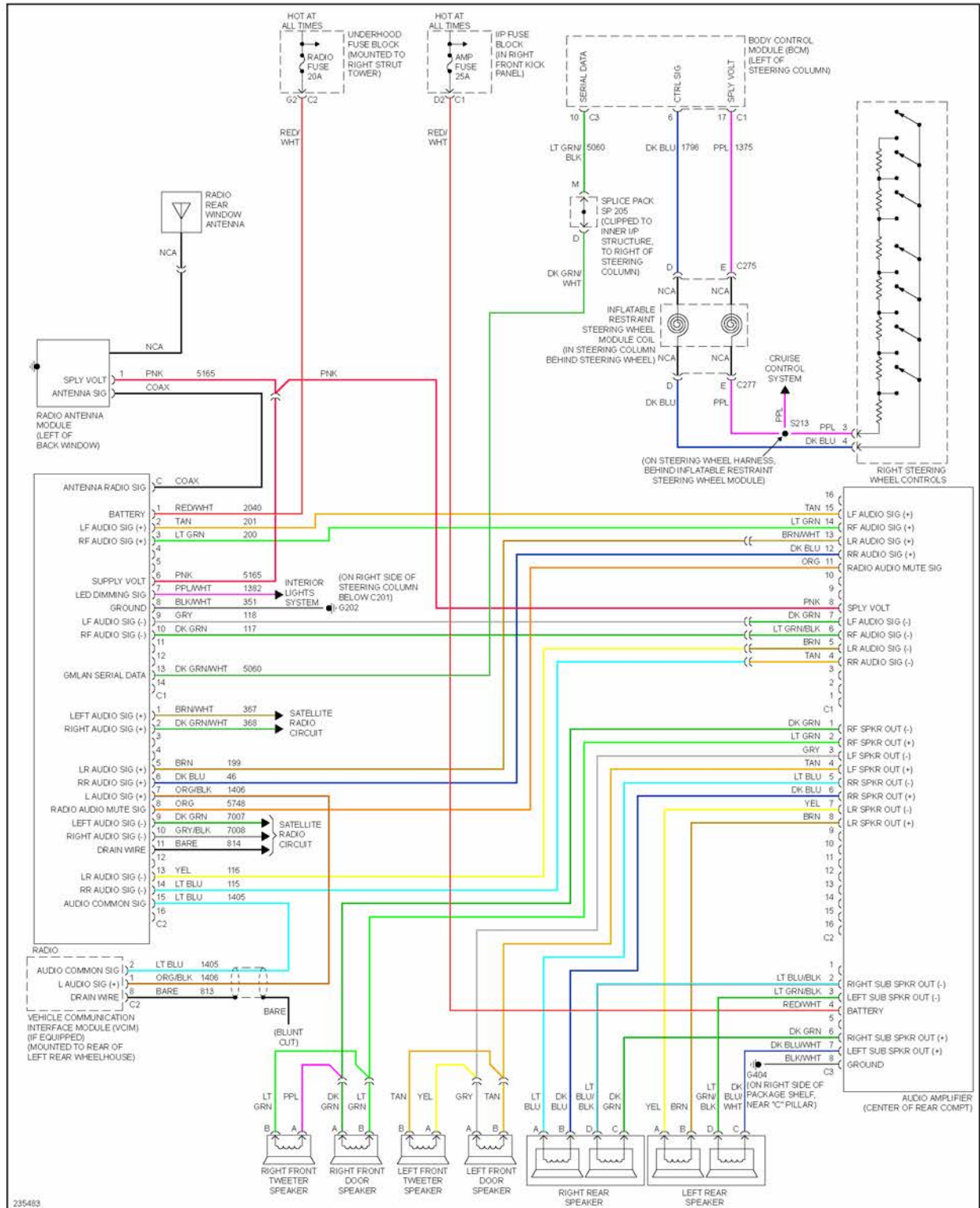
Fig. 54: Radio Circuit, W/ Amplifier
