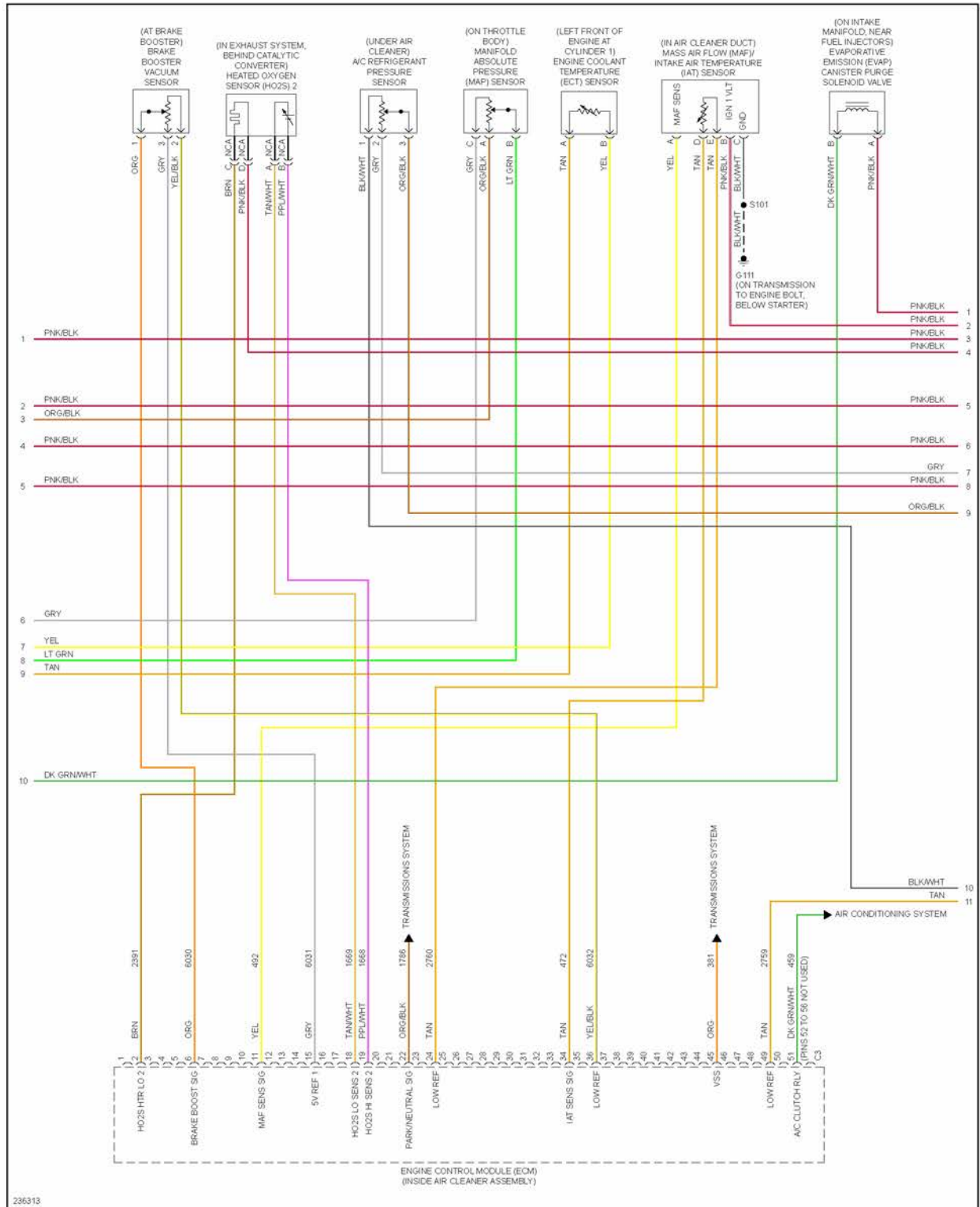
Fig. 26: 5.3L VIN C, Engine Performance Circuit (3 of 4)
