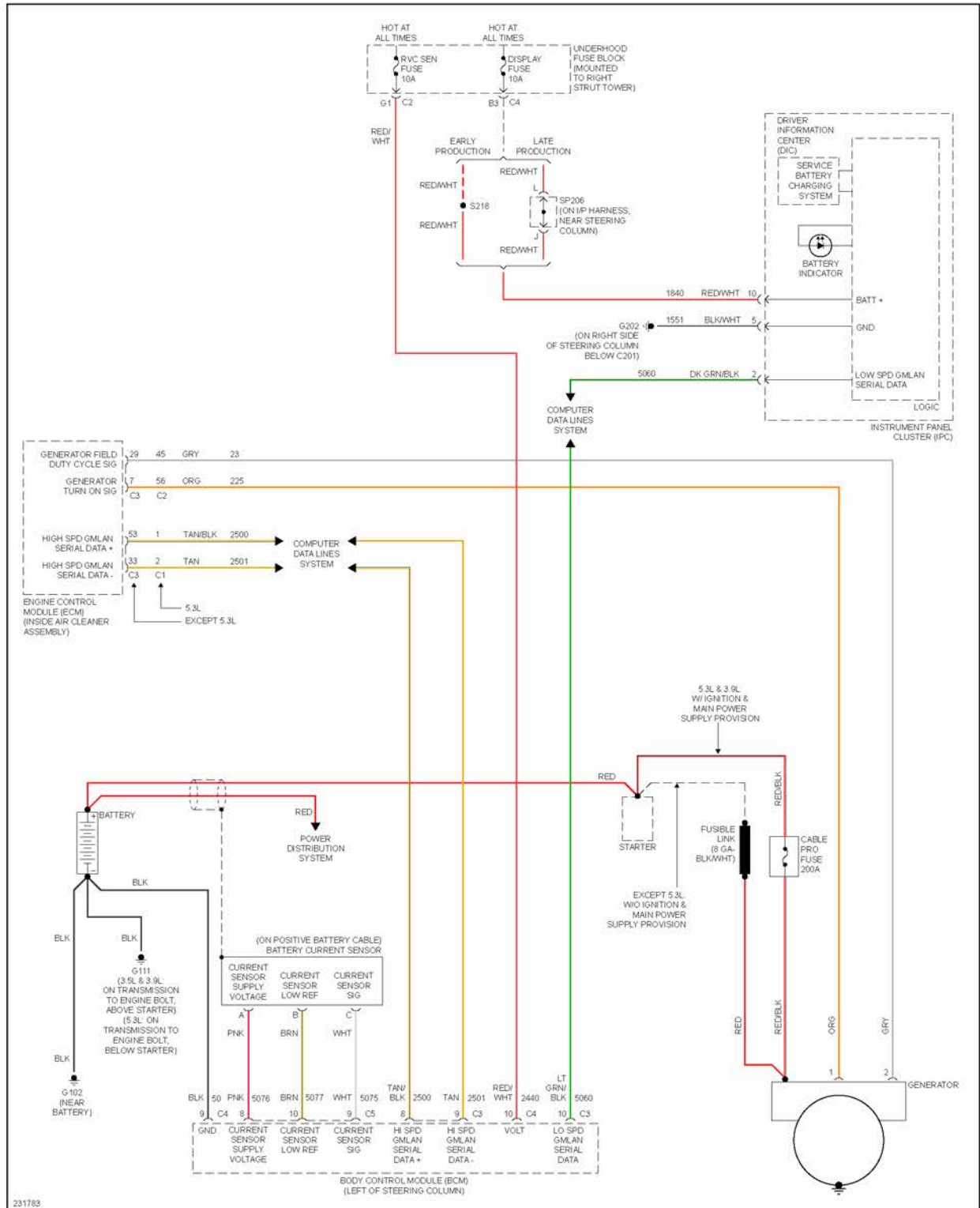
Fig. 59: Charging Circuit
