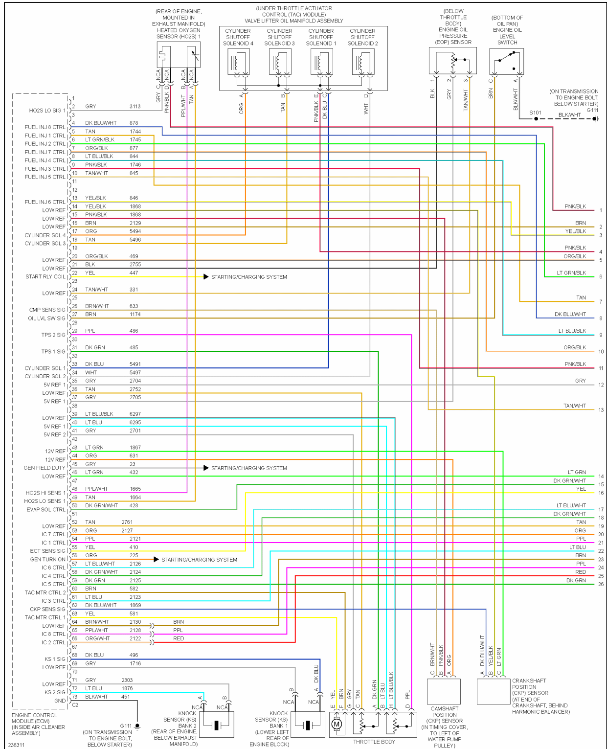
Fig. 24: 5.3L VIN C, Engine Performance Circuit (1 of 4)
