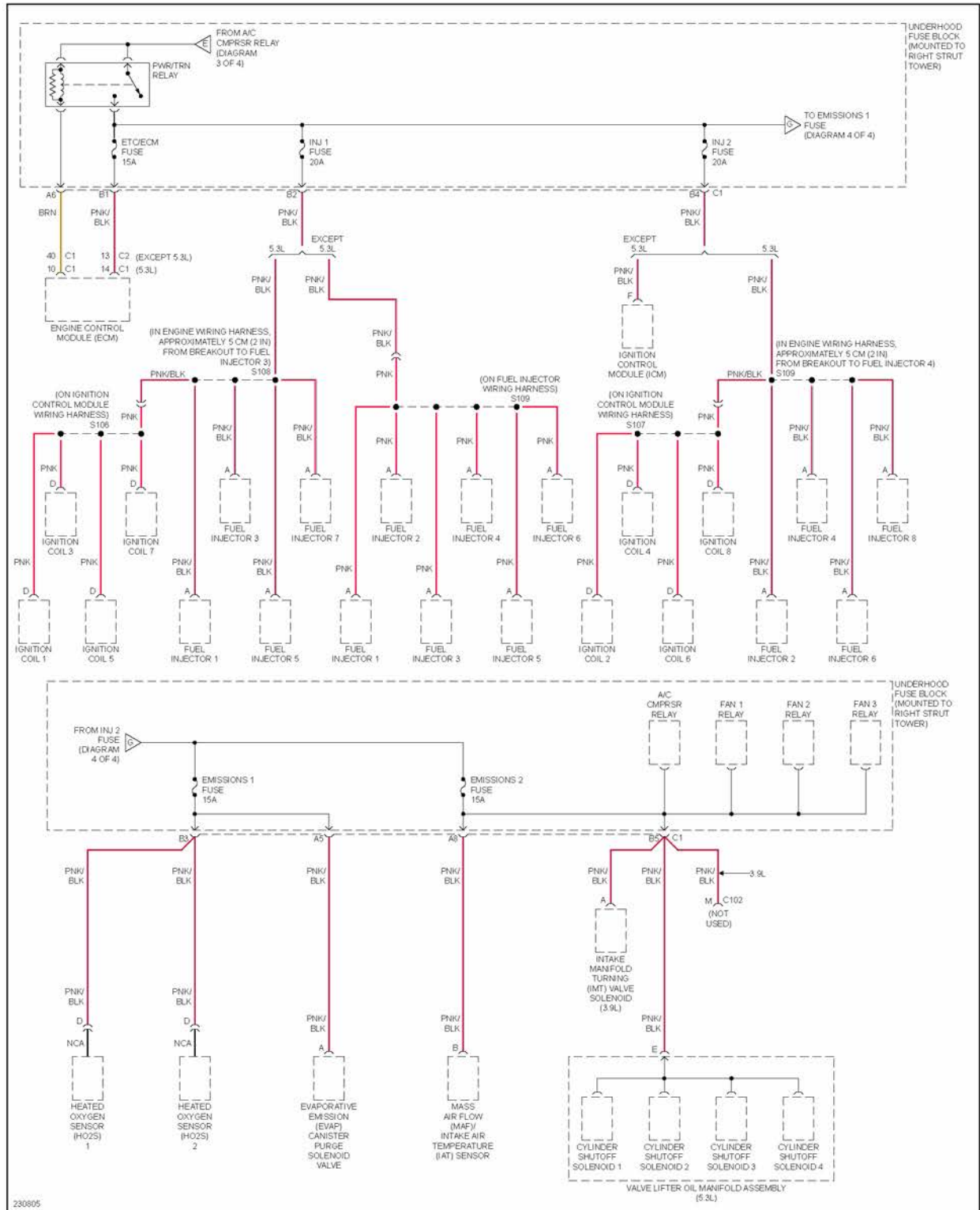
Fig. 43: Power Distribution Circuit (4 of 4)
