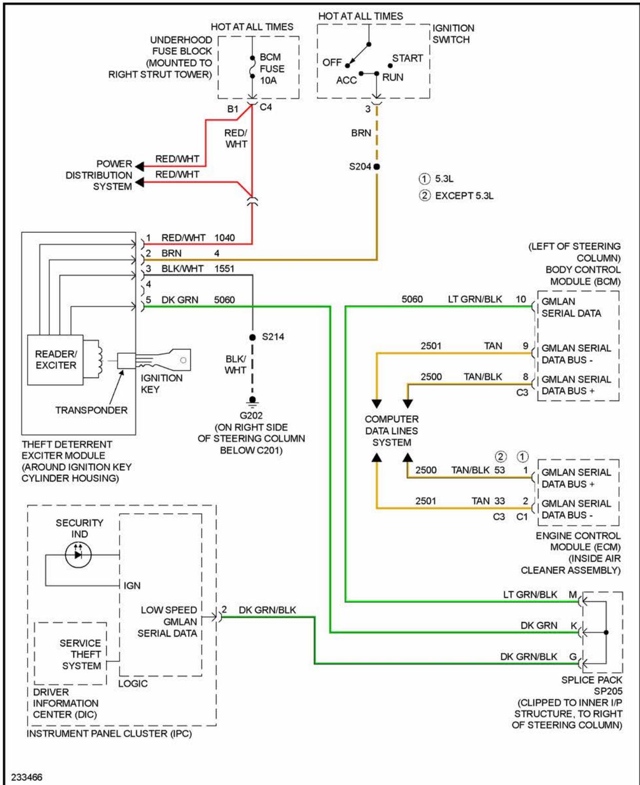
Fig. 8: Pass-Key Circuit
