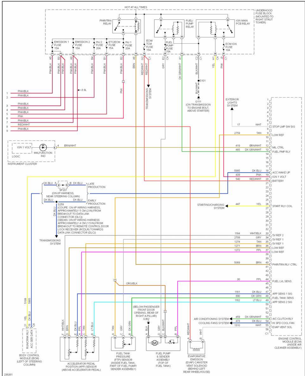
Fig. 19: 3.5L VIN K, Engine Performance Circuit (4 of 4)
