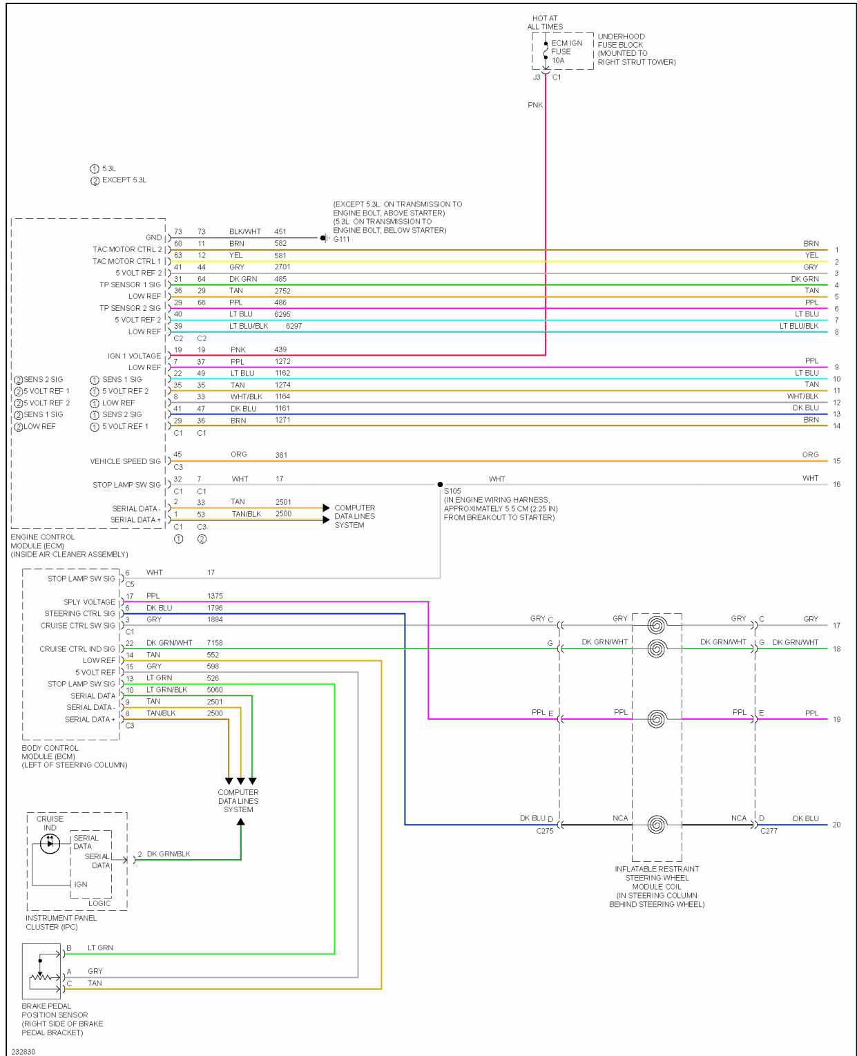
Fig. 13: Cruise Control Circuit (1 of 2)
