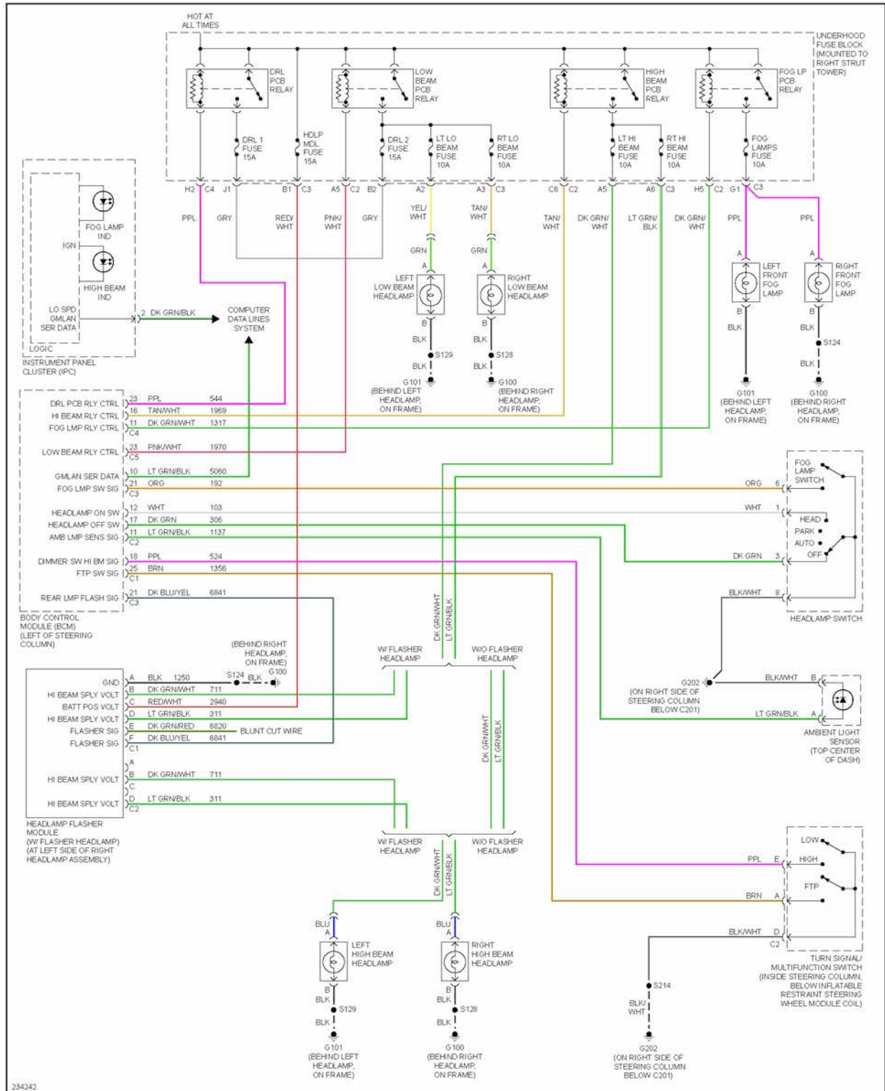
Fig. 35: Headlights Circuit, W/O Police Option
