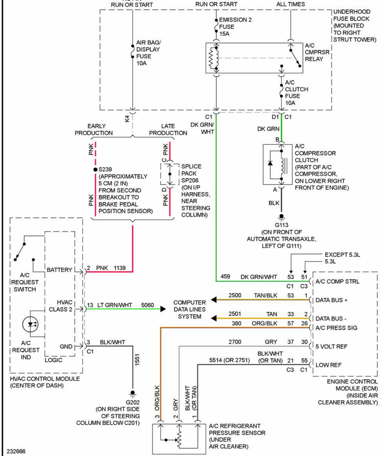
Fig. 1: Compressor Circuit
