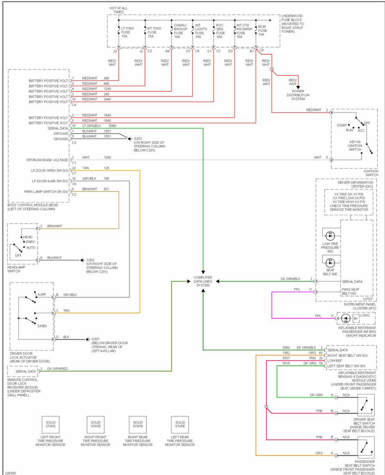
Fig. 66: Warning Systems Circuit
