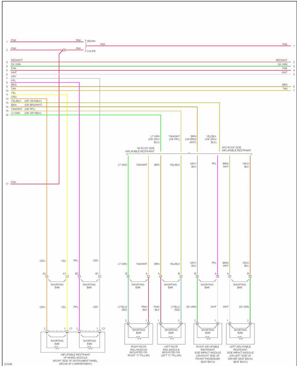
Fig. 62: Supplemental Restraints Circuit (2 of 3)
