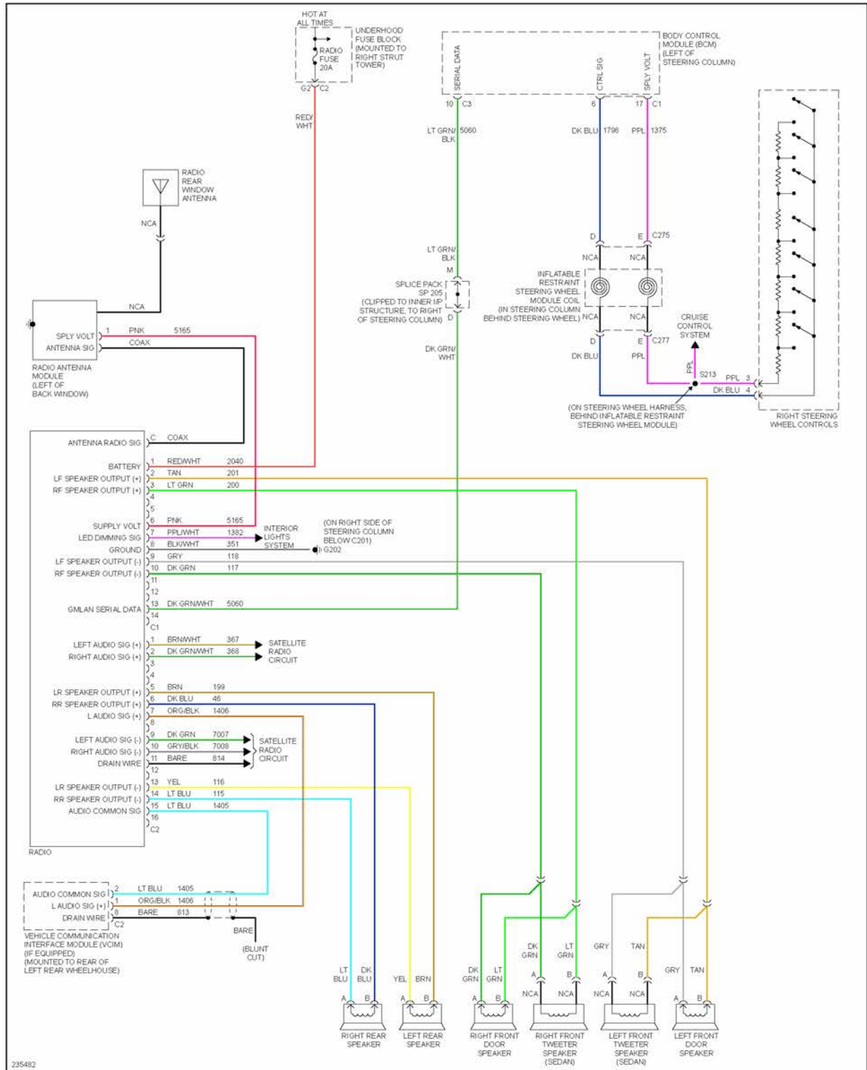
Fig. 55: Radio Circuit, W/O Amplifier
