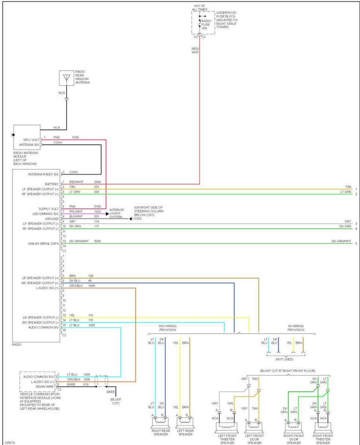
Fig. 52: Radio Circuit, Police Option (1 of 2)
