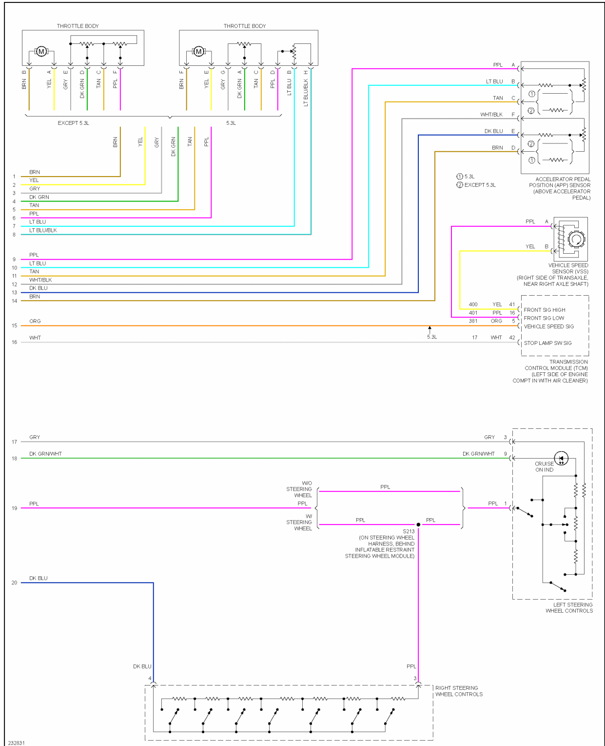
Fig. 14: Cruise Control Circuit (2 of 2)
