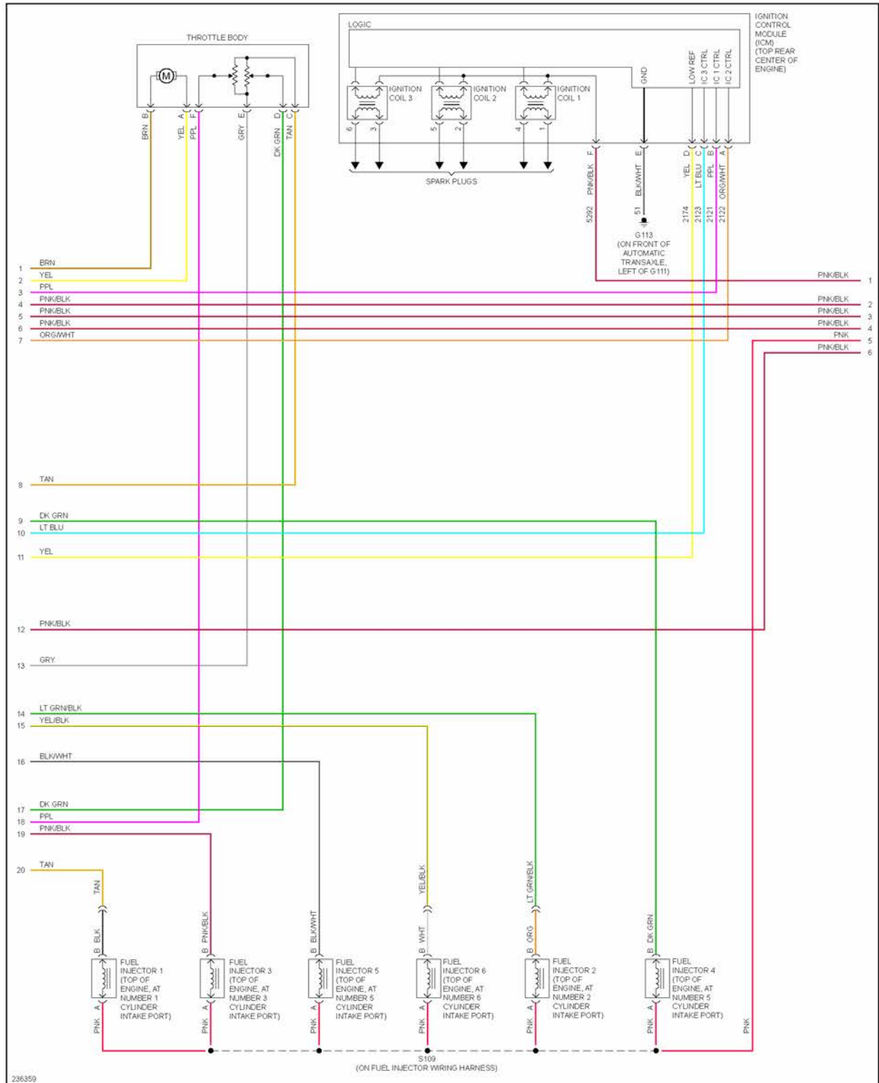
Fig. 17: 3.5L VIN K, Engine Performance Circuit (2 of 4)
