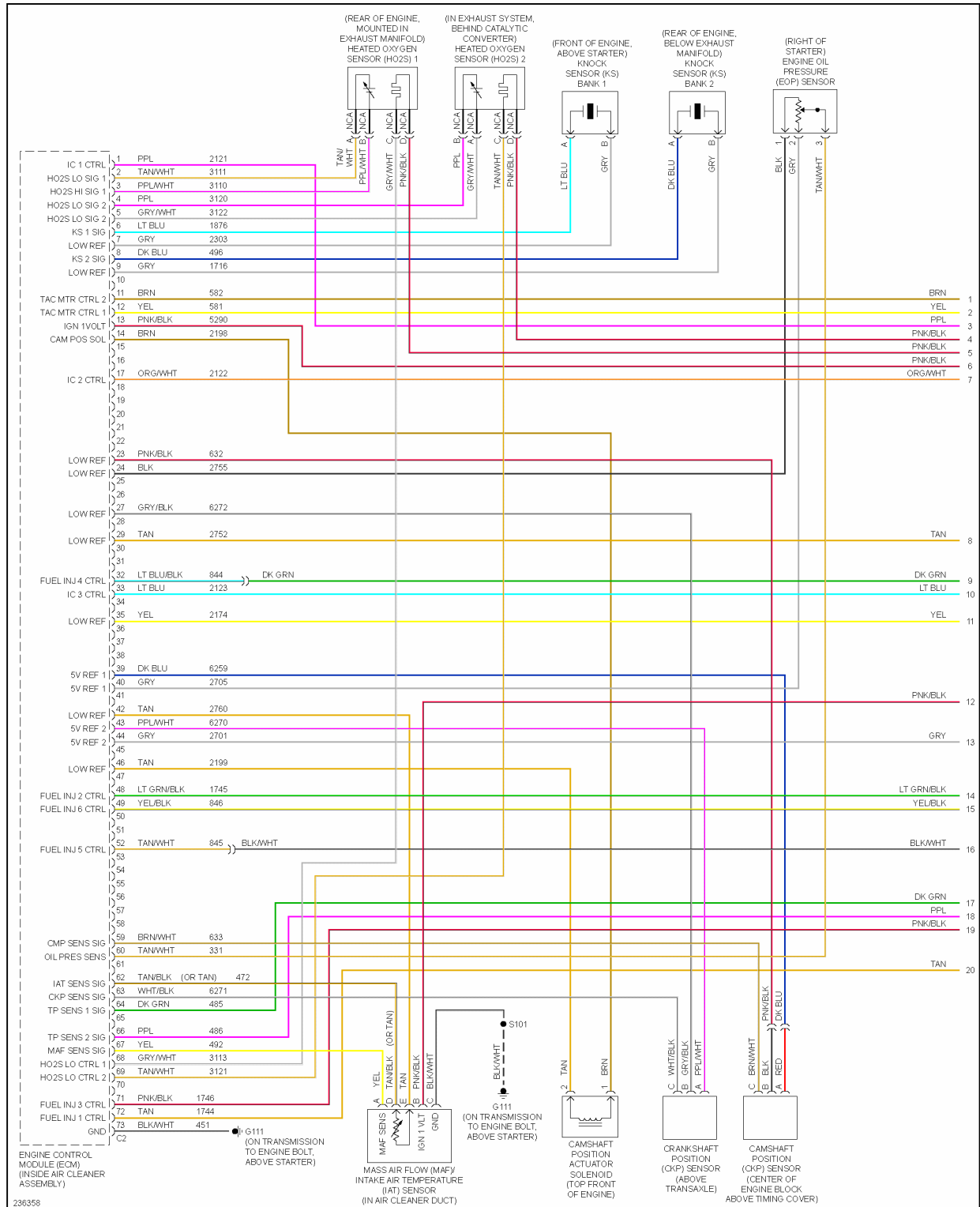
Fig. 16: 3.5L VIN K, Engine Performance Circuit (1 of 4)
