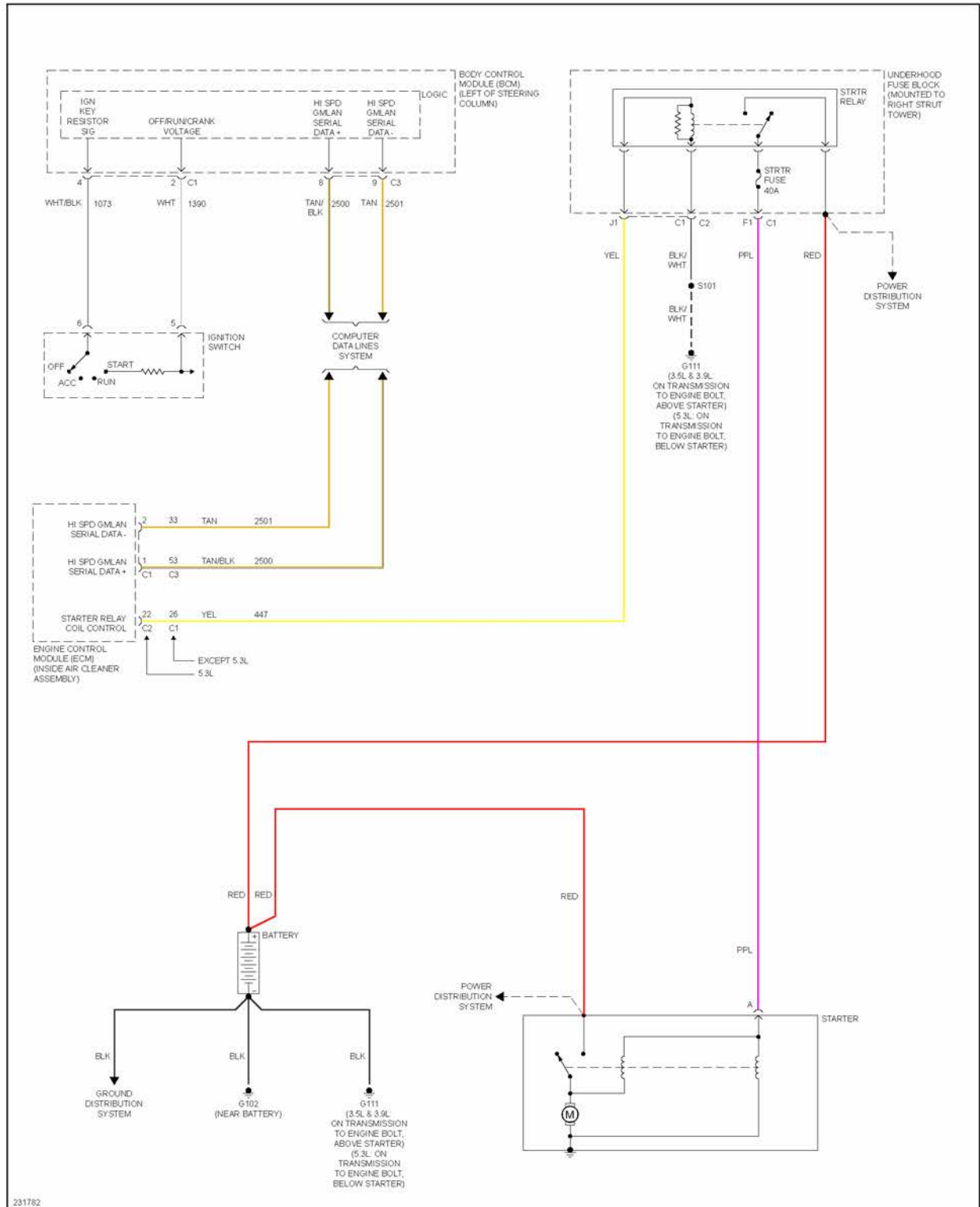
Fig. 60: Starting Circuit
