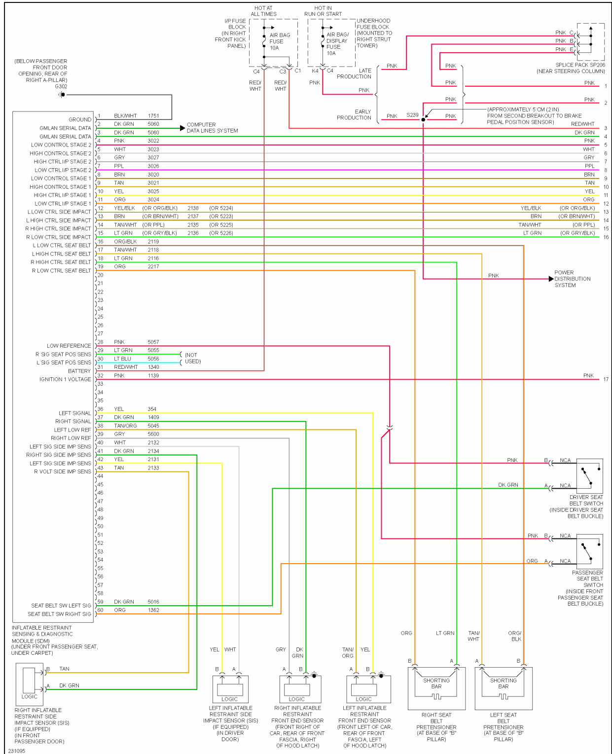
Fig. 61: Supplemental Restraints Circuit (1 of 3)
