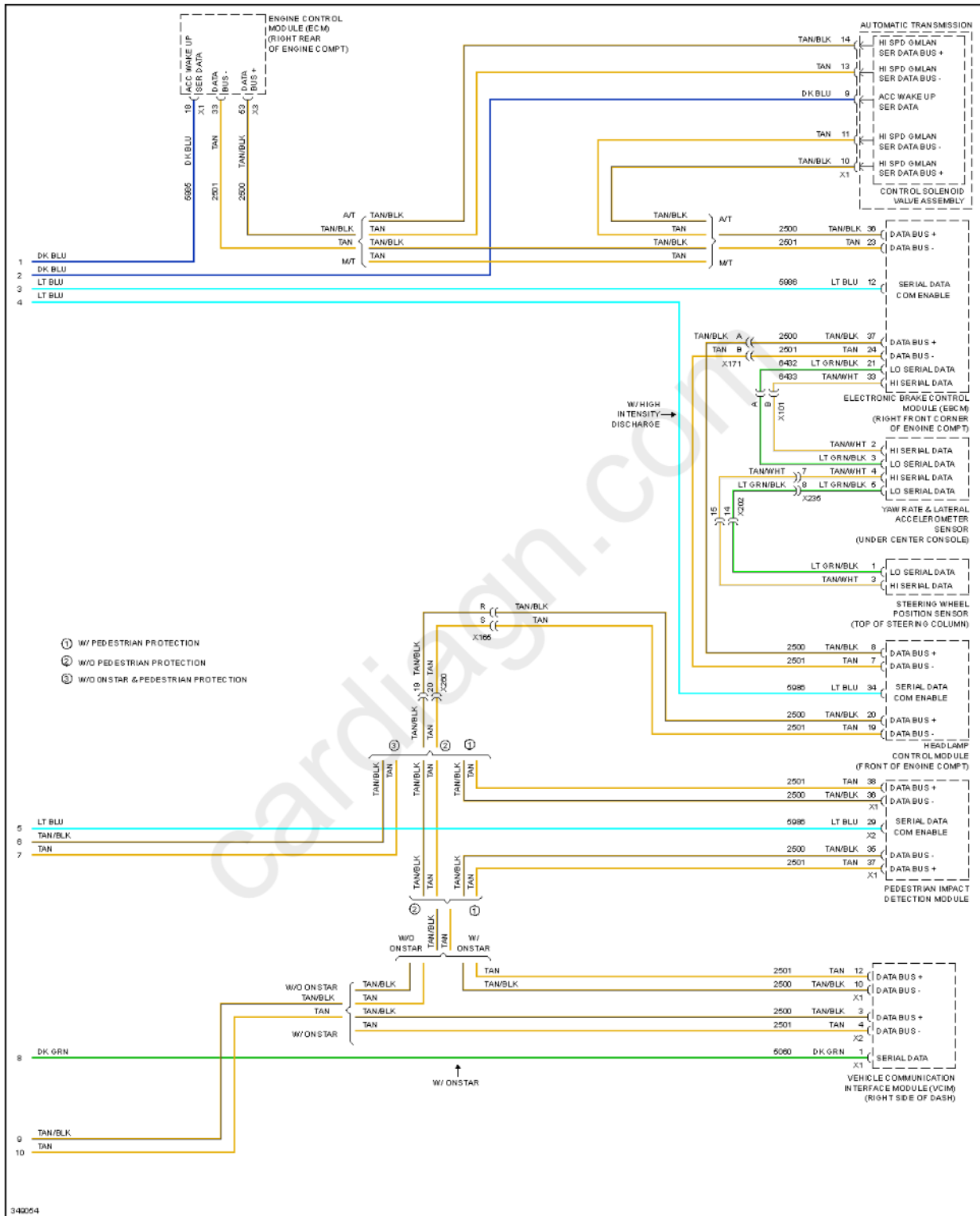
Fig. 20: 6.2L VIN P, Computer Data Lines Circuit (3 of 3)
