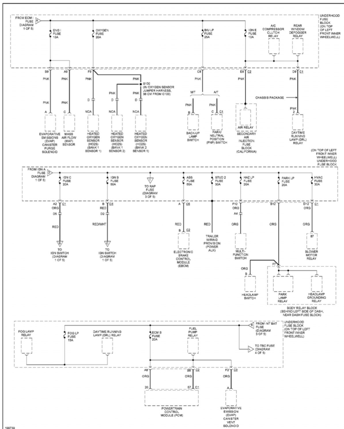
Fig. 29: Power Distribution Circuit (2 of 5)
