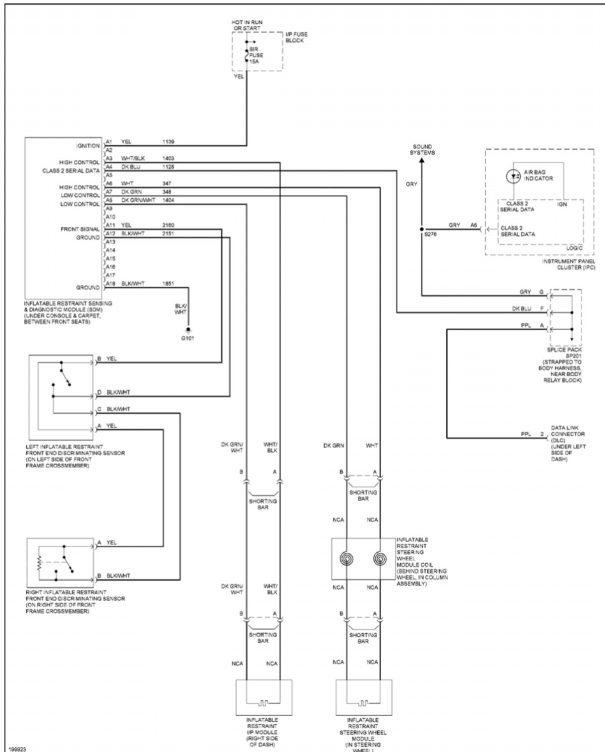
Fig. 50: Supplemental Restraints Circuit
