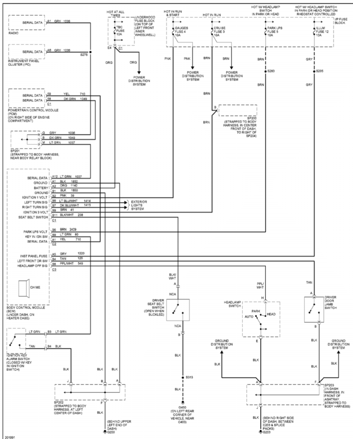
Fig. 55: Warning Systems Circuit
