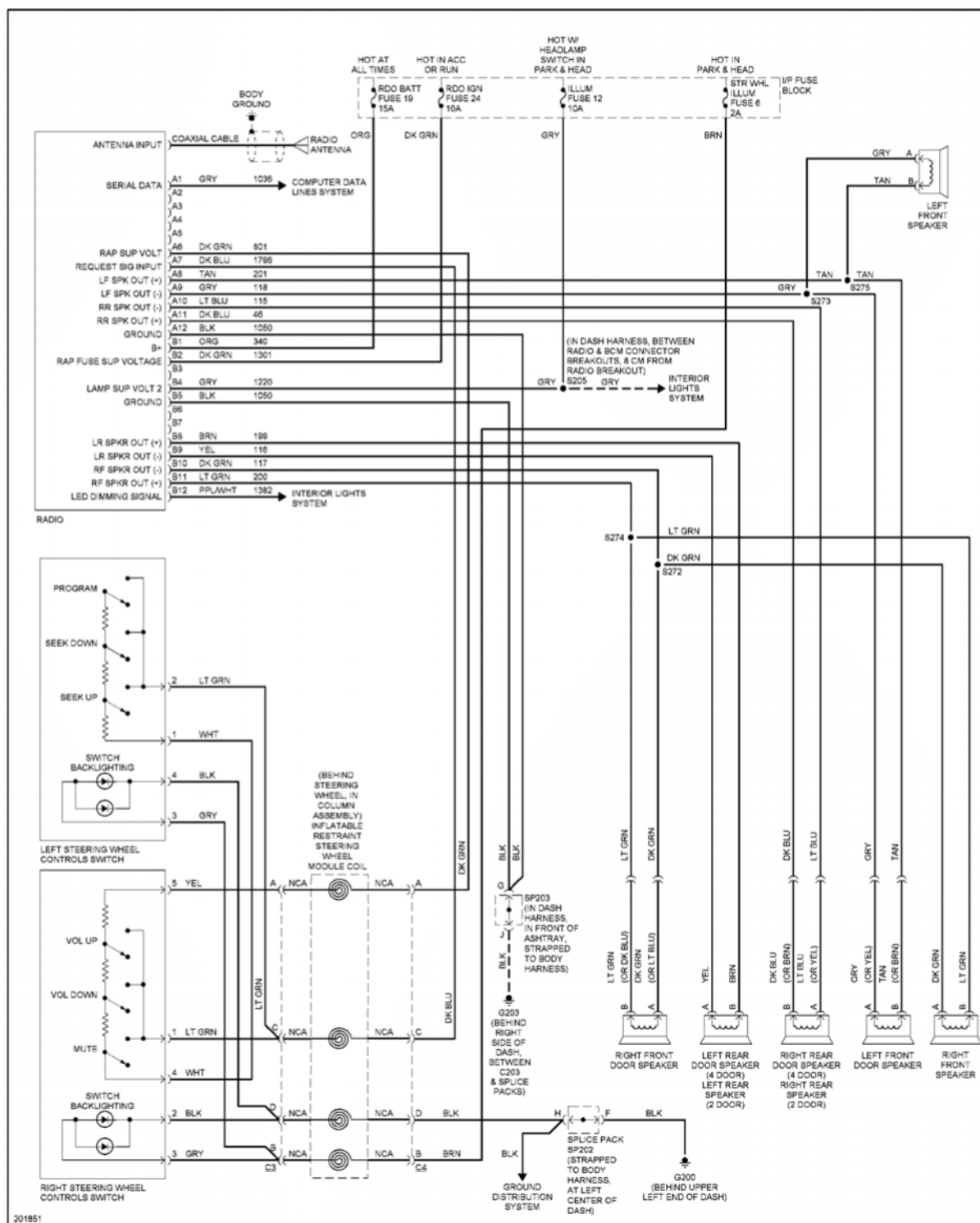
Fig. 44: Radio Circuit
