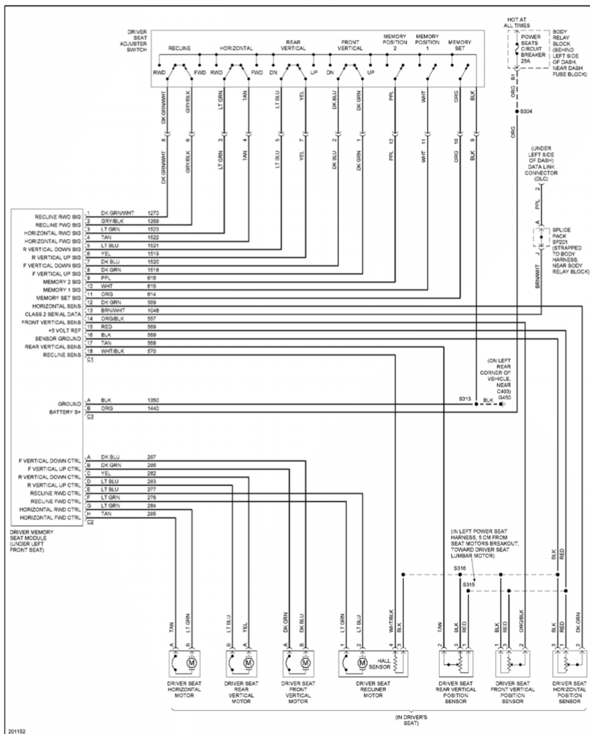
Fig. 27: Driver's Memory Seat Circuit
