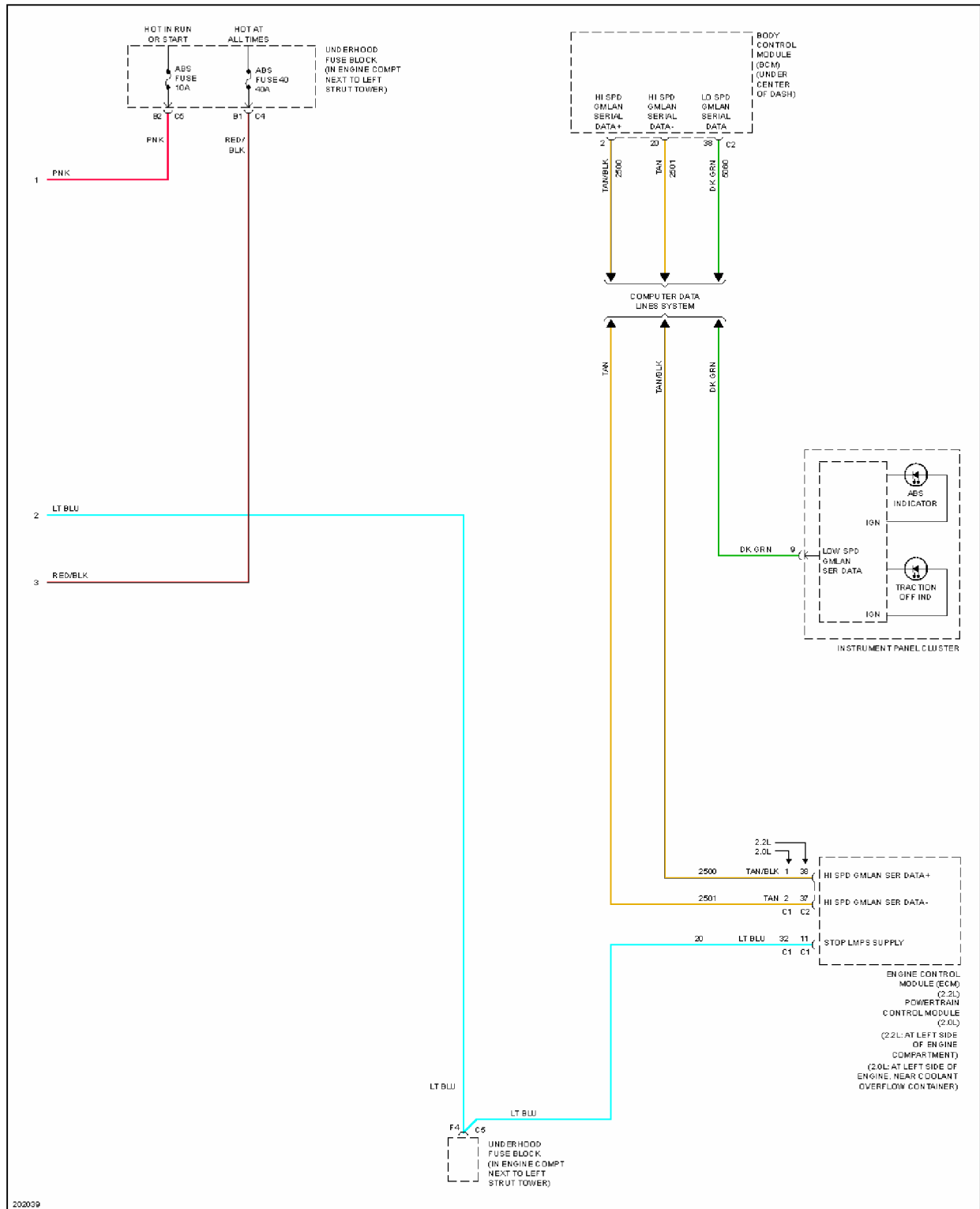
Fig. 8: Anti-lock Brakes Circuit (2 of 2)
