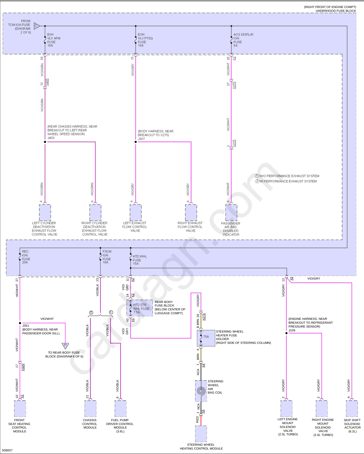
Fig 5: Power Distribution Circuit (5 of 6)
