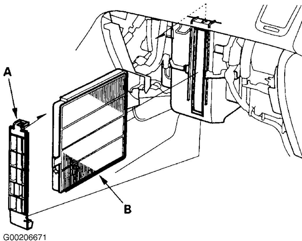
Fig. 6: Removing Dust & Pollen Filter
