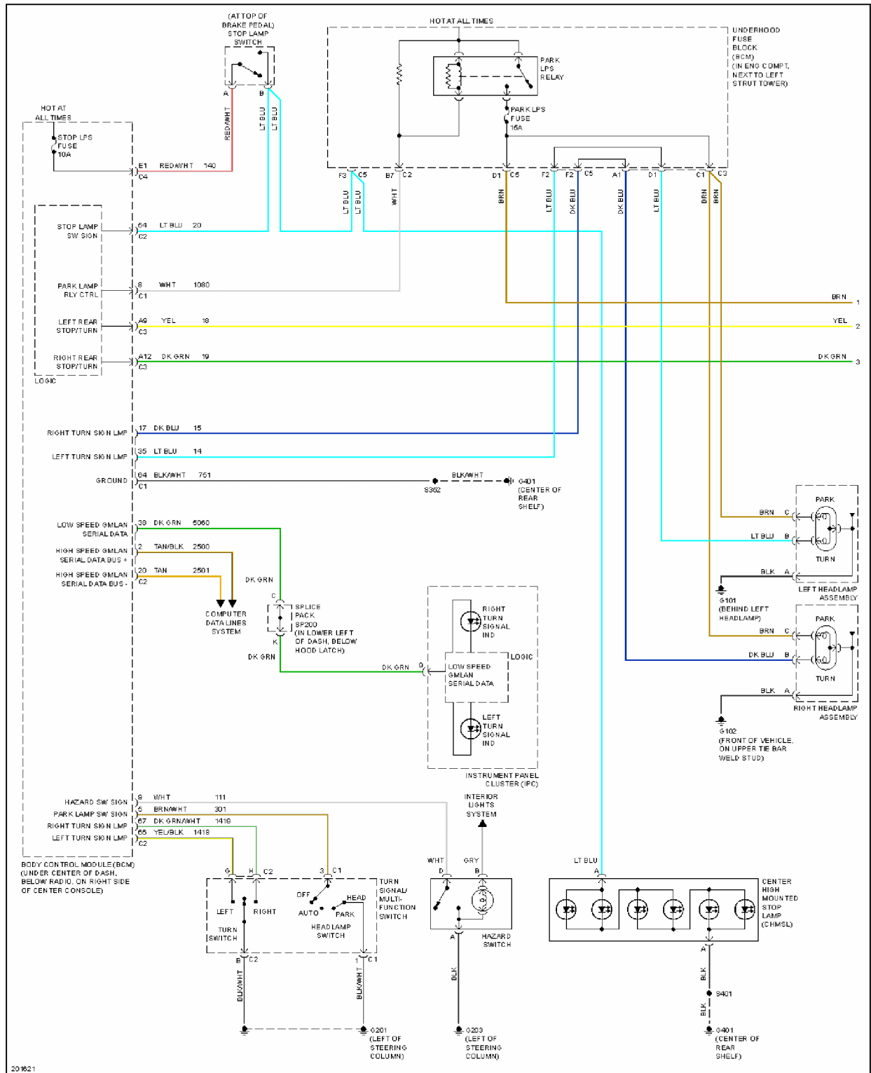
Fig. 30: Exterior Lamps Circuit (1 of 2)
