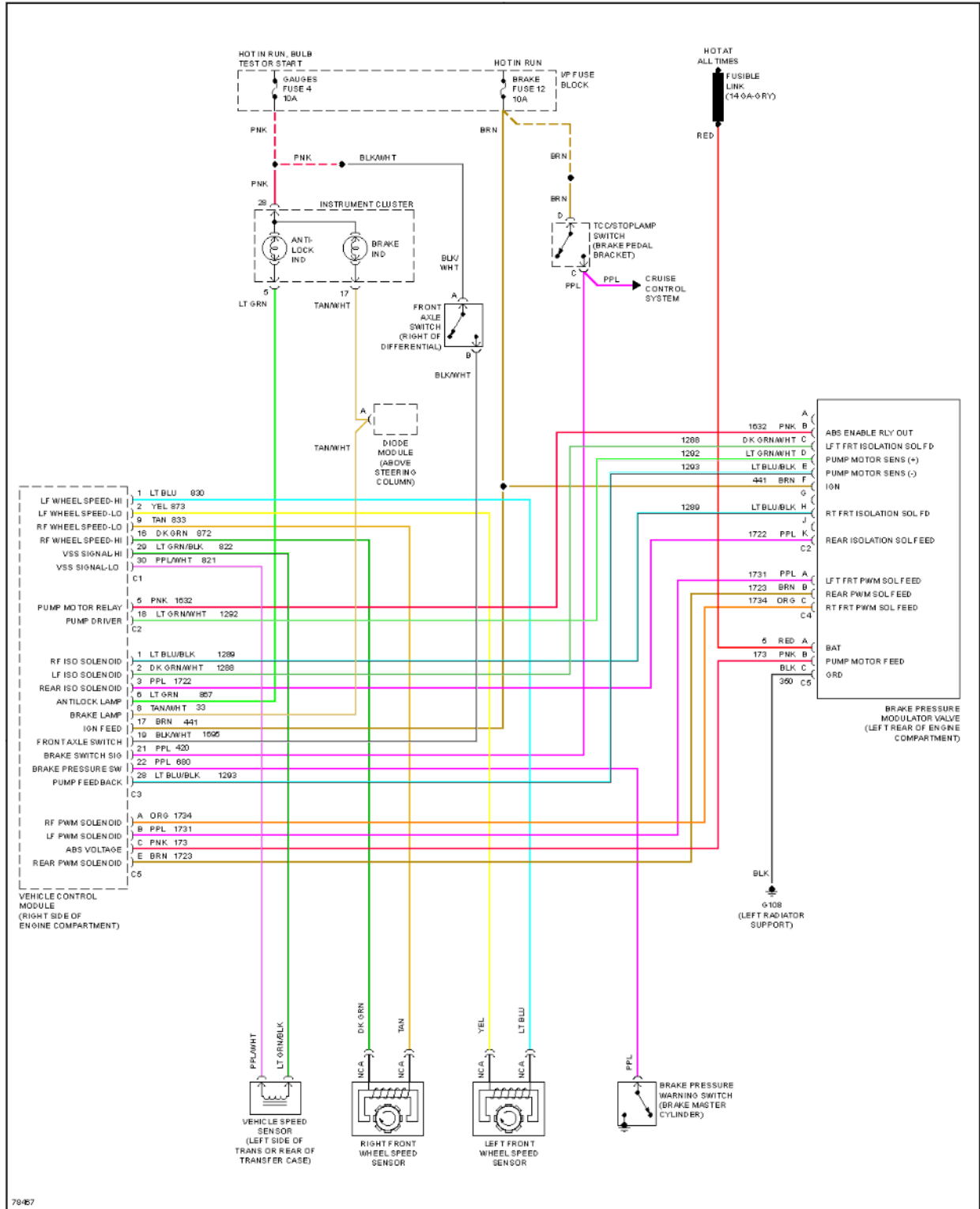
Fig. 2: 4.3L (VIN W), Anti-lock Brake Circuits
