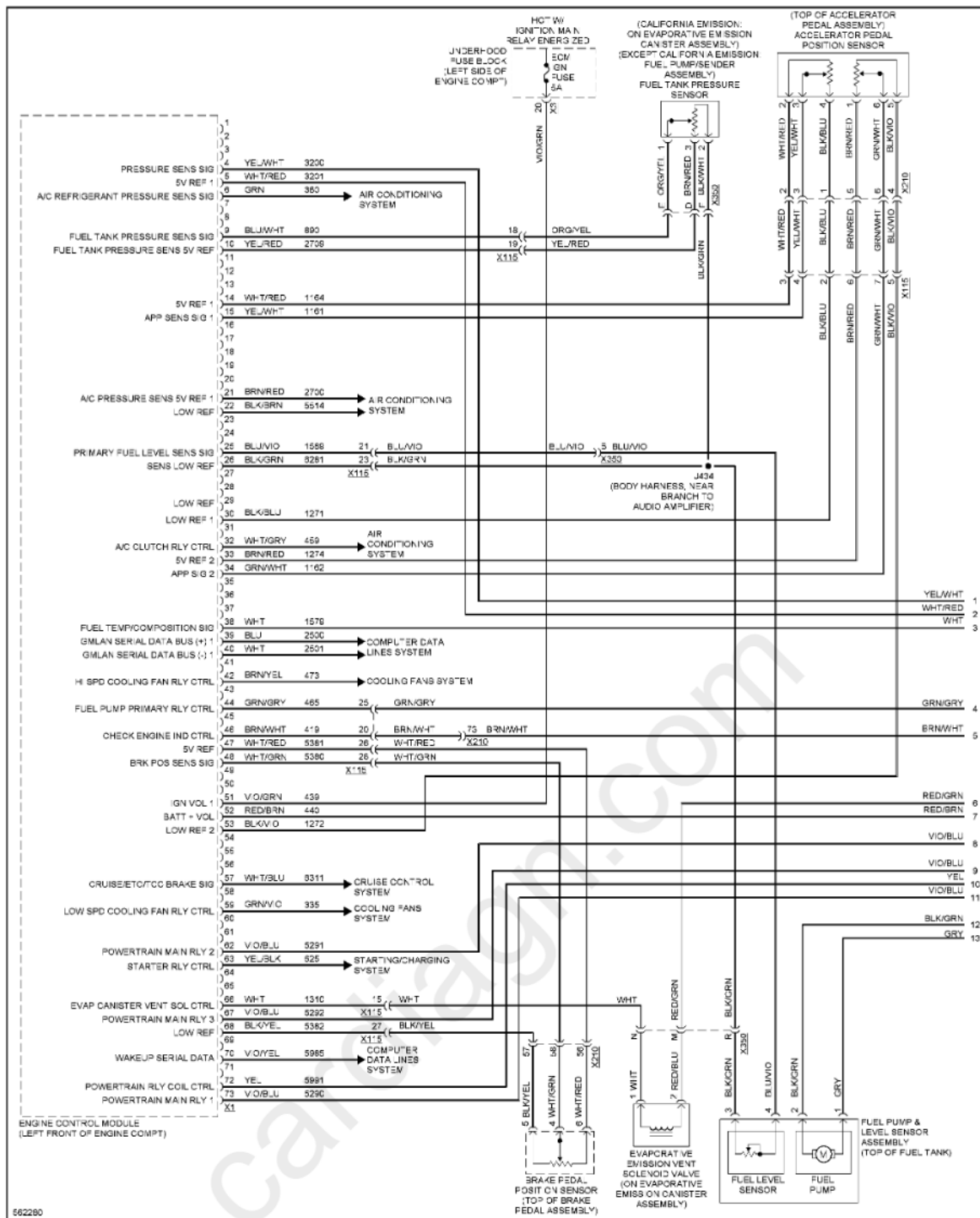
Fig. 41: 3.6L VIN 3, Engine Performance Circuit (1 of 6)
