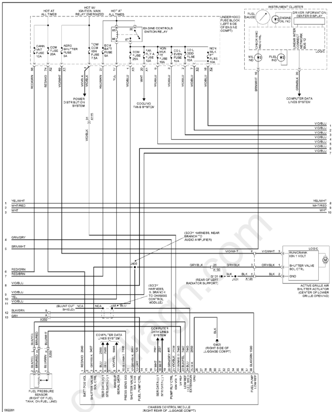
Fig. 42: 3.6L VIN 3, Engine Performance Circuit (2 of 6)
