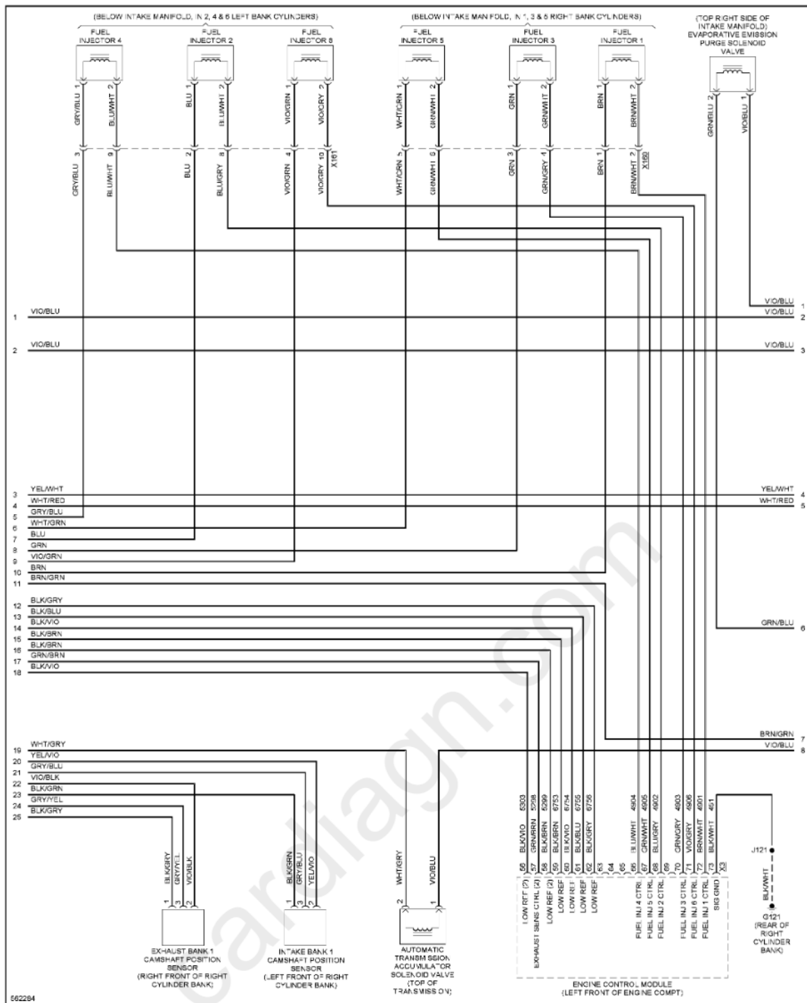
Fig. 45: 3.6L VIN 3, Engine Performance Circuit (5 of 6)
