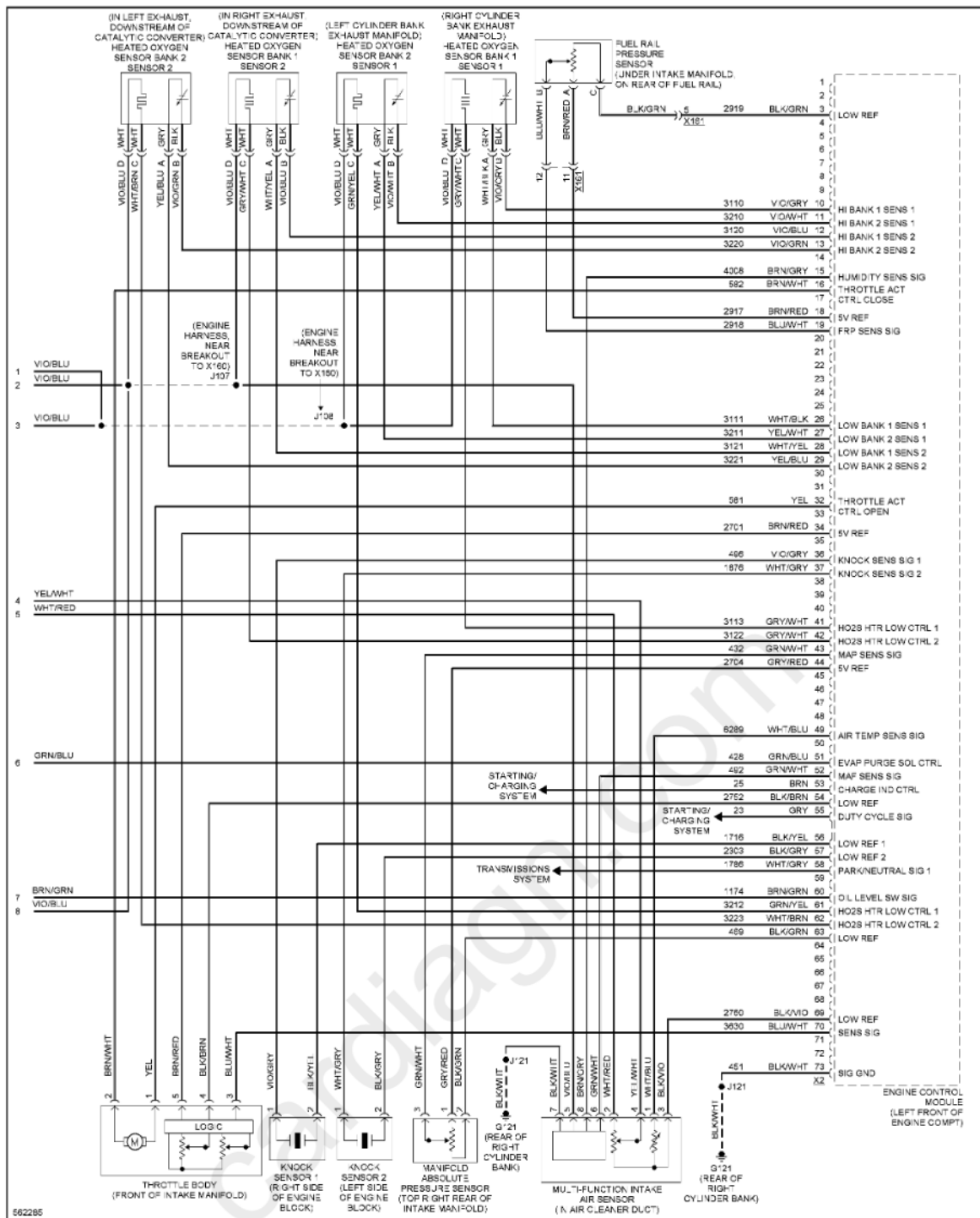
Fig. 46: 3.6L VIN 3, Engine Performance Circuit (6 of 6)
