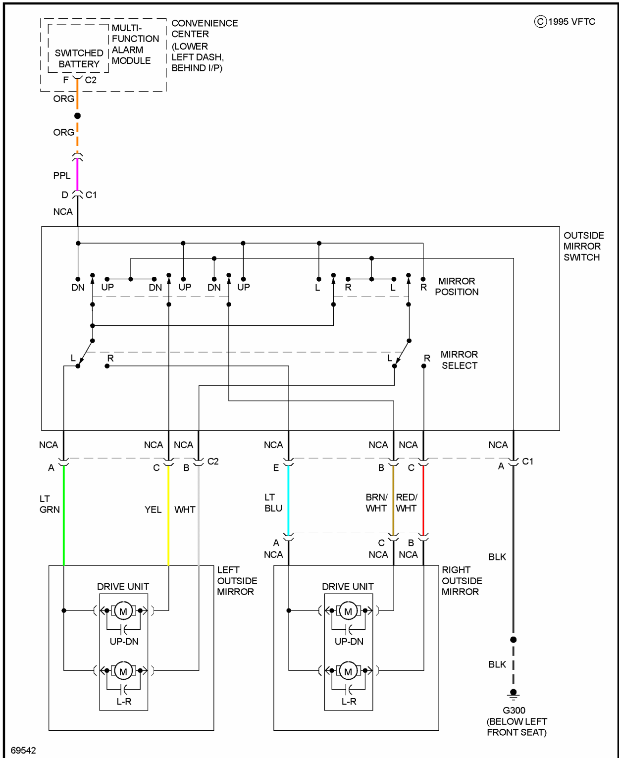
Fig. 33: Power Mirror Circuit
