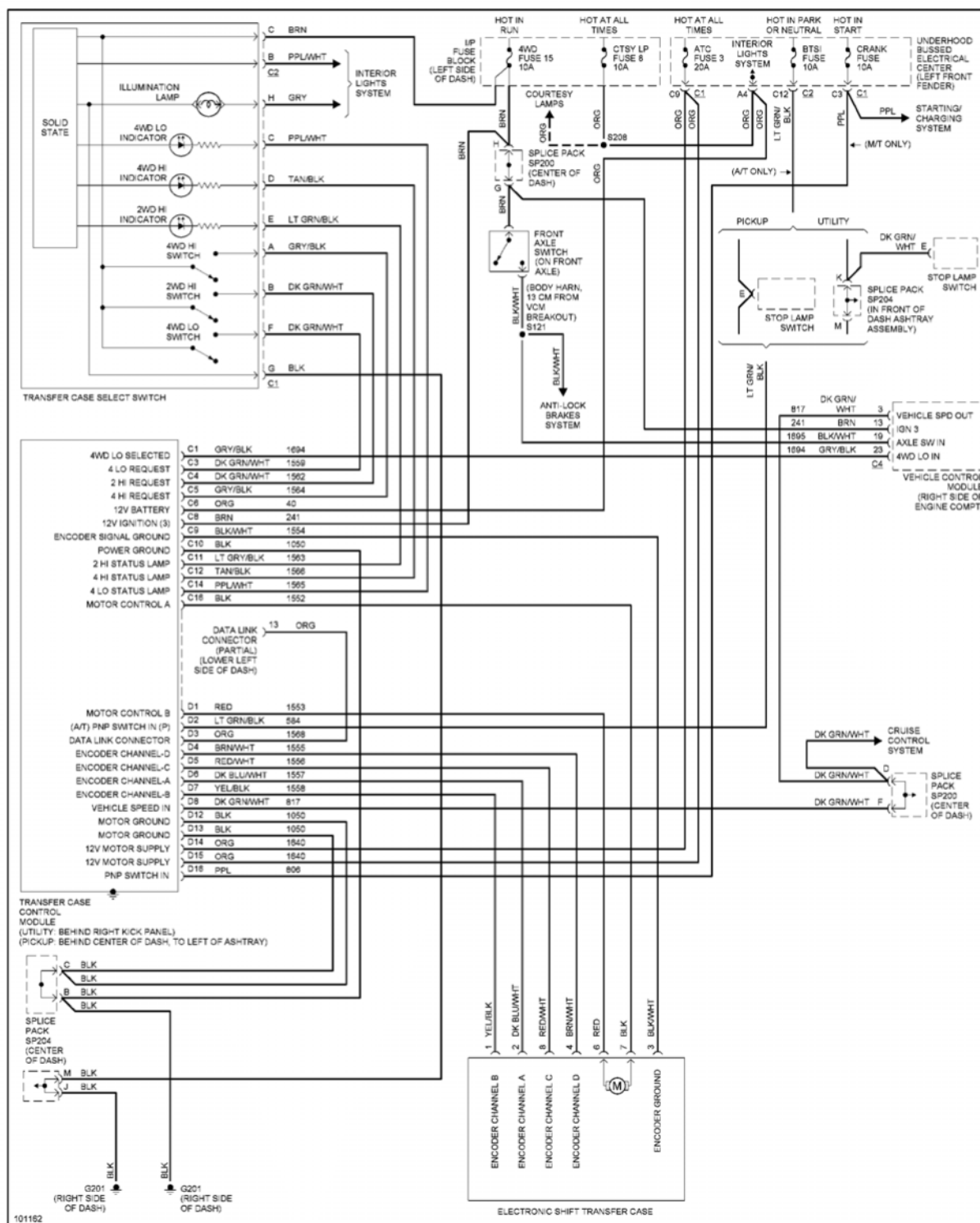
Fig. 50: Electronic Transfer Case Circuit
