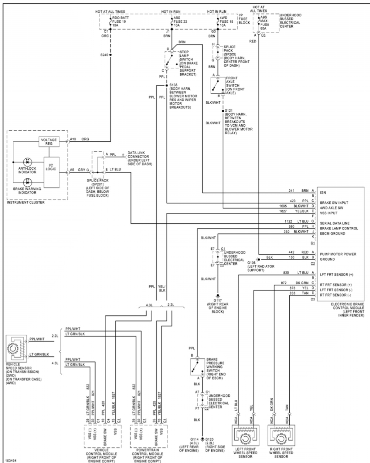
Fig. 5: Anti-lock Brake Circuits
