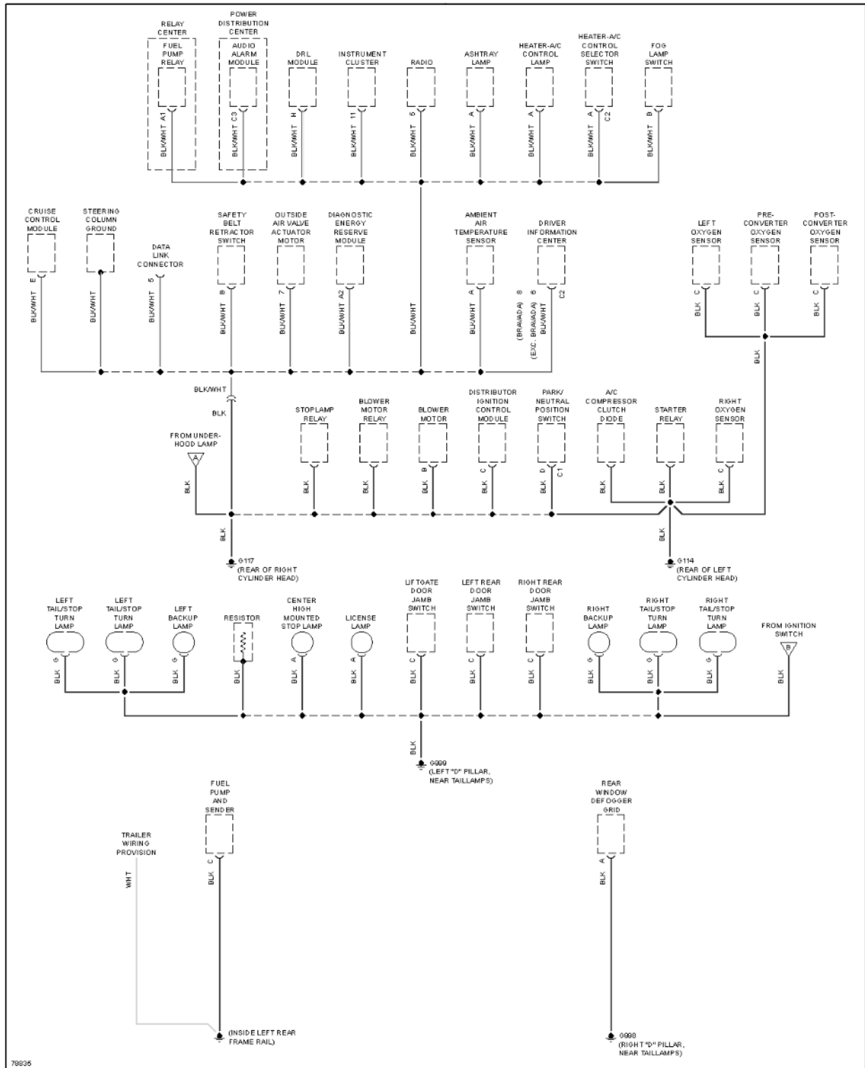
Fig. 13: Ground Distribution Circuit (2 of 2)
