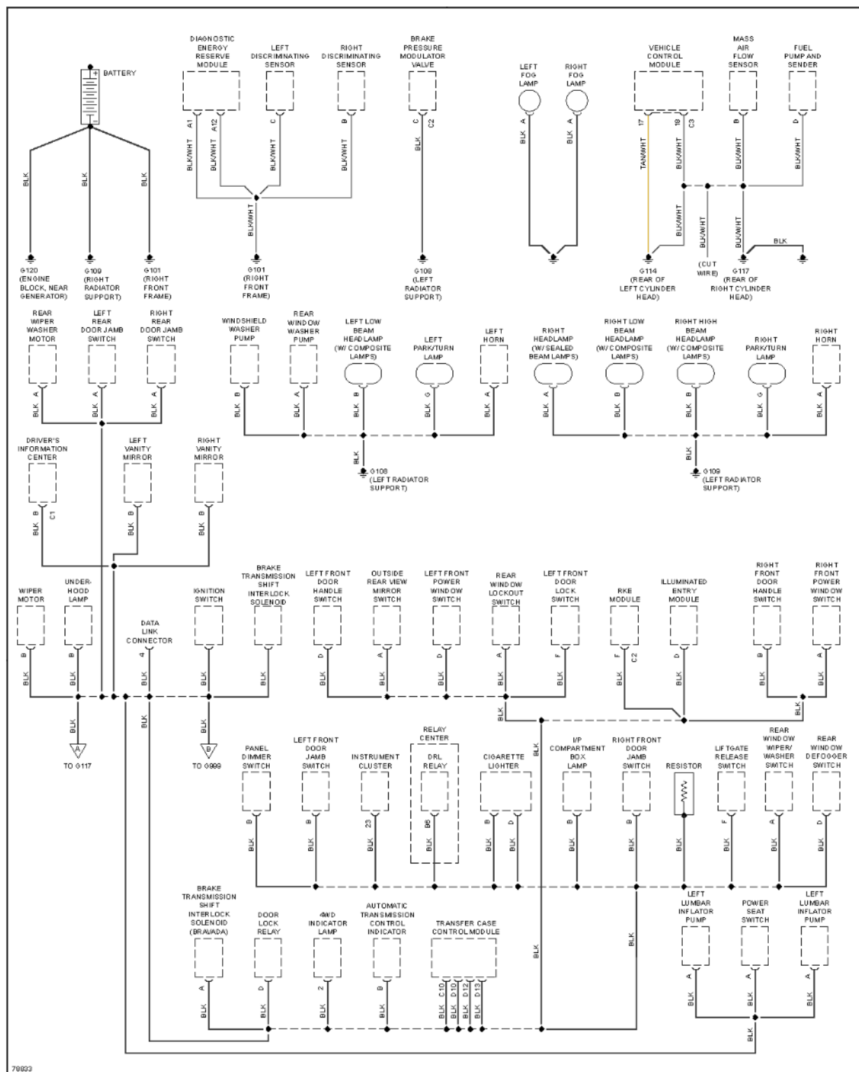
Fig. 12: Ground Distribution Circuit (1 of 2)
