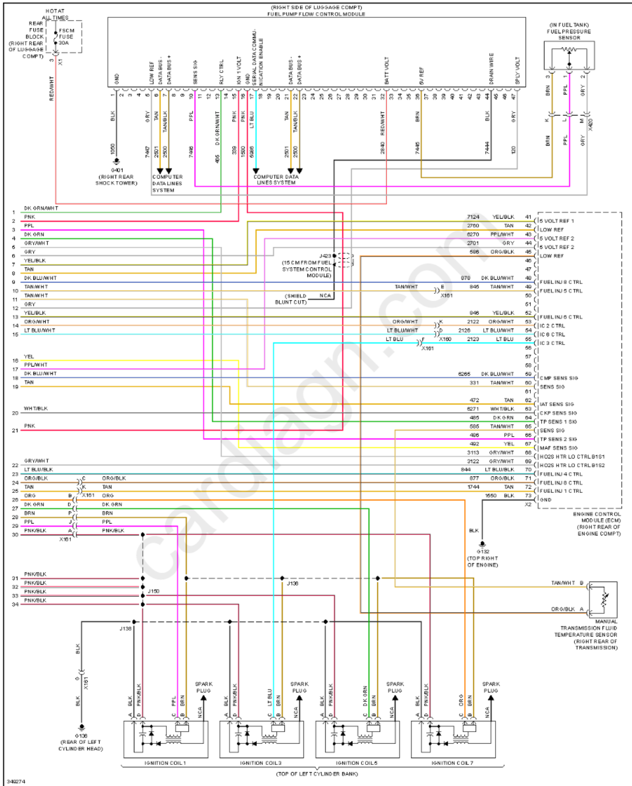
Fig. 41: 6.2L VIN P, Engine Performance Circuit (6 of 6)
