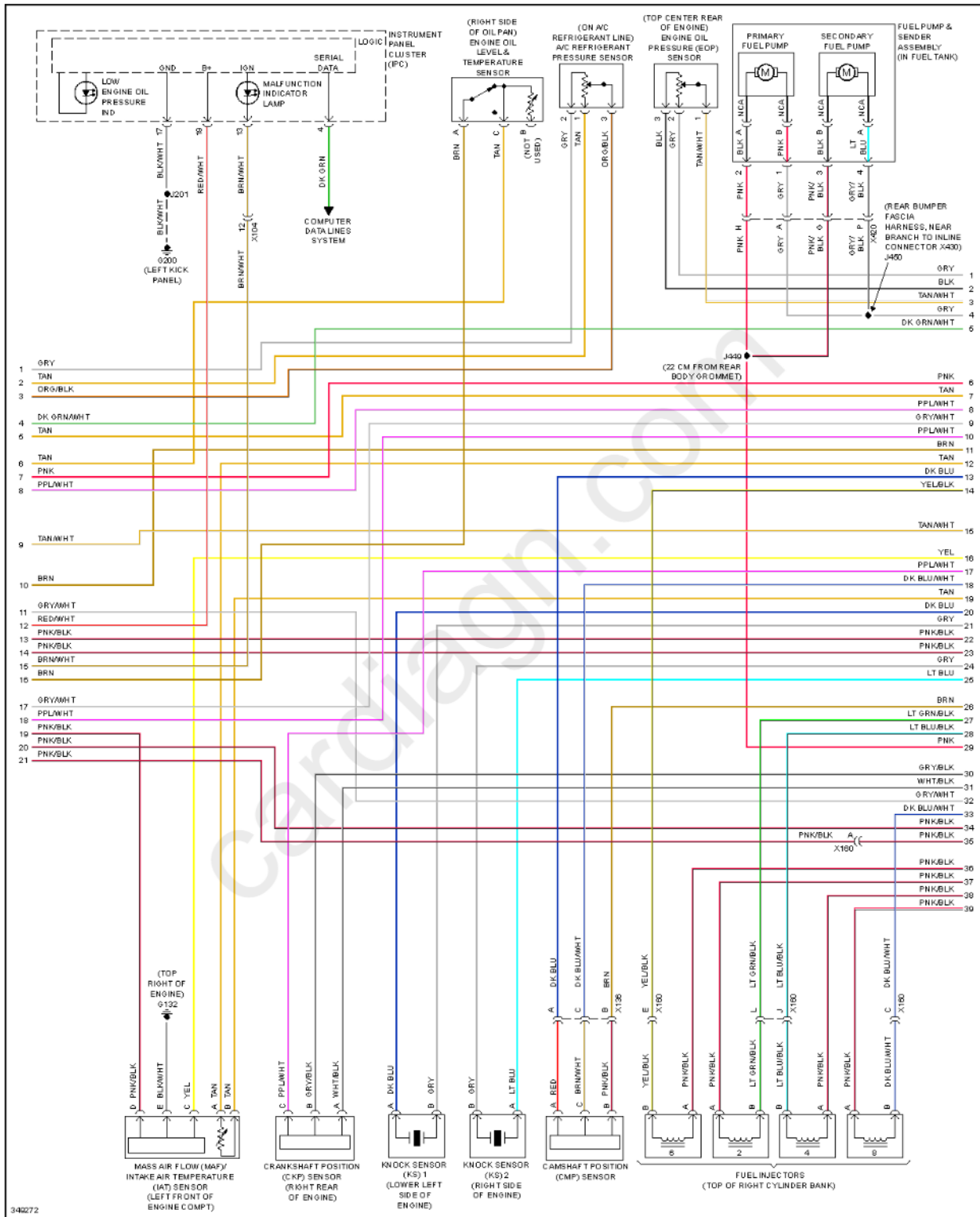
Fig. 39: 6.2L VIN P, Engine Performance Circuit (4 of 6)
