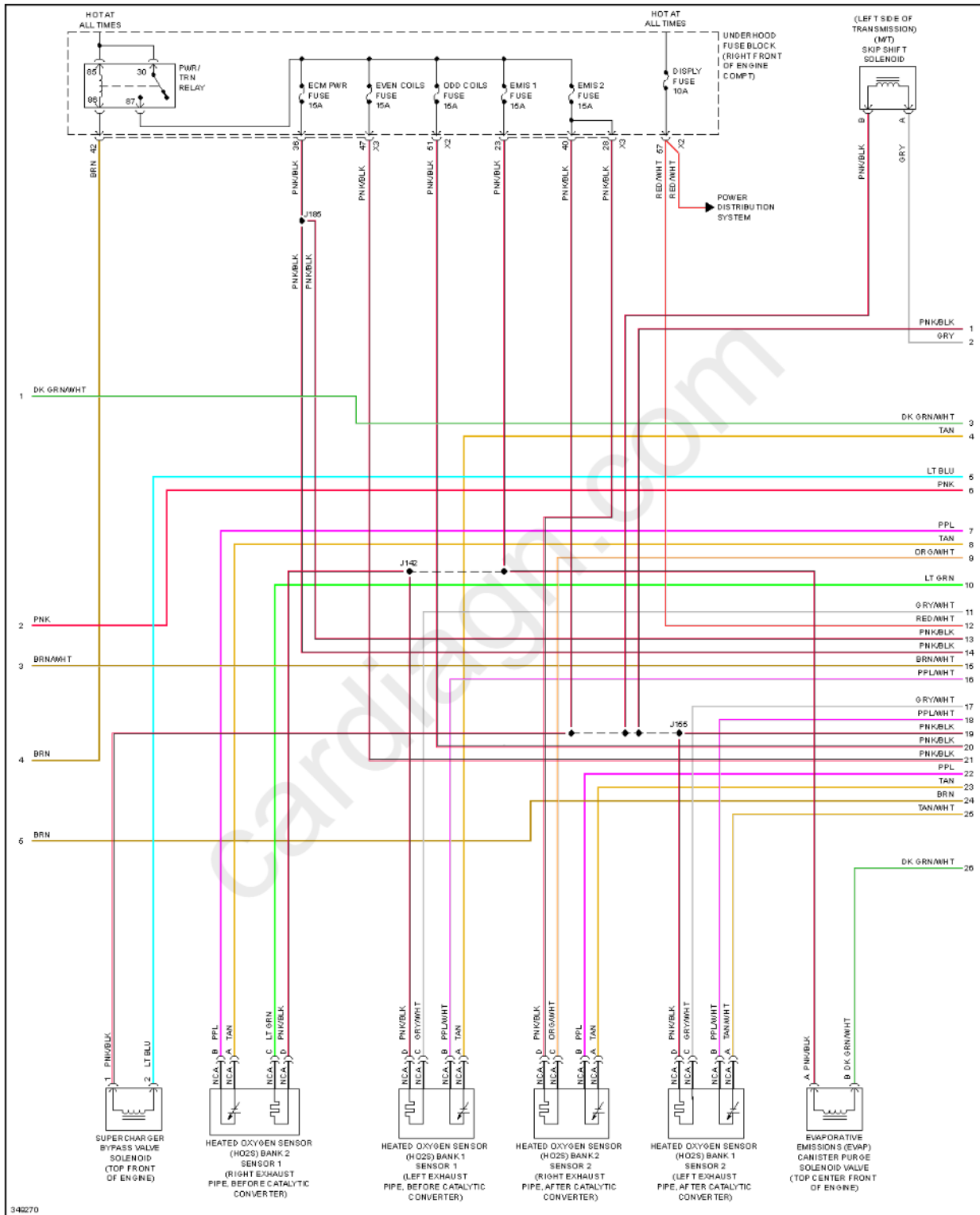
Fig. 37: 6.2L VIN P, Engine Performance Circuit (2 of 6)
