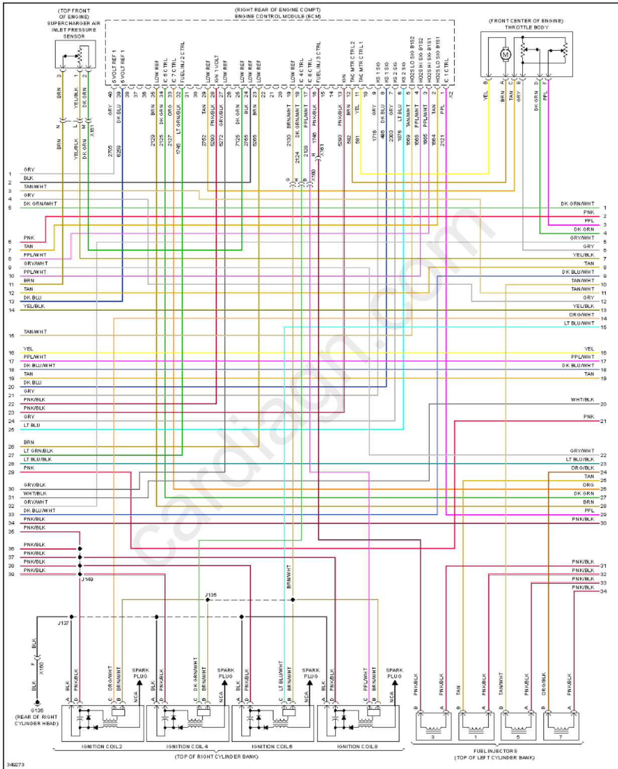
Fig. 40: 6.2L VIN P, Engine Performance Circuit (5 of 6)
