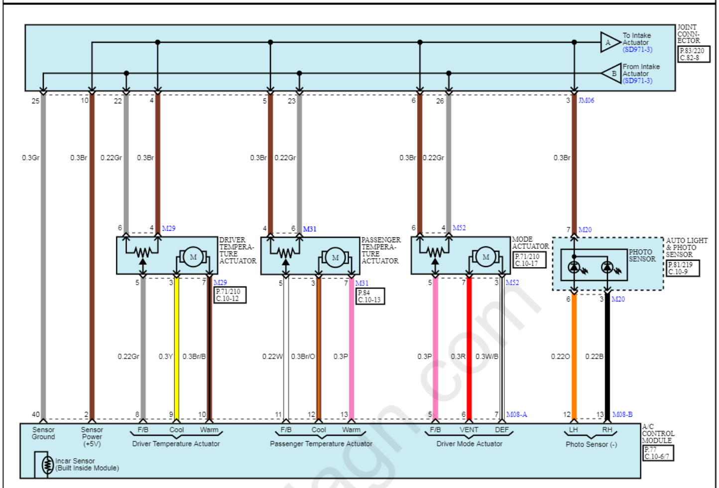
A/C Control System (Auto) (2)
