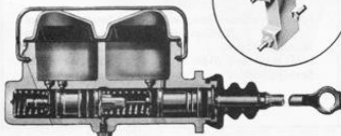
DUAL MASTER CYLINDER
