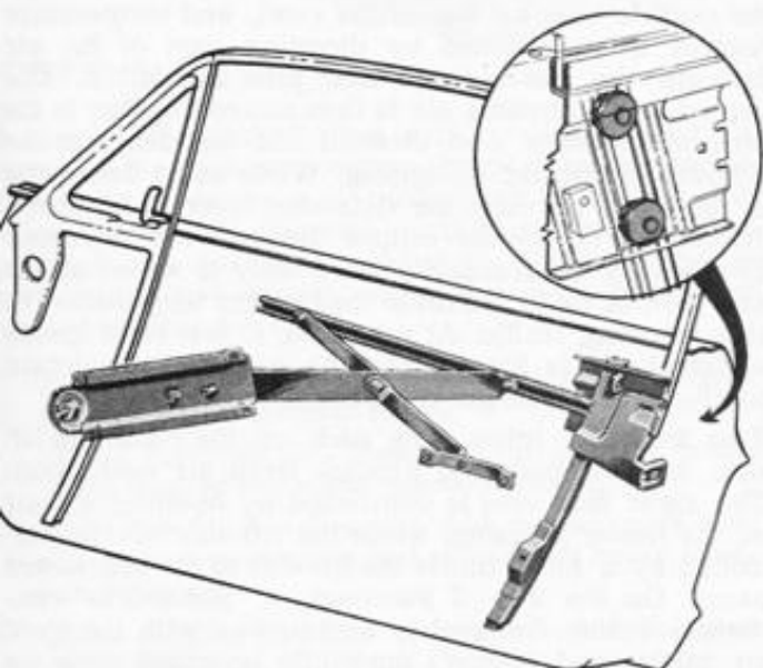
WINDOW REGULATOR AND GUIDE
