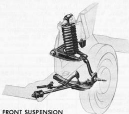
FRONT SUSPENSION
