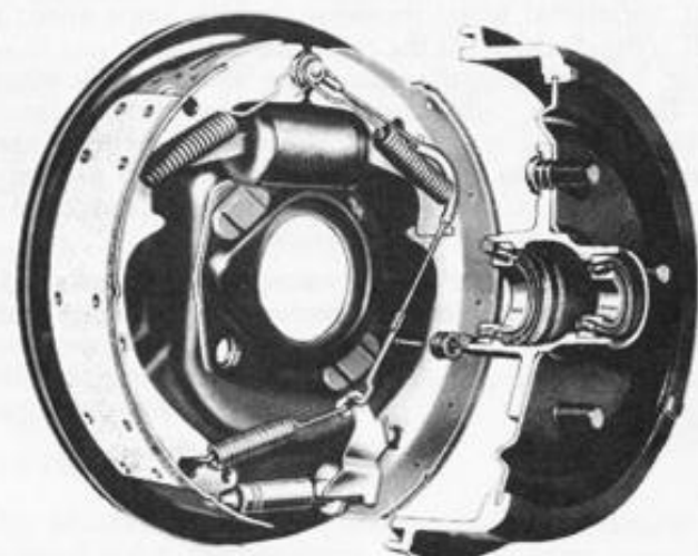
STANDARD DRUM BRAKES
