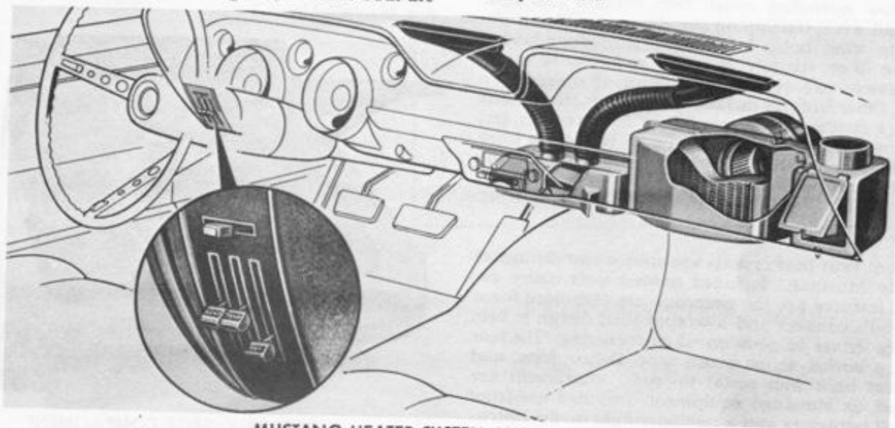
MUSTANG HEATER SYSTEM AND CONTROLS
