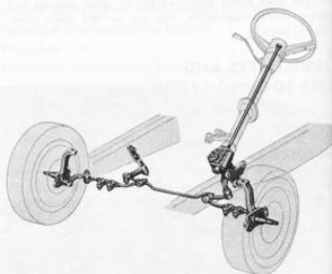
MUSTANG MANUAL STEERING
