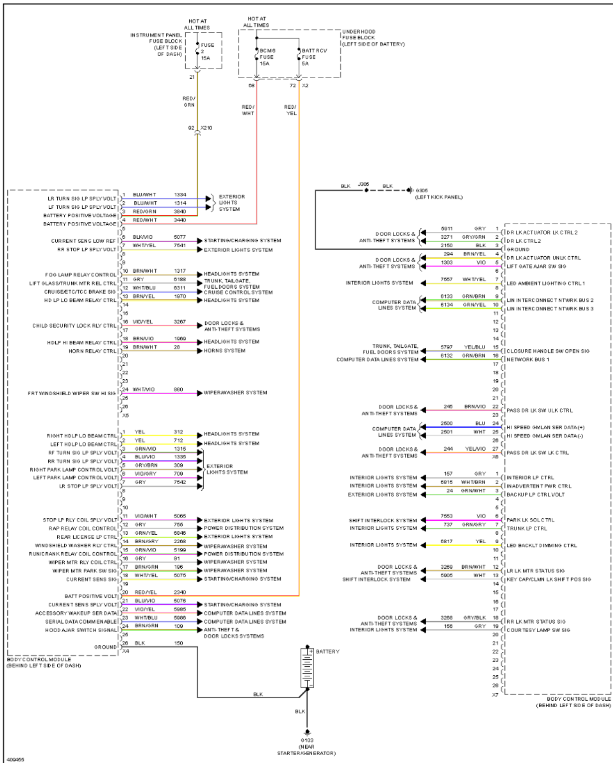
Fig. 19: Body Control Modules Circuit (2 of 2)
