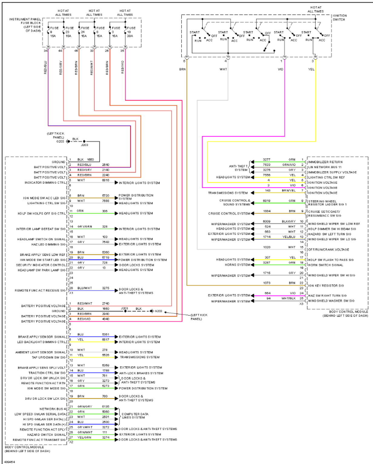
Fig. 18: Body Control Modules Circuit (1 of 2)
