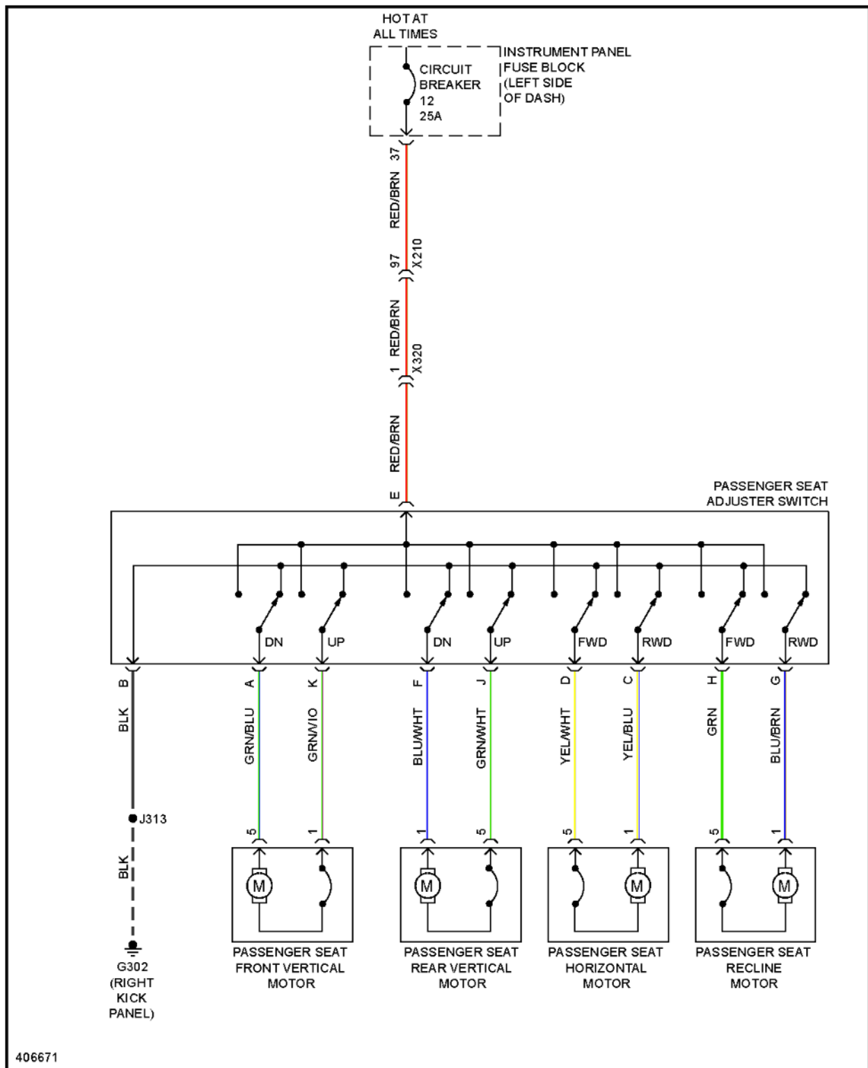
Fig. 108: Passenger Power Seat Circuit, 8-Way Power Seat
