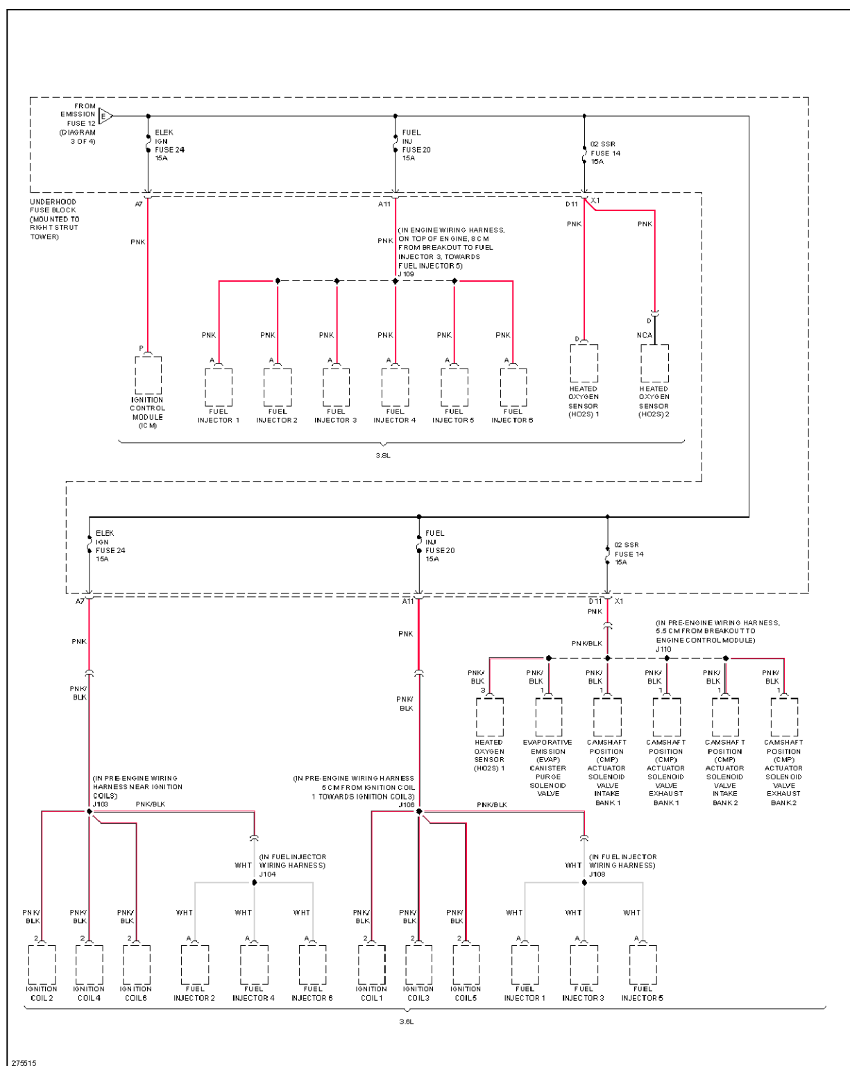
Fig. 63: 3.8L VIN 2, Power Distribution Circuit (4 of 4)
