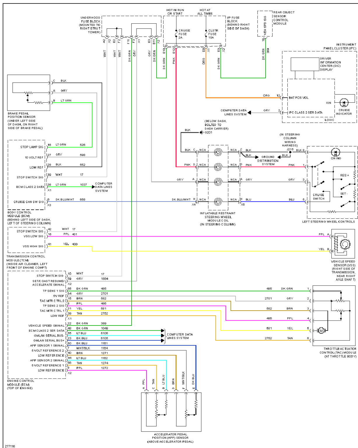
Fig. 19: 3.6L VIN 7, Cruise Control Circuit
