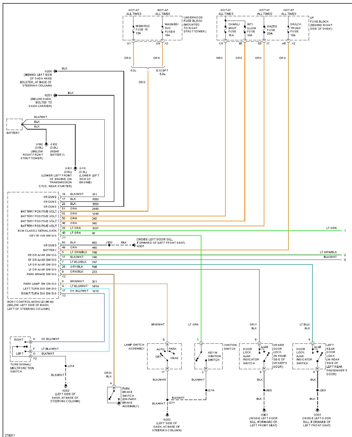
Fig. 93: Warning Systems Circuit (1 of 2)
