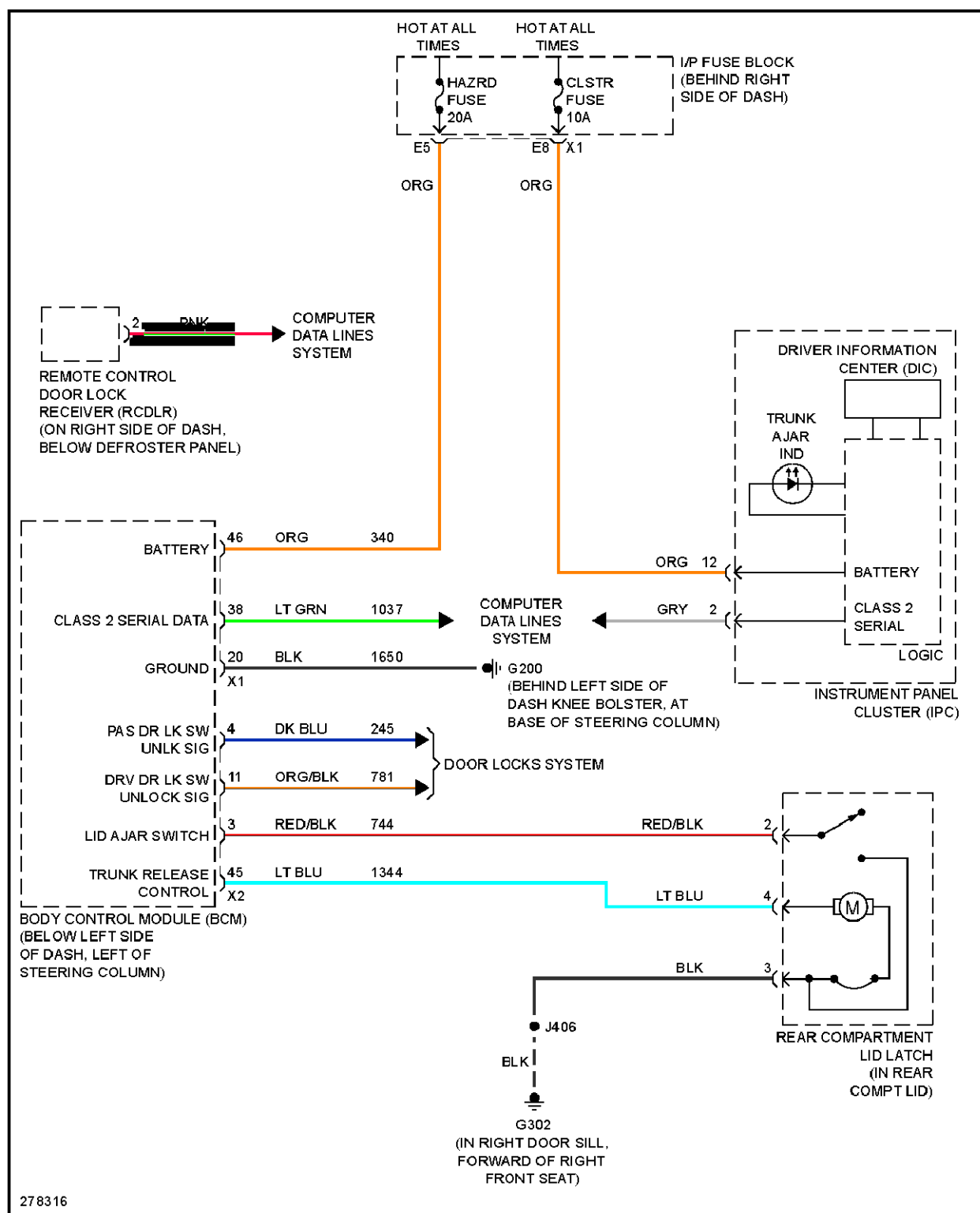
Fig. 92: Trunk Release Circuit
