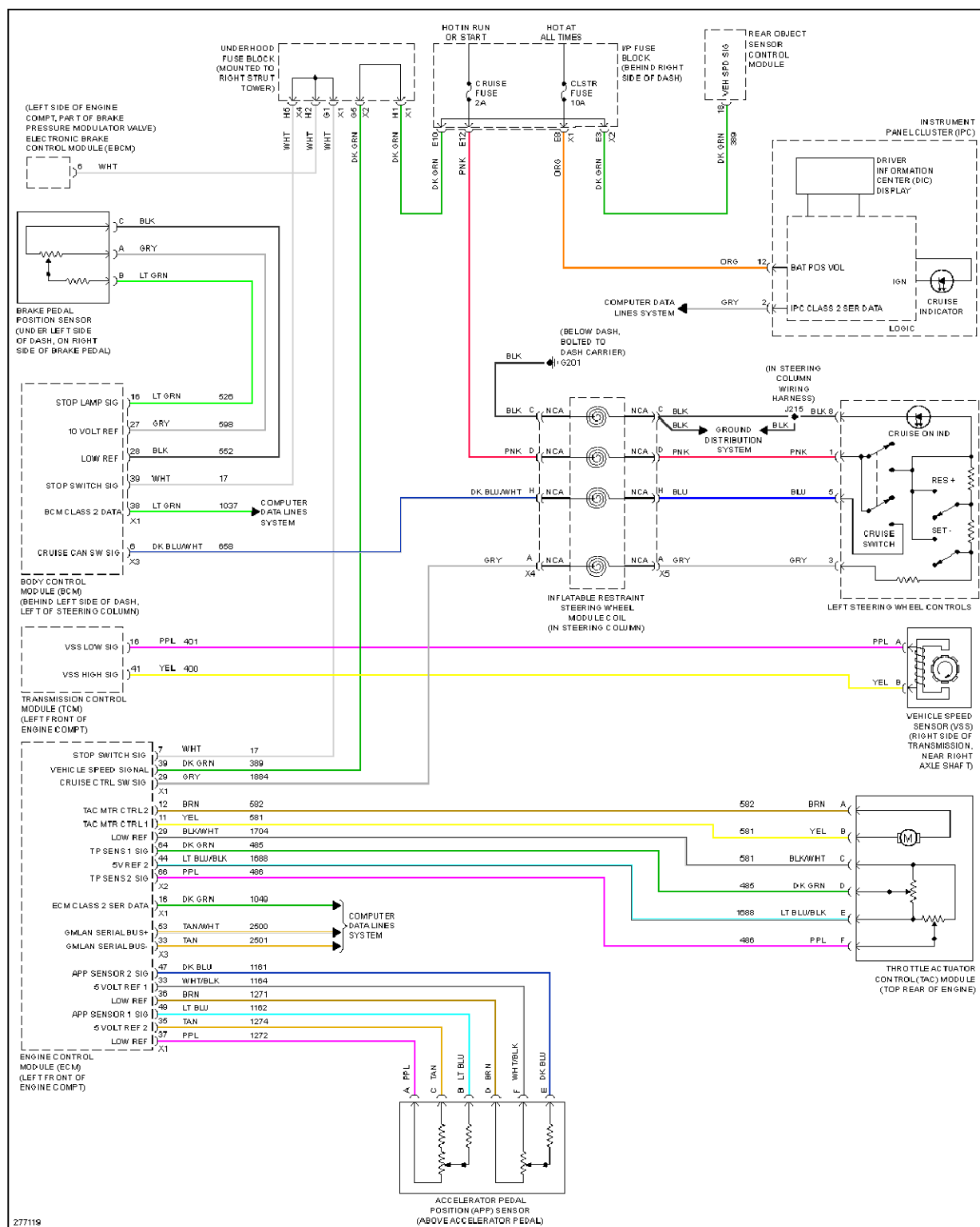
Fig. 21: 5.3L VIN C, Cruise Control Circuit
