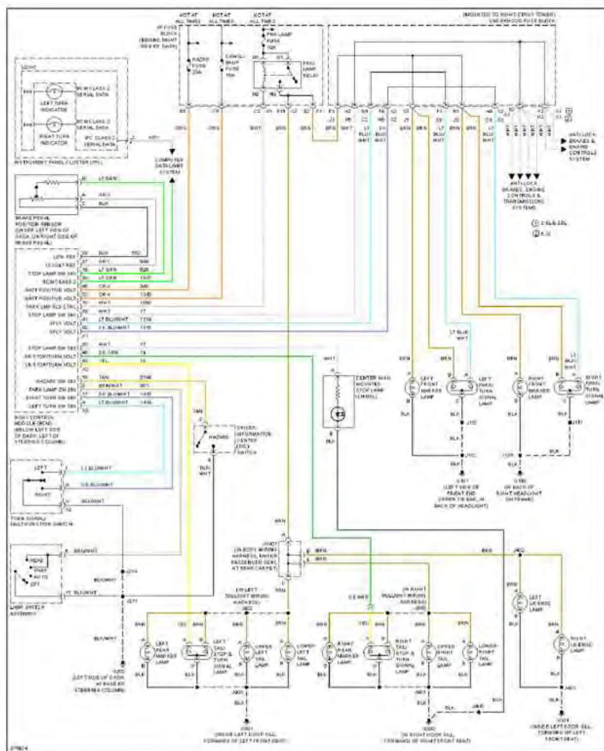
Fig. 38: Exterior Lamps Circuit
