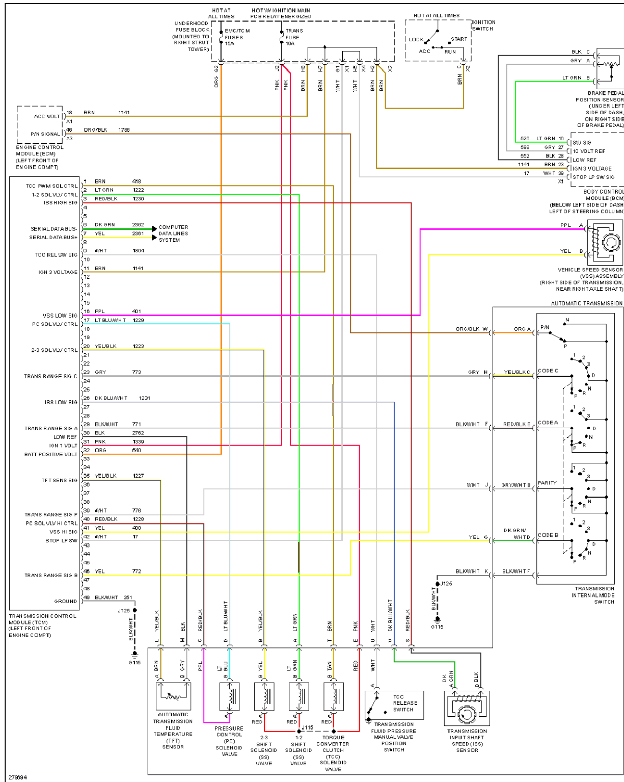
Fig. 91: 5.3L VIN C, Transmission Circuit
