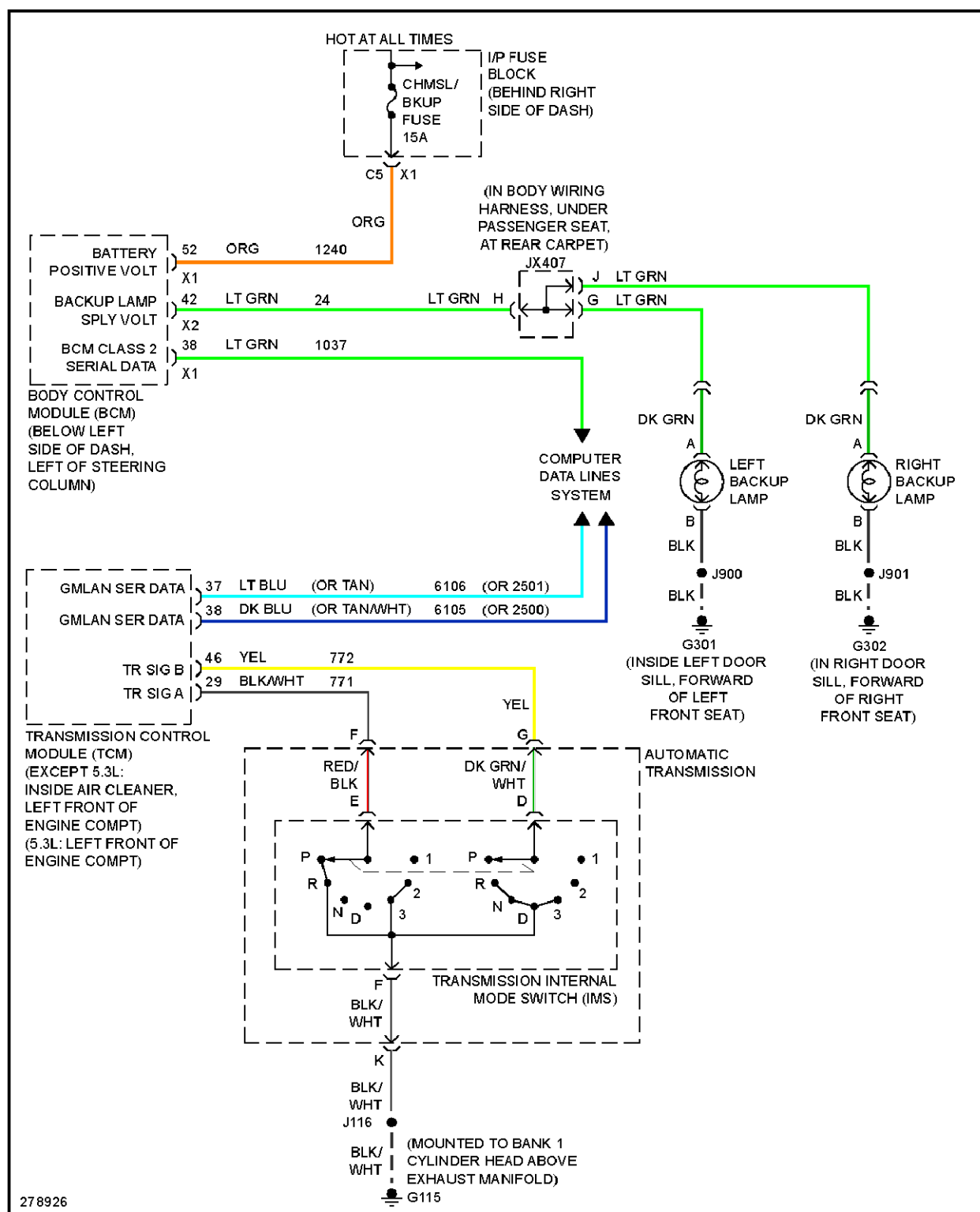
Fig. 39: 3.6L VIN 7, Backup Lamps Circuit
