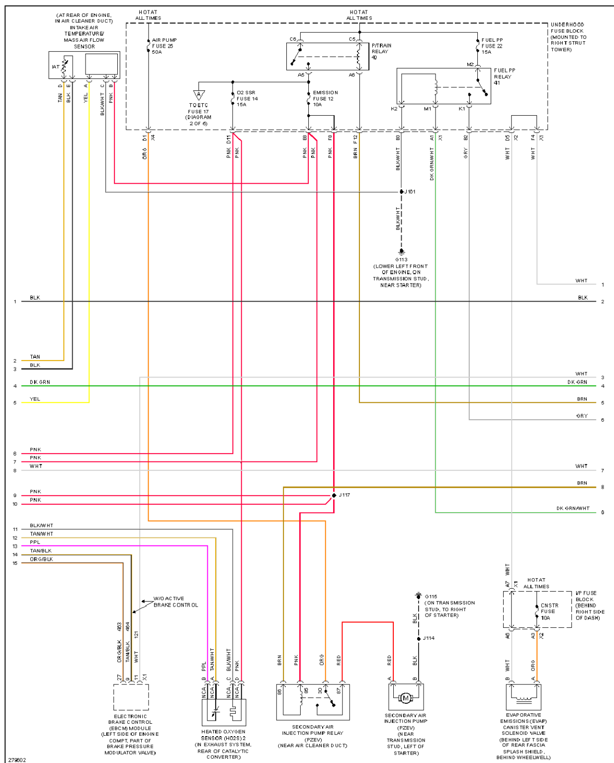
Fig. 31: 3.8L VIN 2, Engine Performance Circuit (4 of 5)
