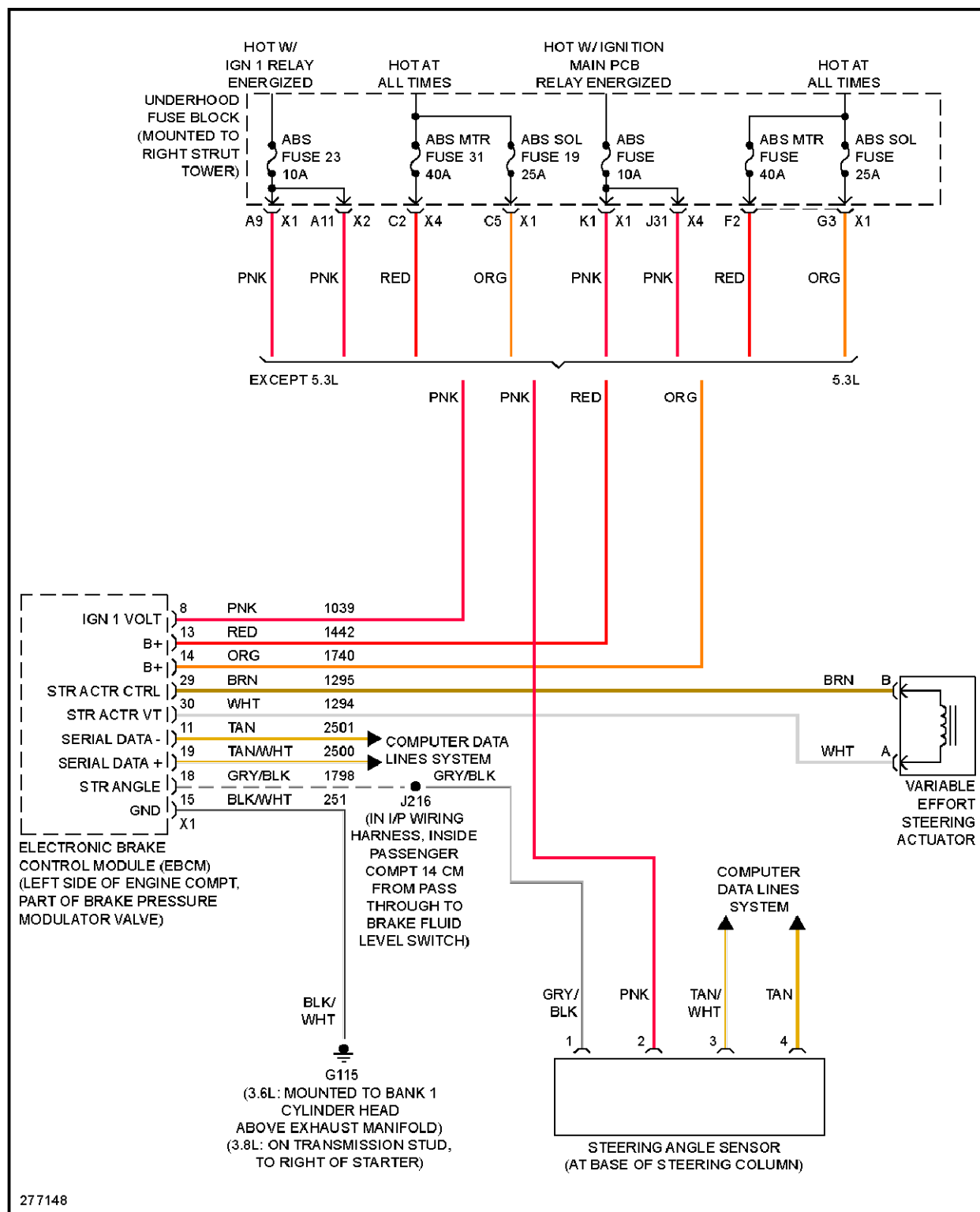
Fig. 23: Electronic Power Steering Circuit
