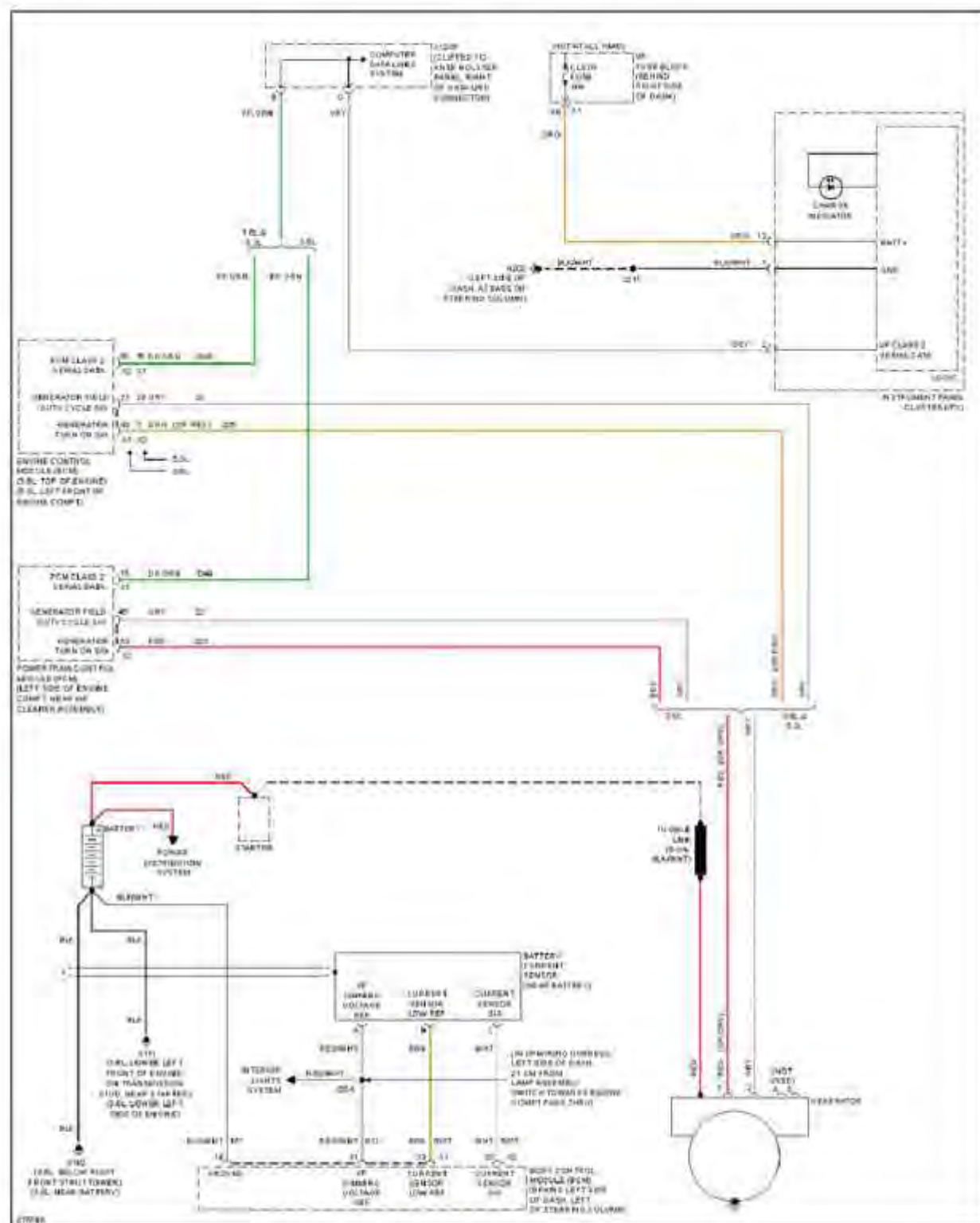
Fig. 83: Charging Circuit
