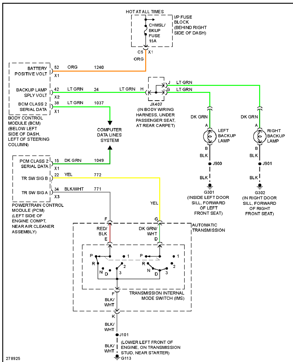
Fig. 40: 3.8L VIN 2, Backup Lamps Circuit
