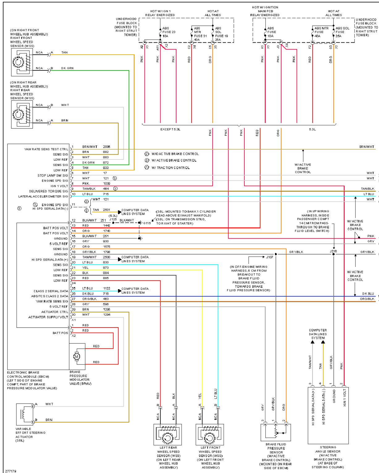
Fig. 10: Anti-lock Brakes Circuit (1 of 2)
