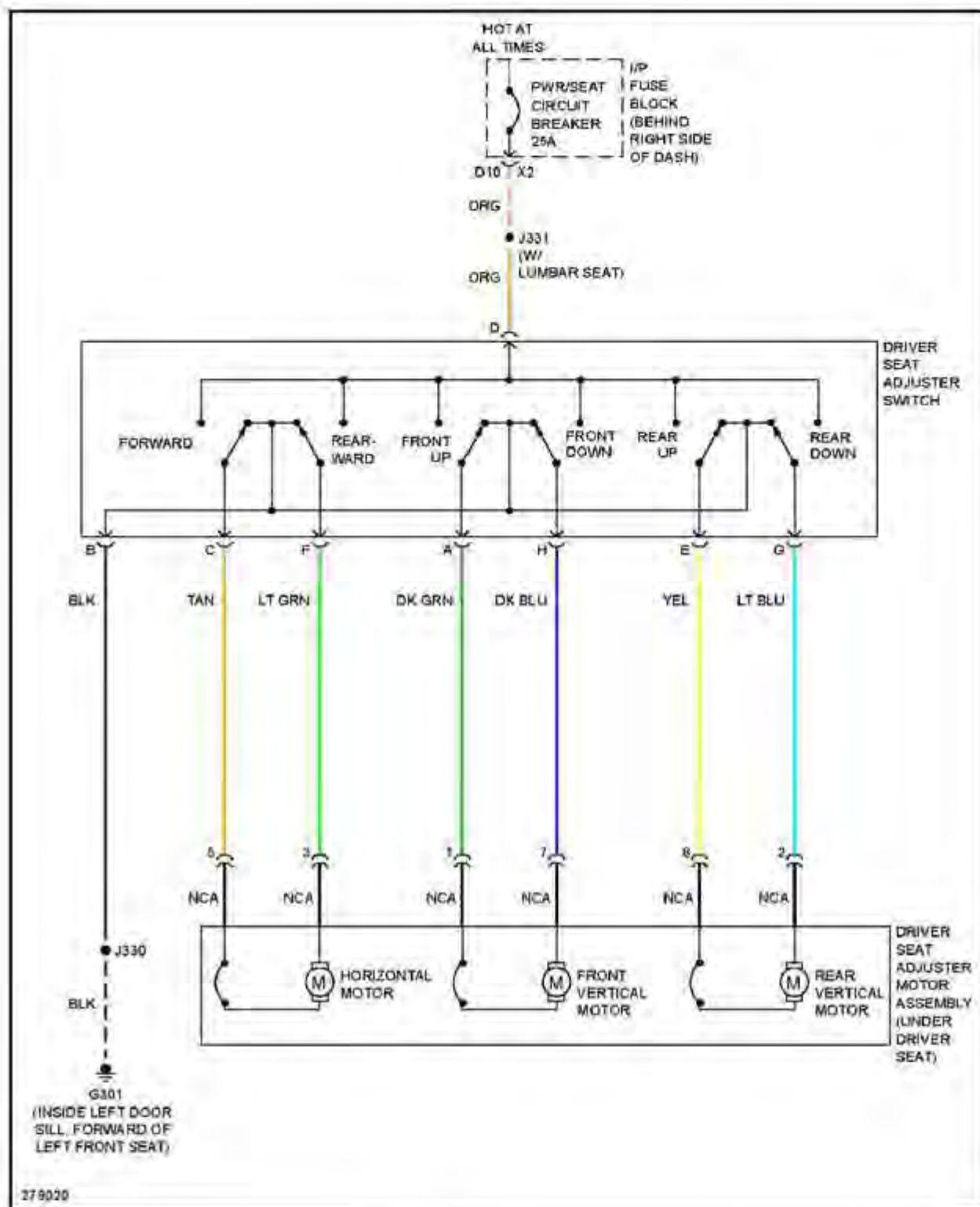
Fig. 70: Driver Power Seat Circuit
