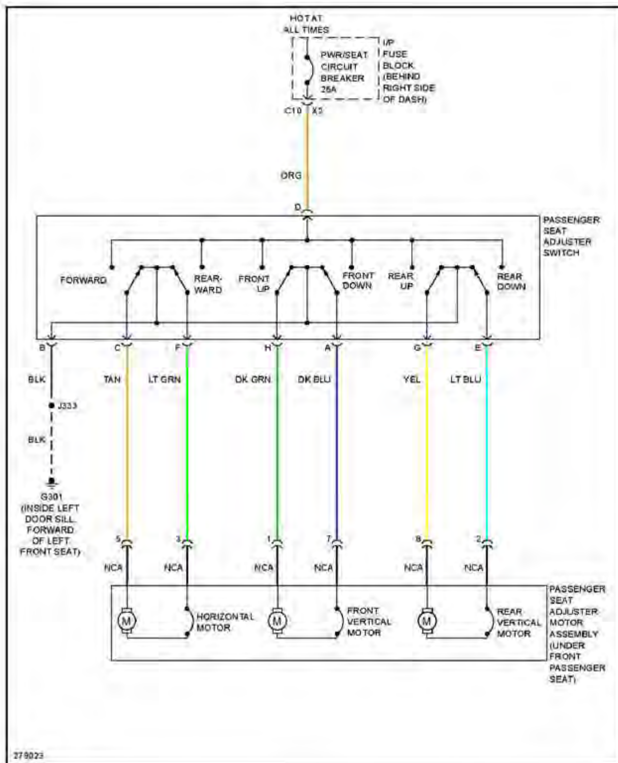
Fig. 73: Passenger's Power Seat Circuit
