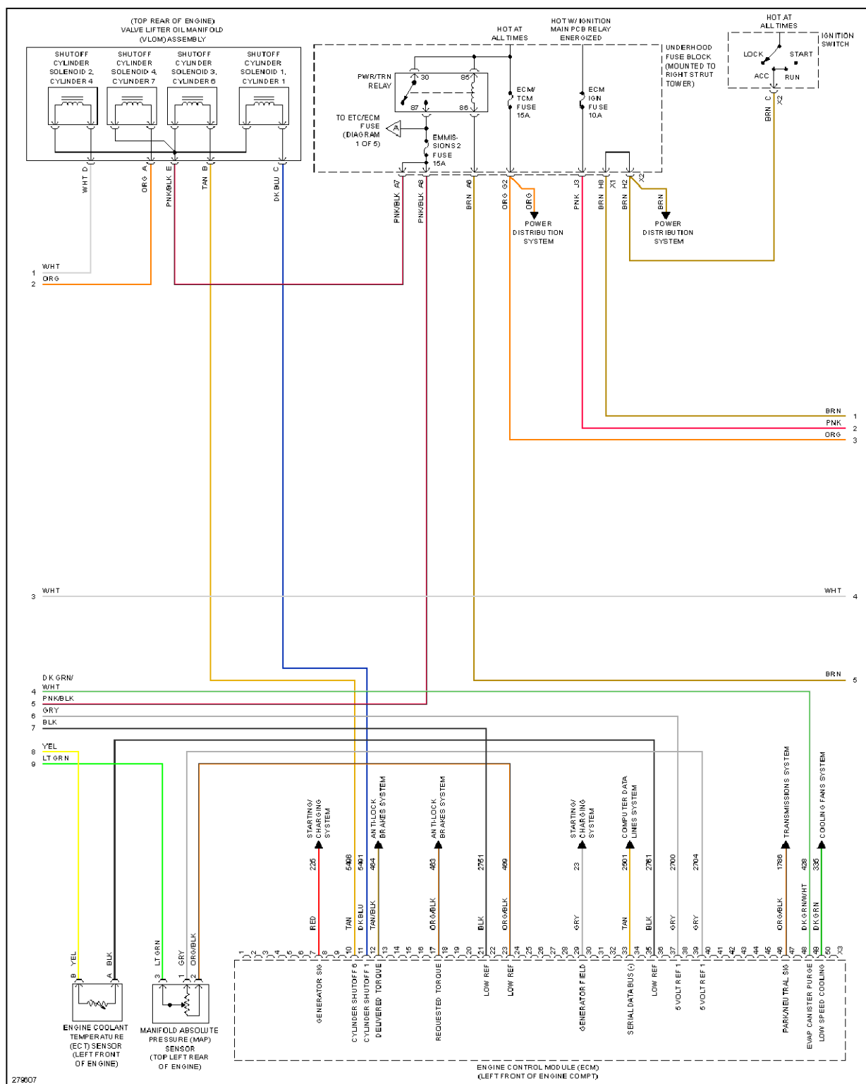
Fig. 36: 5.3L VIN C, Engine Performance Circuit (4 of 5)
