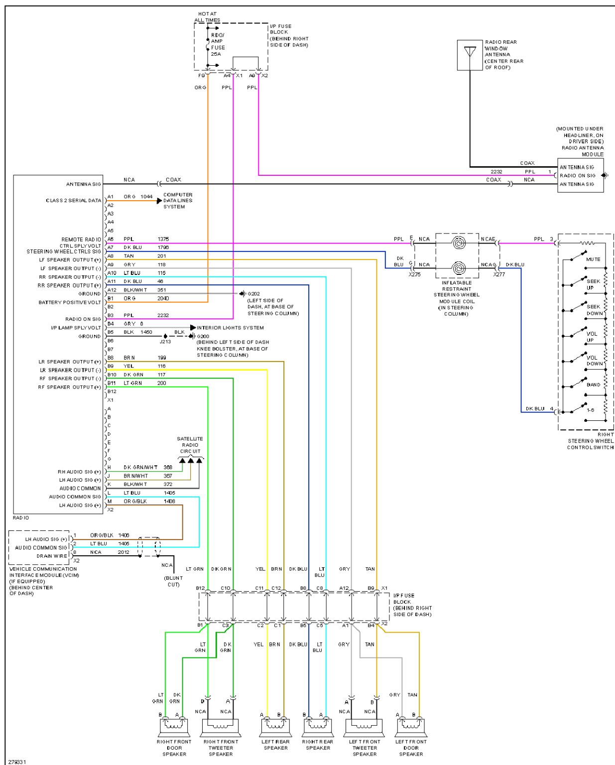
Fig. 77: Radio Circuit, W/O Amplifier
