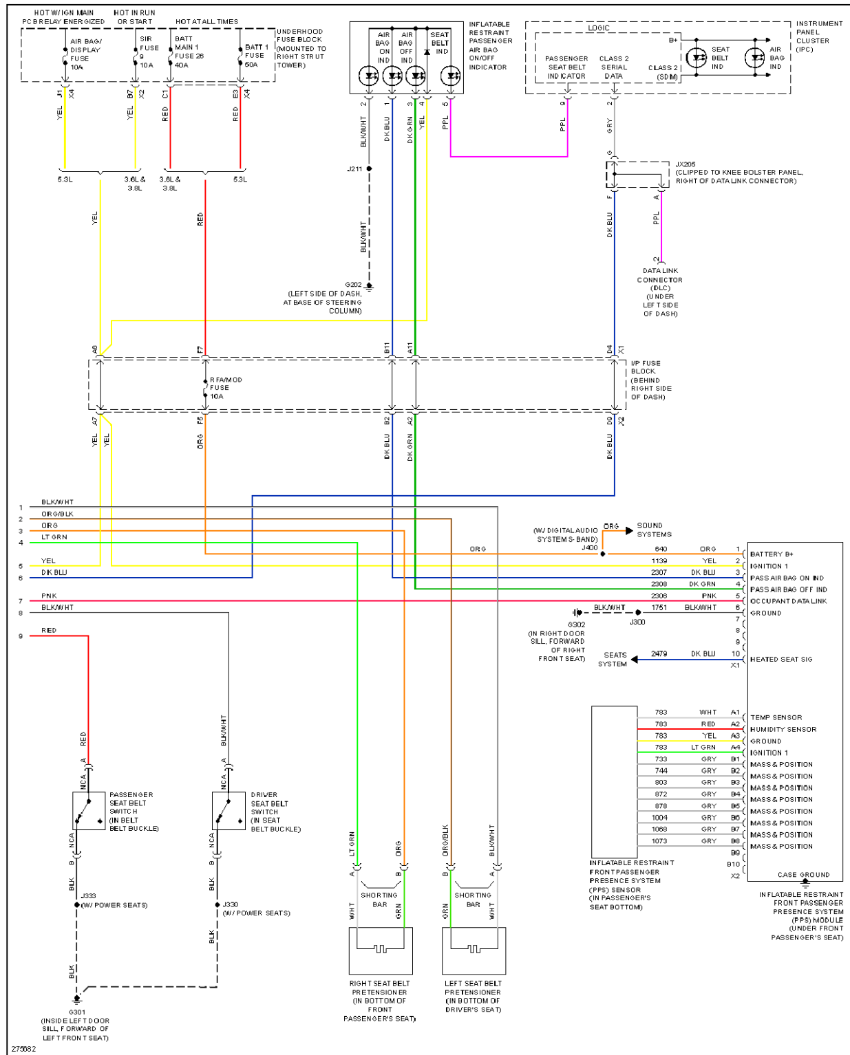
Fig. 88: Supplemental Restraints Circuit (2 of 2)
