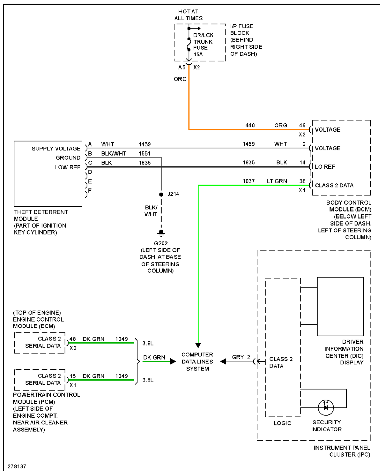
Fig. 13: Pass-Key Circuit
