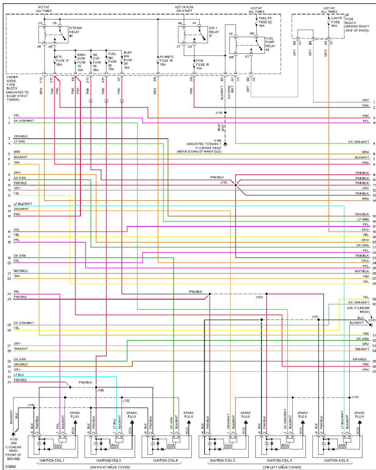
Fig. 25: 3.6L VIN 7, Engine Performance Circuit (2 of 4)
