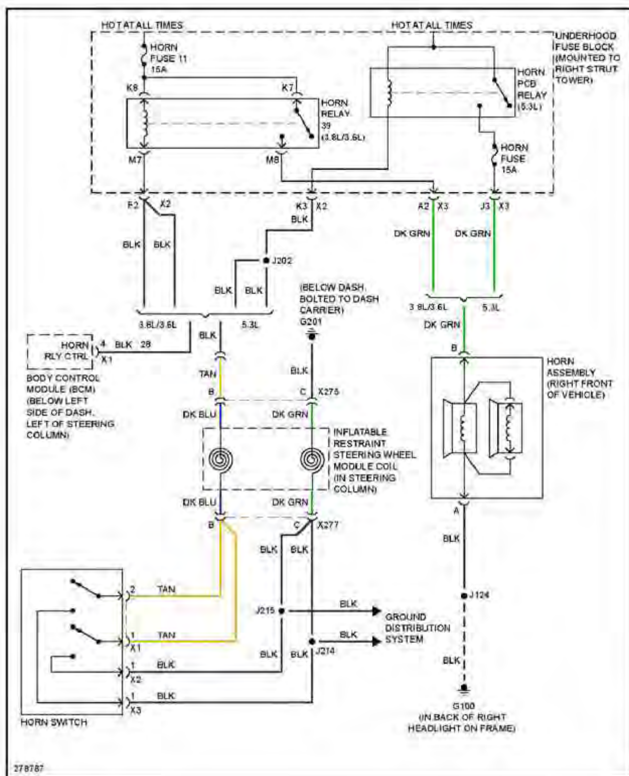
Fig. 48: Horn Circuit
