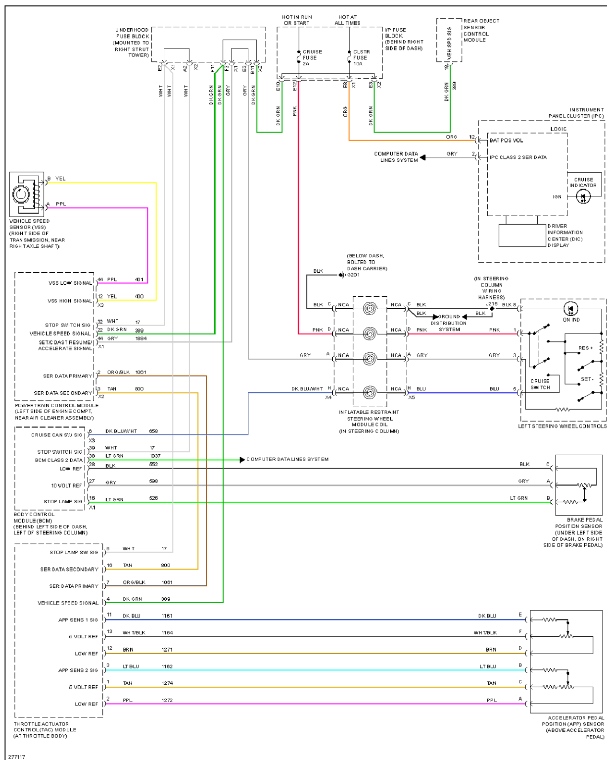
Fig. 20: 3.8L VIN 2, Cruise Control Circuit
