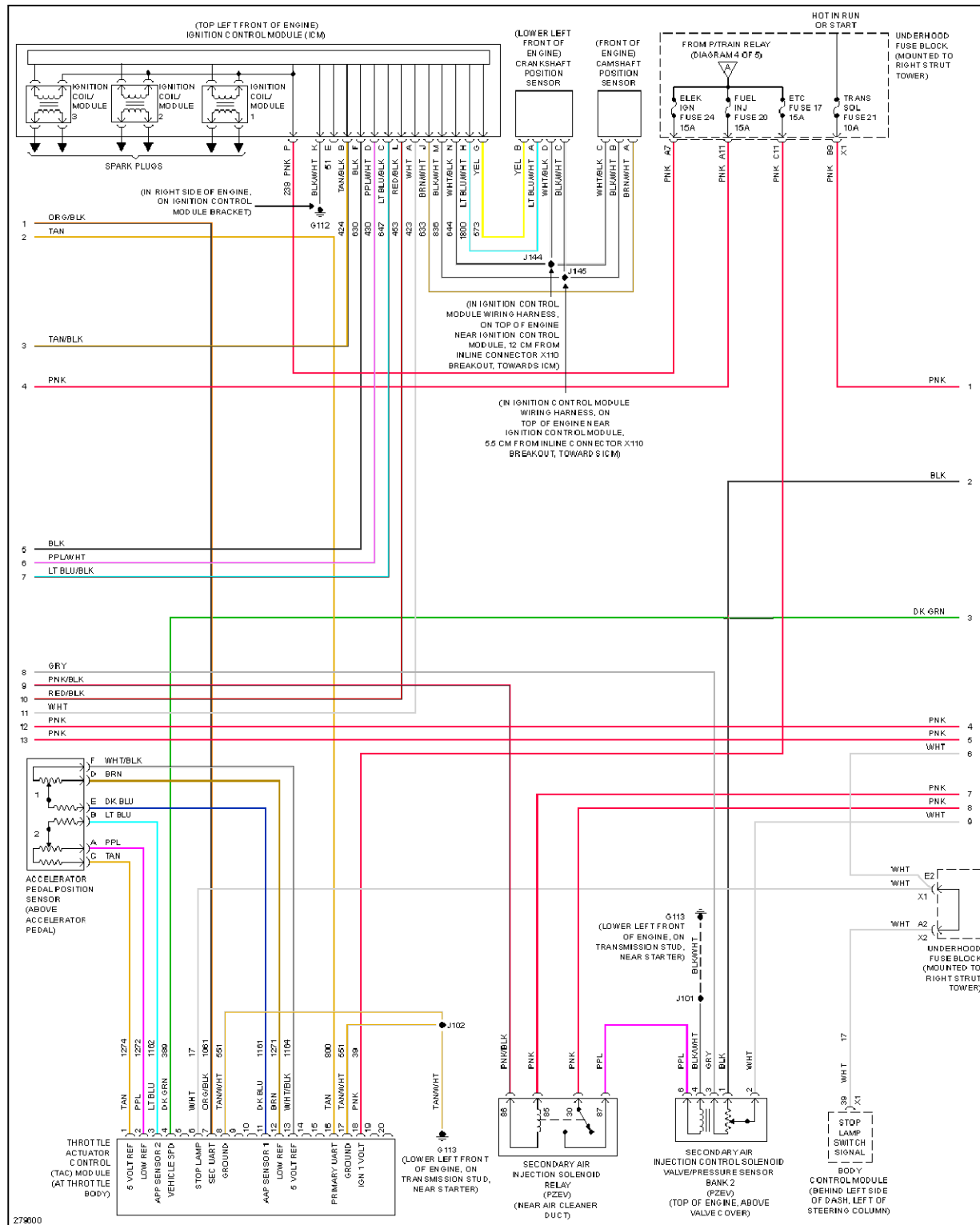
Fig. 29: 3.8L VIN 2, Engine Performance Circuit (2 of 5)
