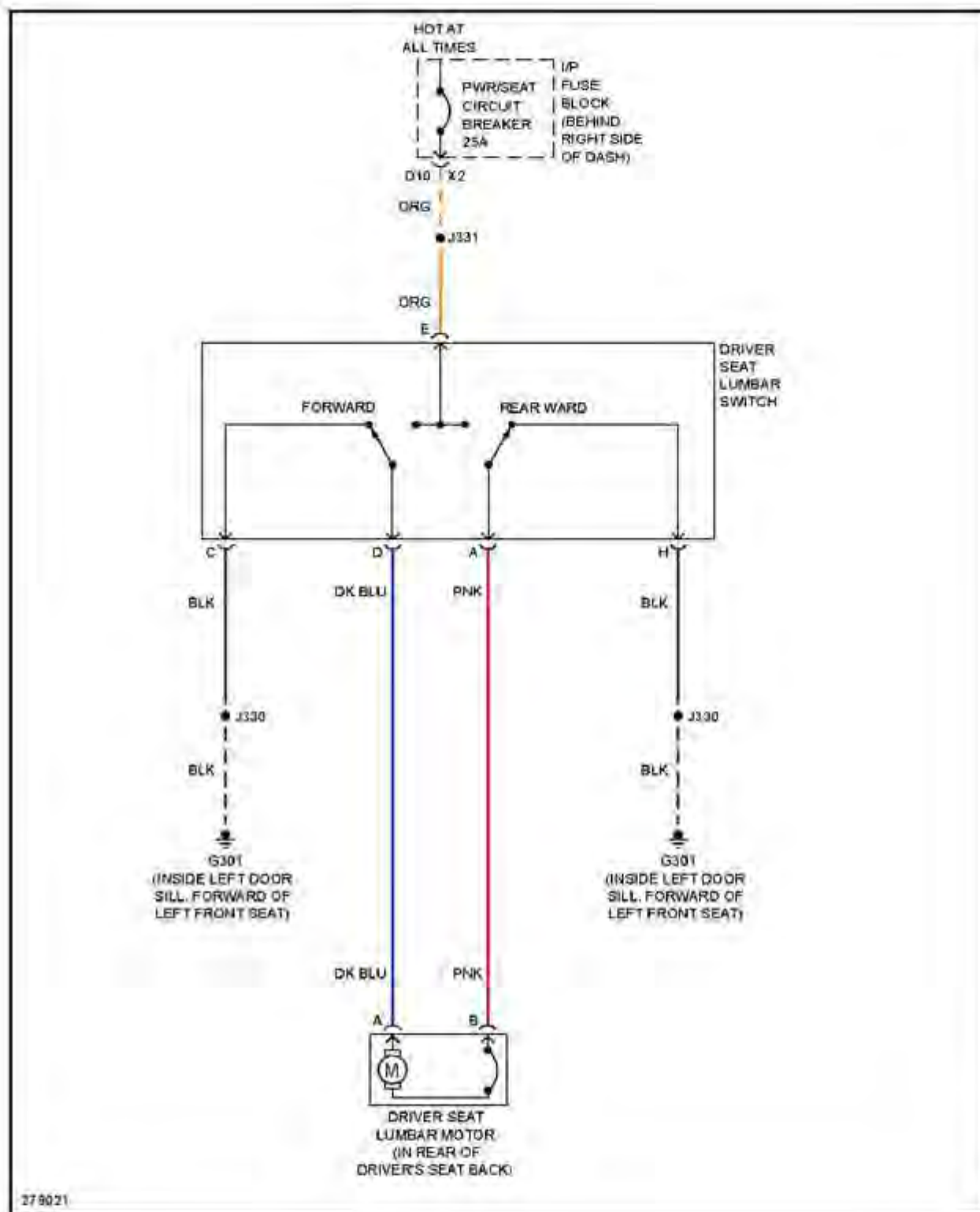
Fig. 71: Driver's Lumbar Circuit
