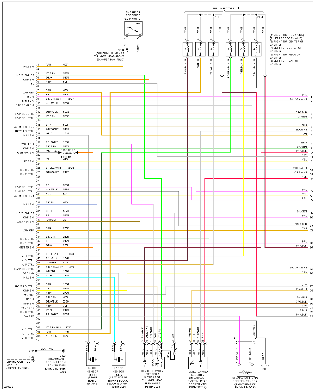
Fig. 24: 3.6L VIN 7, Engine Performance Circuit (1 of 4)
