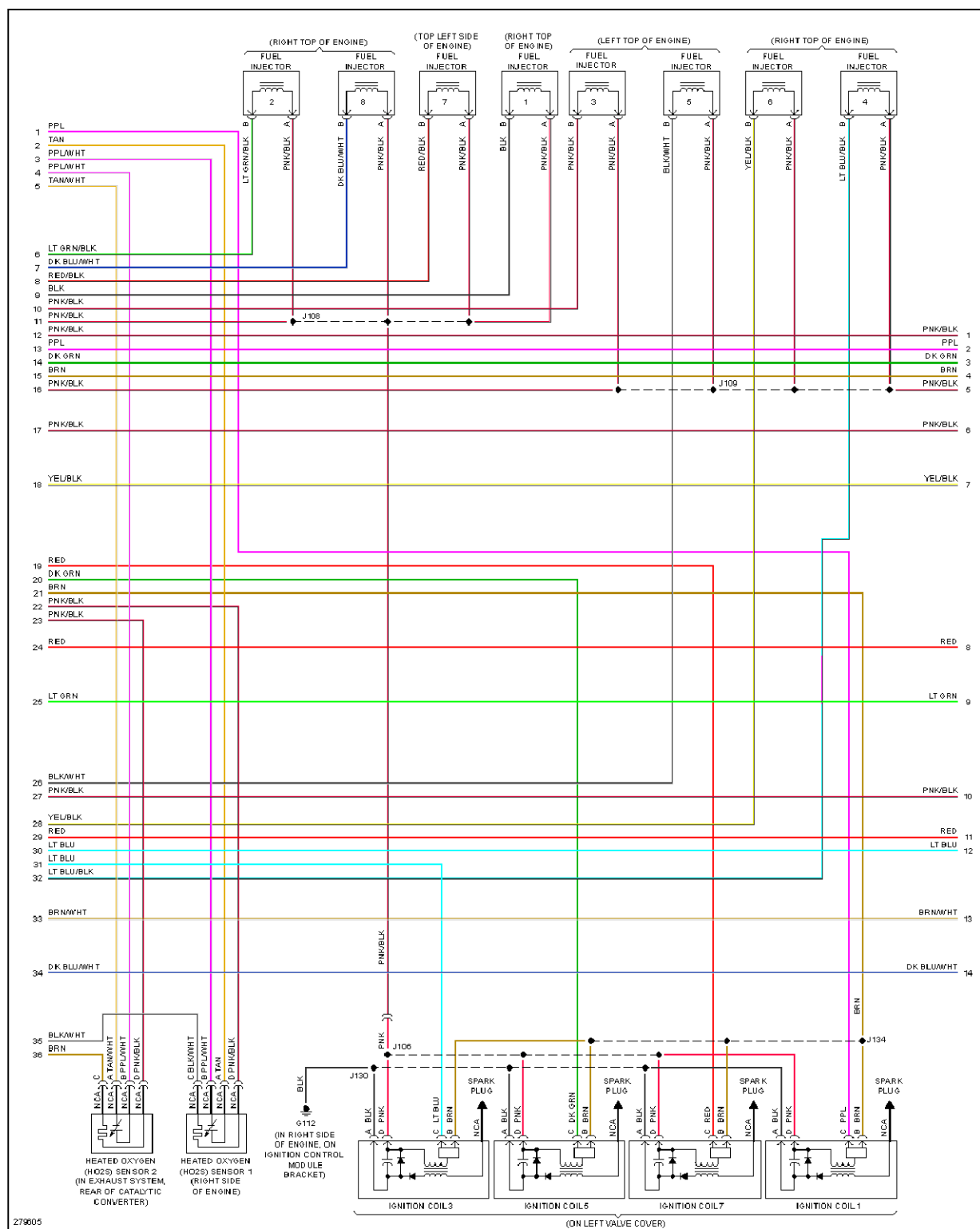
Fig. 34: 5.3L VIN C, Engine Performance Circuit (2 of 5)
