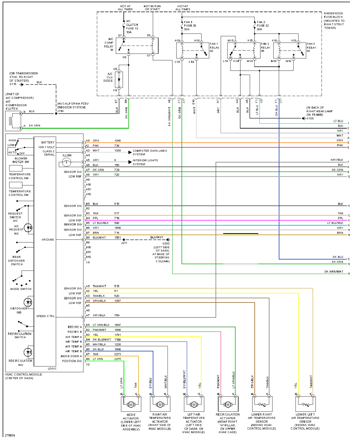
Fig. 4: 3.8L VIN 2, Automatic A/C Circuit (1 of 2)
