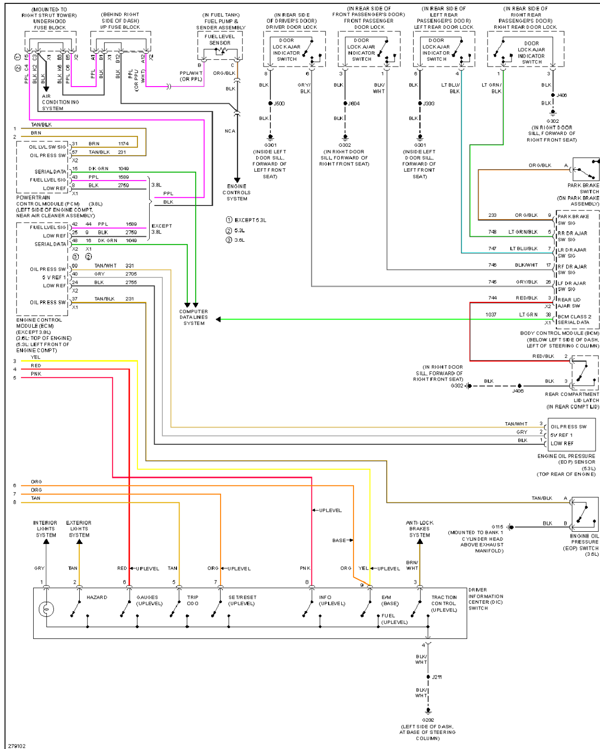
Fig. 50: Instrument Cluster Circuit, W/ Message Center (2 of 2)
