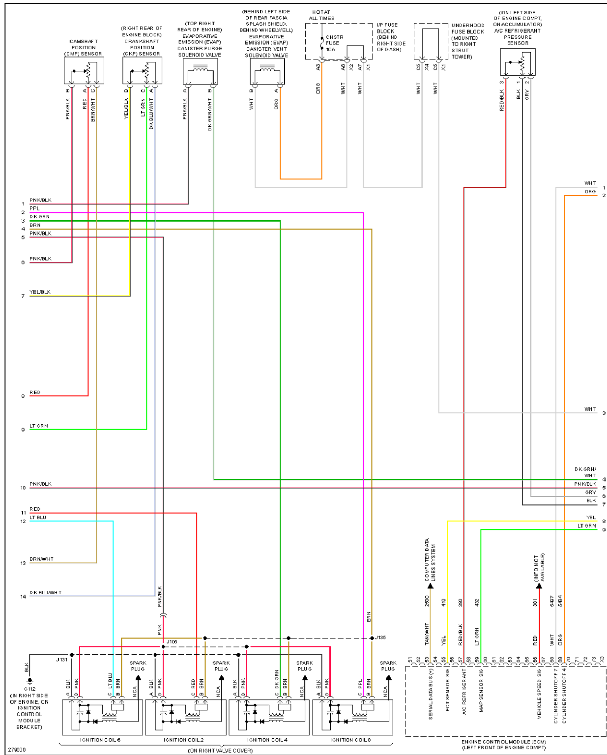
Fig. 35: 5.3L VIN C, Engine Performance Circuit (3 of 5)
