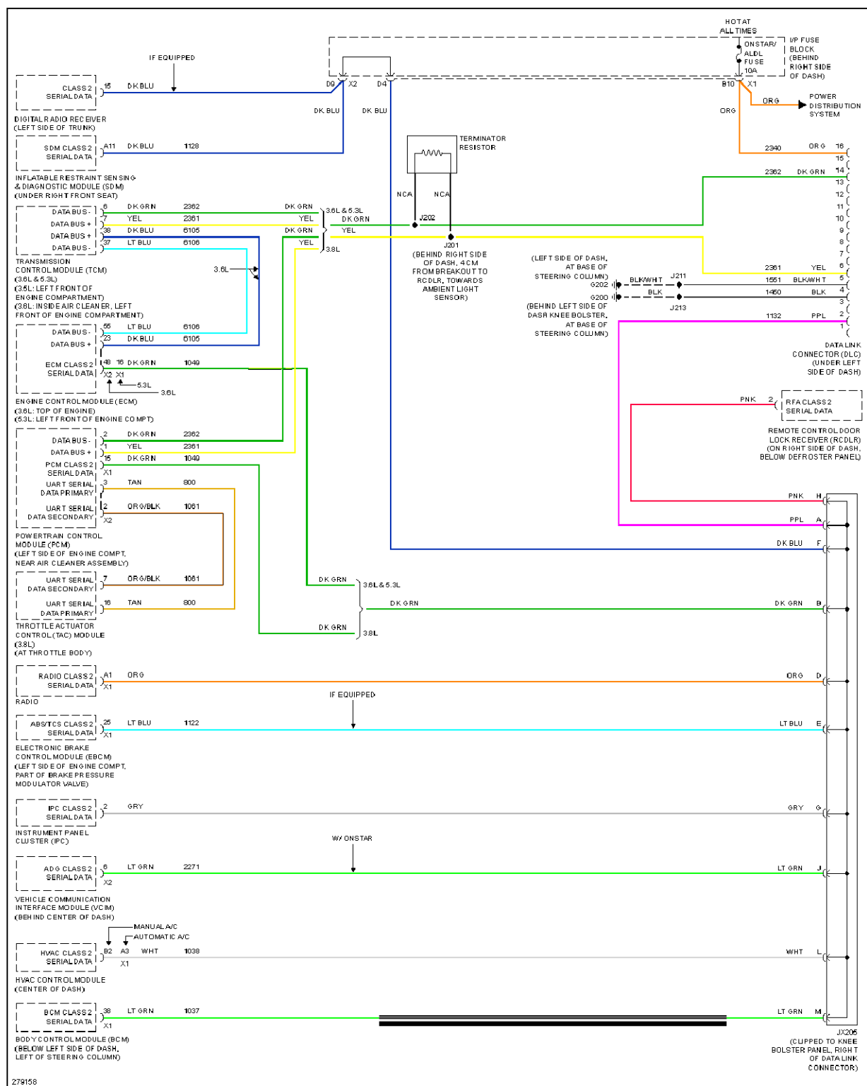
Fig. 15: Computer Data Lines Circuit
