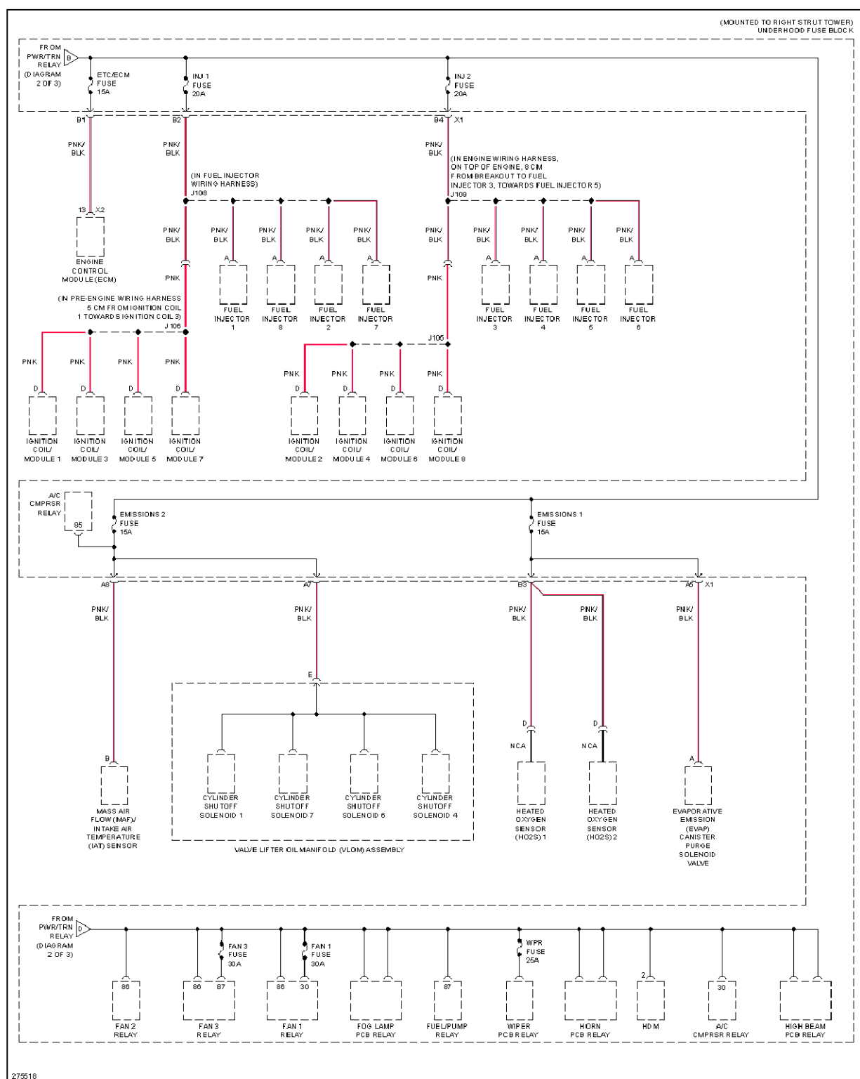
Fig. 66: 5.3L VIN C, Power Distribution Circuit (3 of 3)
