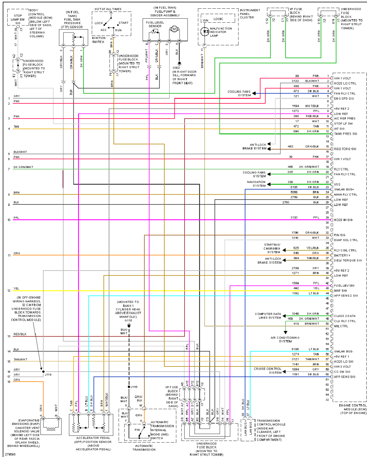
Fig. 27: 3.6L VIN 7, Engine Performance Circuit (4 of 4)
