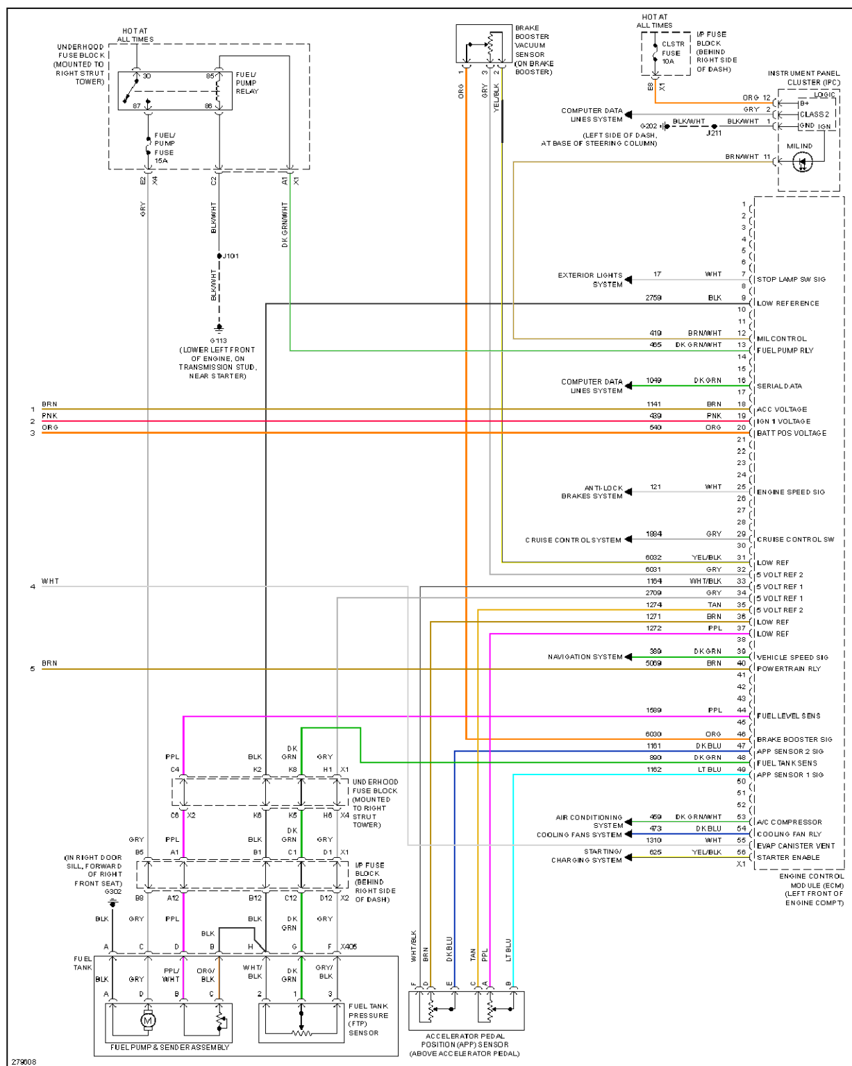
Fig. 37: 5.3L VIN C, Engine Performance Circuit (5 of 5)
