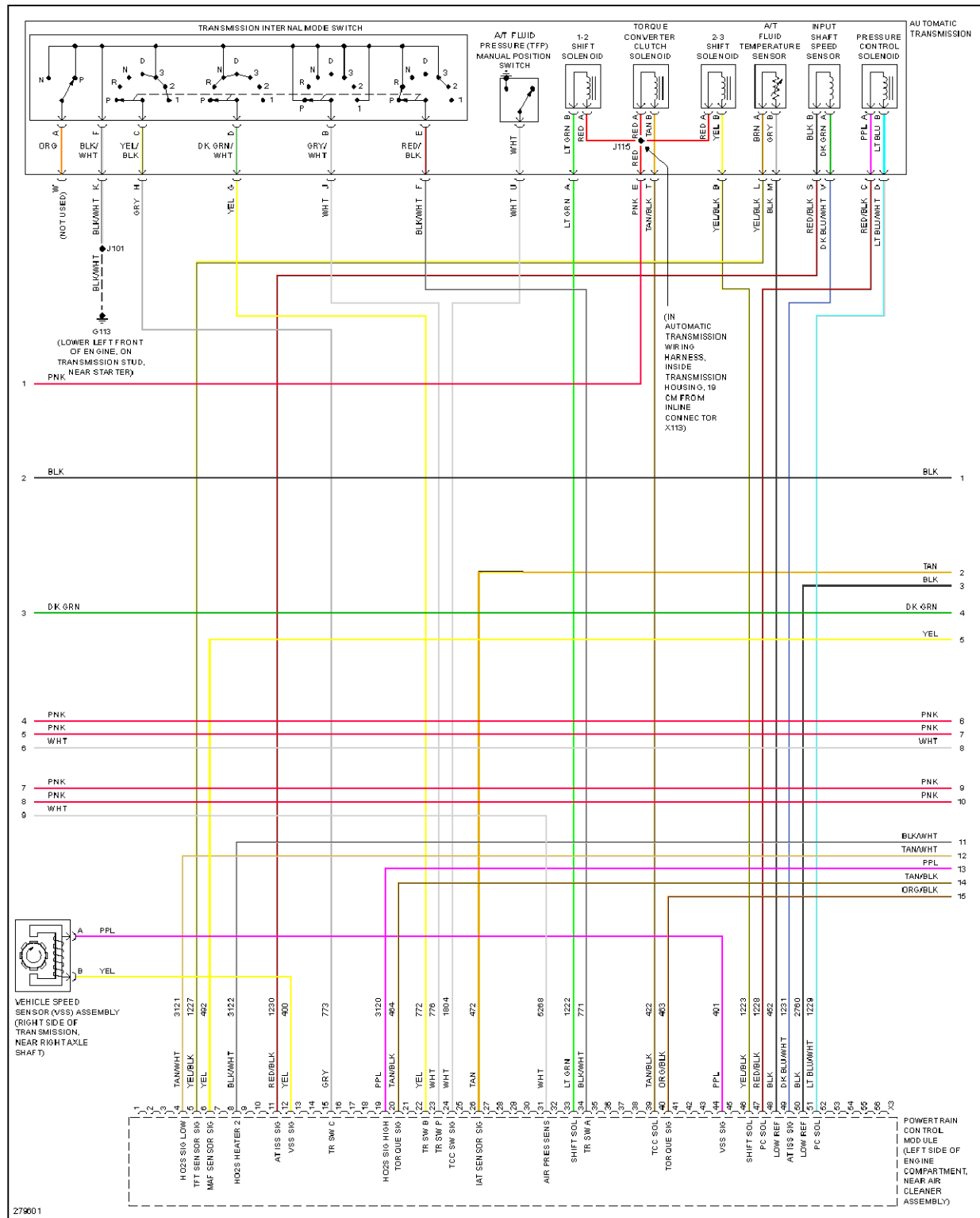
Fig. 30: 3.8L VIN 2, Engine Performance Circuit (3 of 5)
