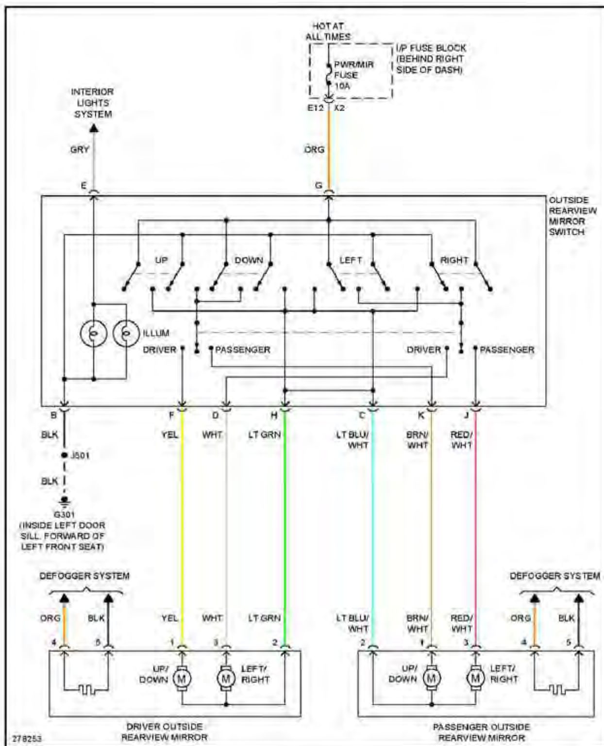
Fig. 69: Power Mirrors Circuit
