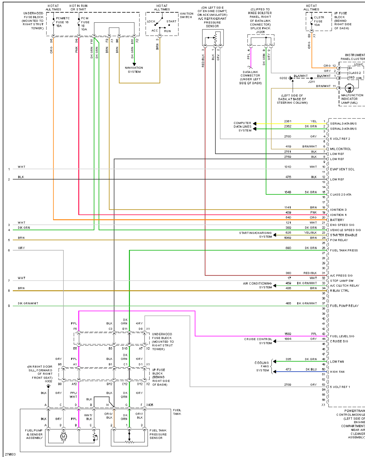
Fig. 32: 3.8L VIN 2, Engine Performance Circuit (5 of 5)
