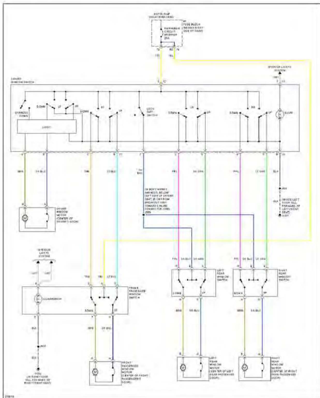
Fig. 75: Power Windows Circuit
