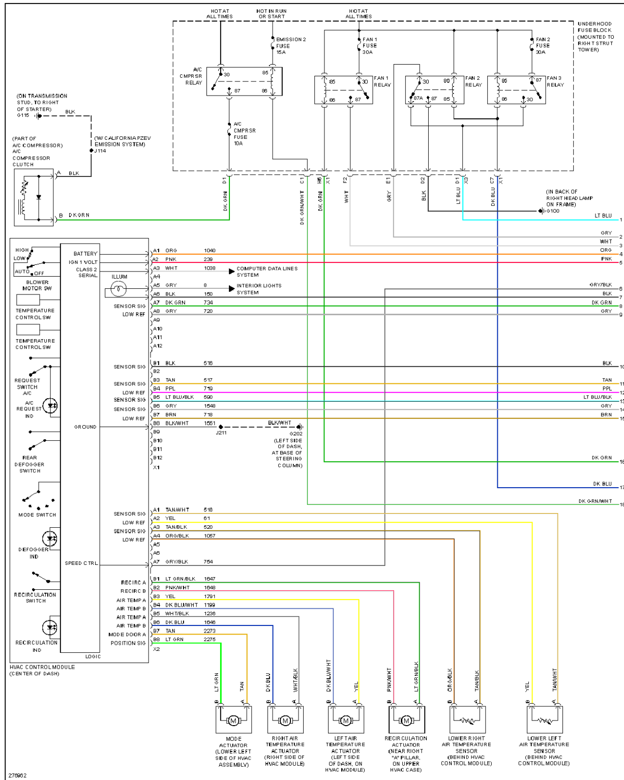
Fig. 7: 5.3L VIN C, Automatic A/C Circuit (1 of 2)
