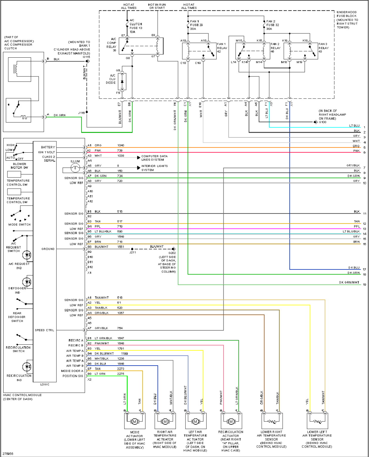
Fig. 1: 3.6L VIN 7, Automatic A/C Circuit (1 of 2)
