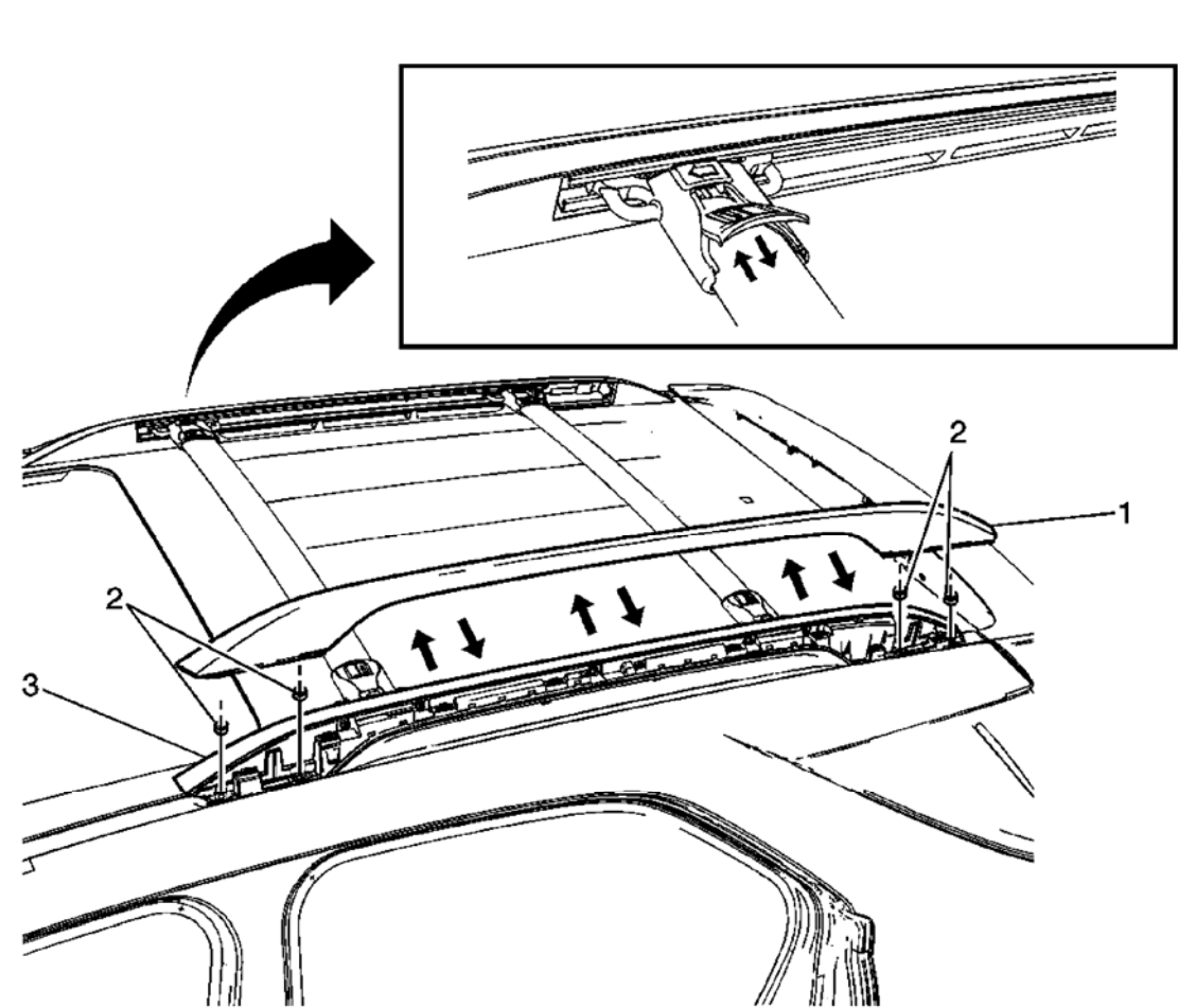
Fig. 1: Identifying Luggage Carrier Side Rail Components Courtesy of GENERAL MOTORS CORP.
