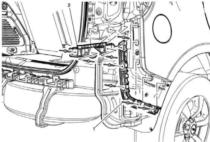
Rear Bumper Fascia Guide Replacement - Right Side
