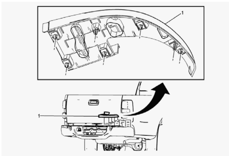
Rear Bumper Step Outer Pad Replacement
