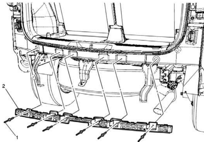
Rear Bumper Fascia Guide Replacement
