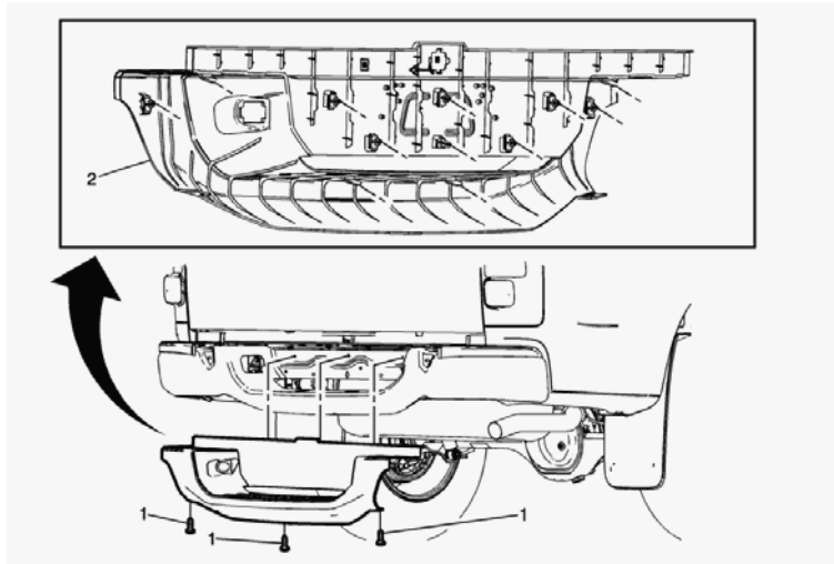
Rear Bumper Step Center Pad Replacement
