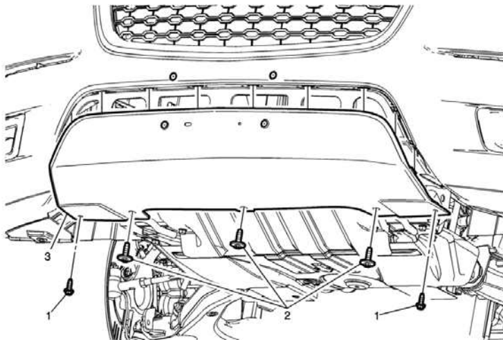
Front Bumper Lower Fascia Trim Insert Replacement
