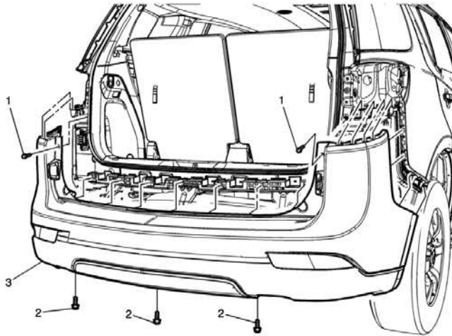
Rear Bumper Fascia Replacement
