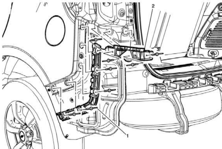
Rear Bumper Fascia Guide Replacement - Left Side
