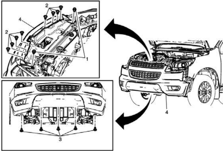
Front Bumper Fascia Replacement
