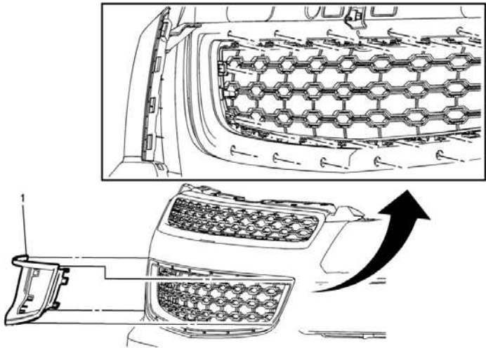
Front Bumper Fascia Lower Molding Replacement
