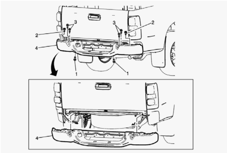
Rear Bumper Impact Bar Replacement
