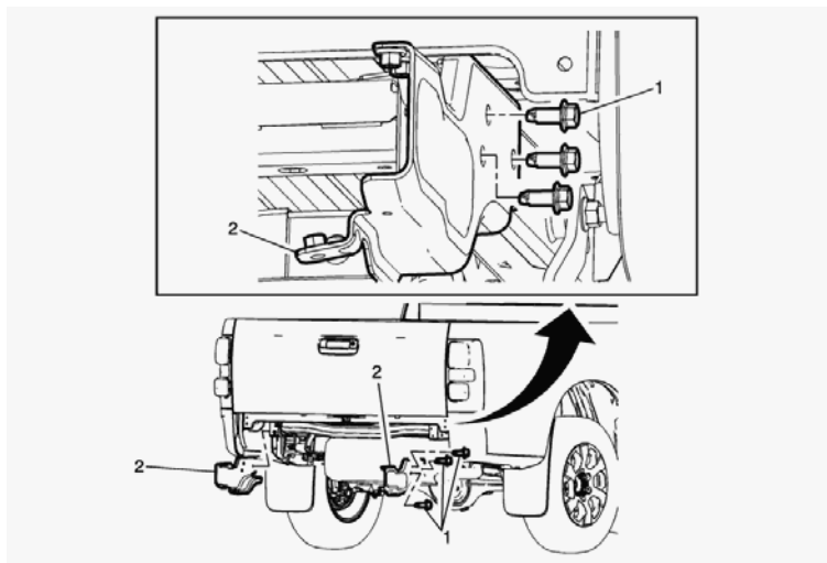
Rear Bumper Impact Bar Bracket Replacement
