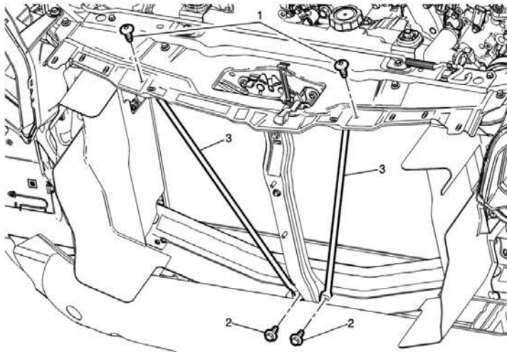
Front Bumper Fascia Brace Replacement
