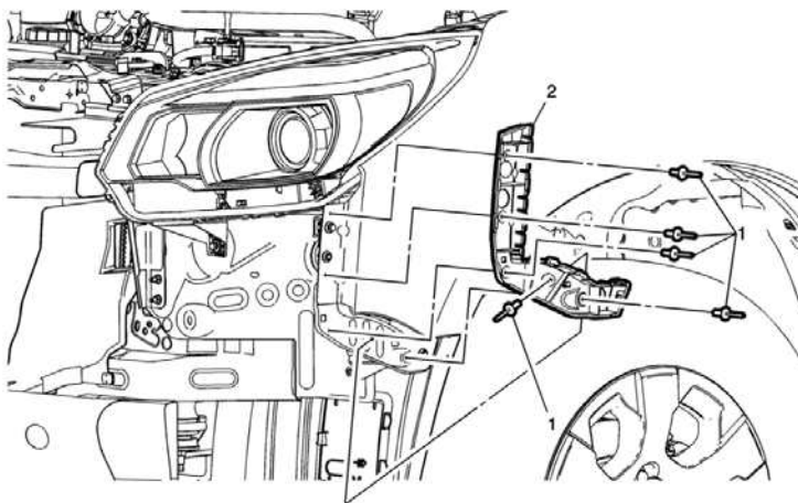
Front Bumper Fascia Guide Replacement
