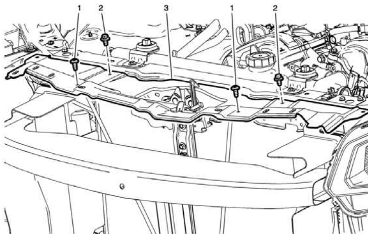
Front Grille Support Reinforcement Replacement
