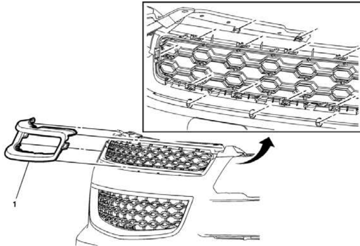
Front Bumper Fascia Upper Molding Replacement
