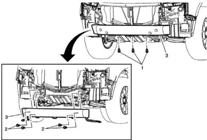
Front Bumper Lower Impact Bar Replacement
