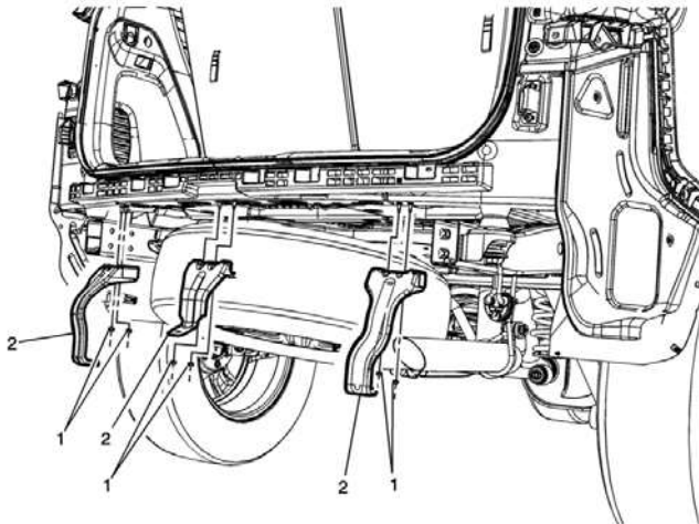
Rear Bumper Fascia Lower Reinforcement Replacement
