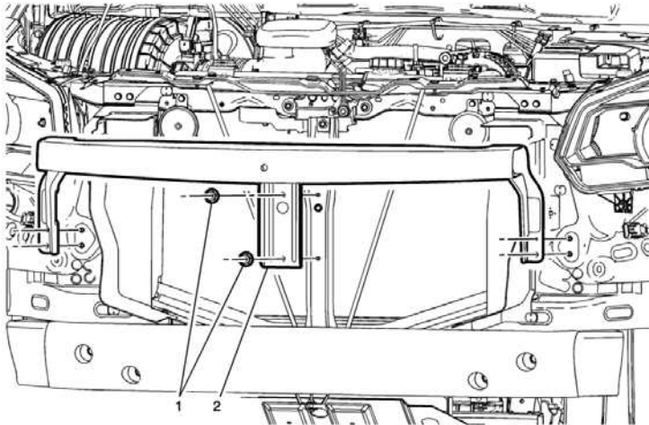
Front Bumper Upper Impact Bar Replacement
