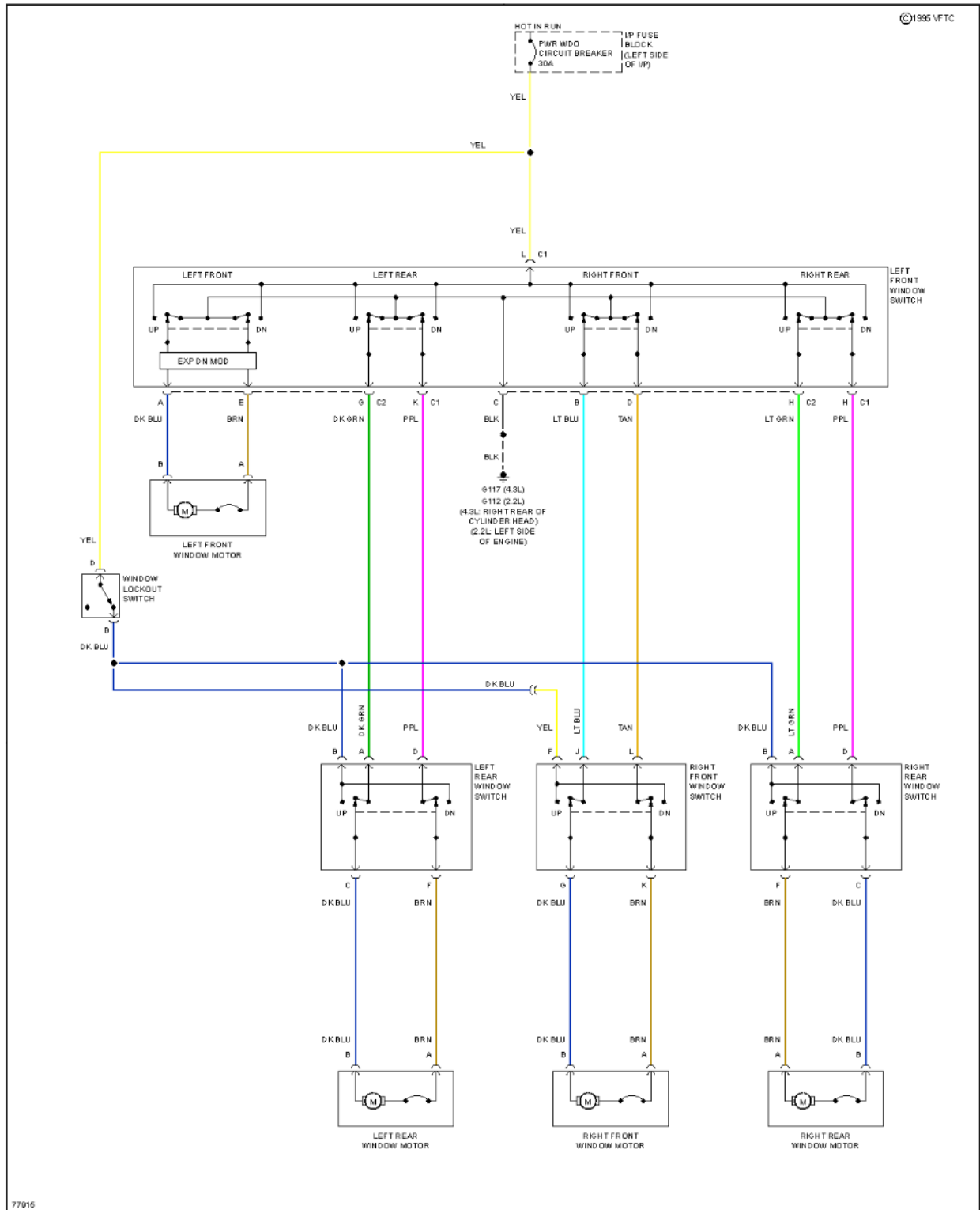
Fig. 29: Power Window Circuit, 4 Door
