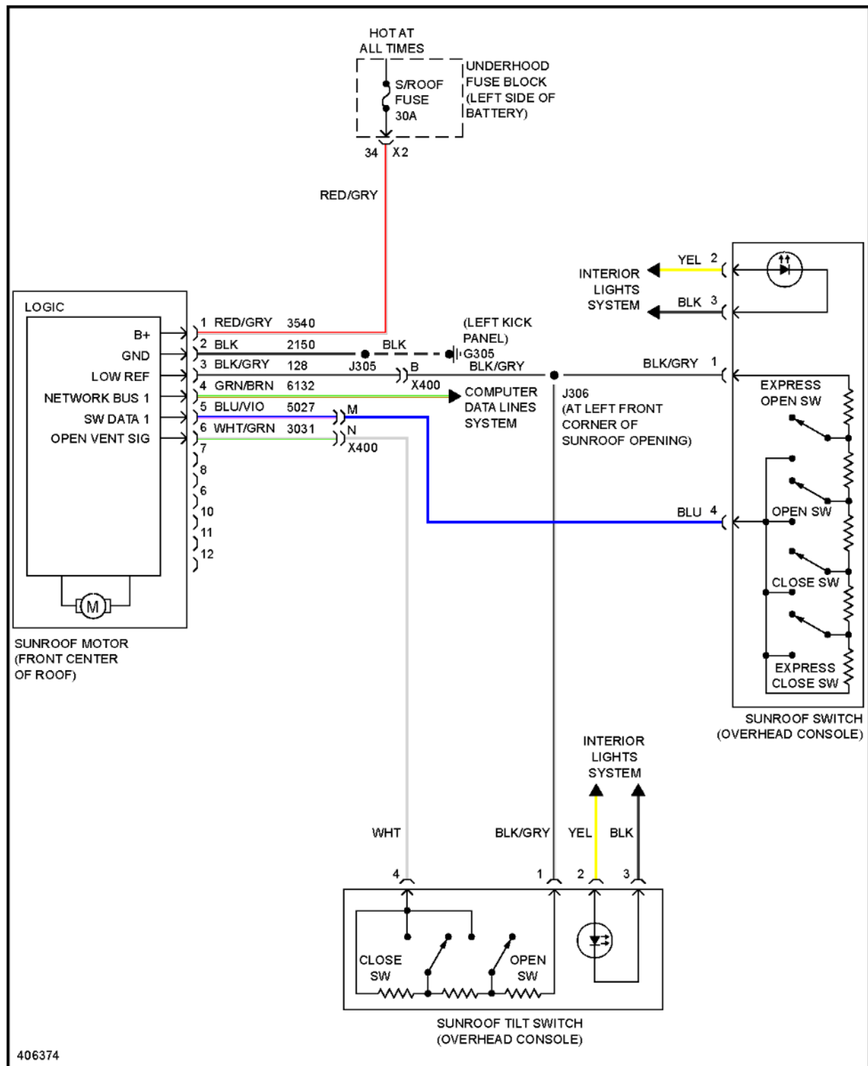
Fig. 110: Power Top/Sunroof Circuit
