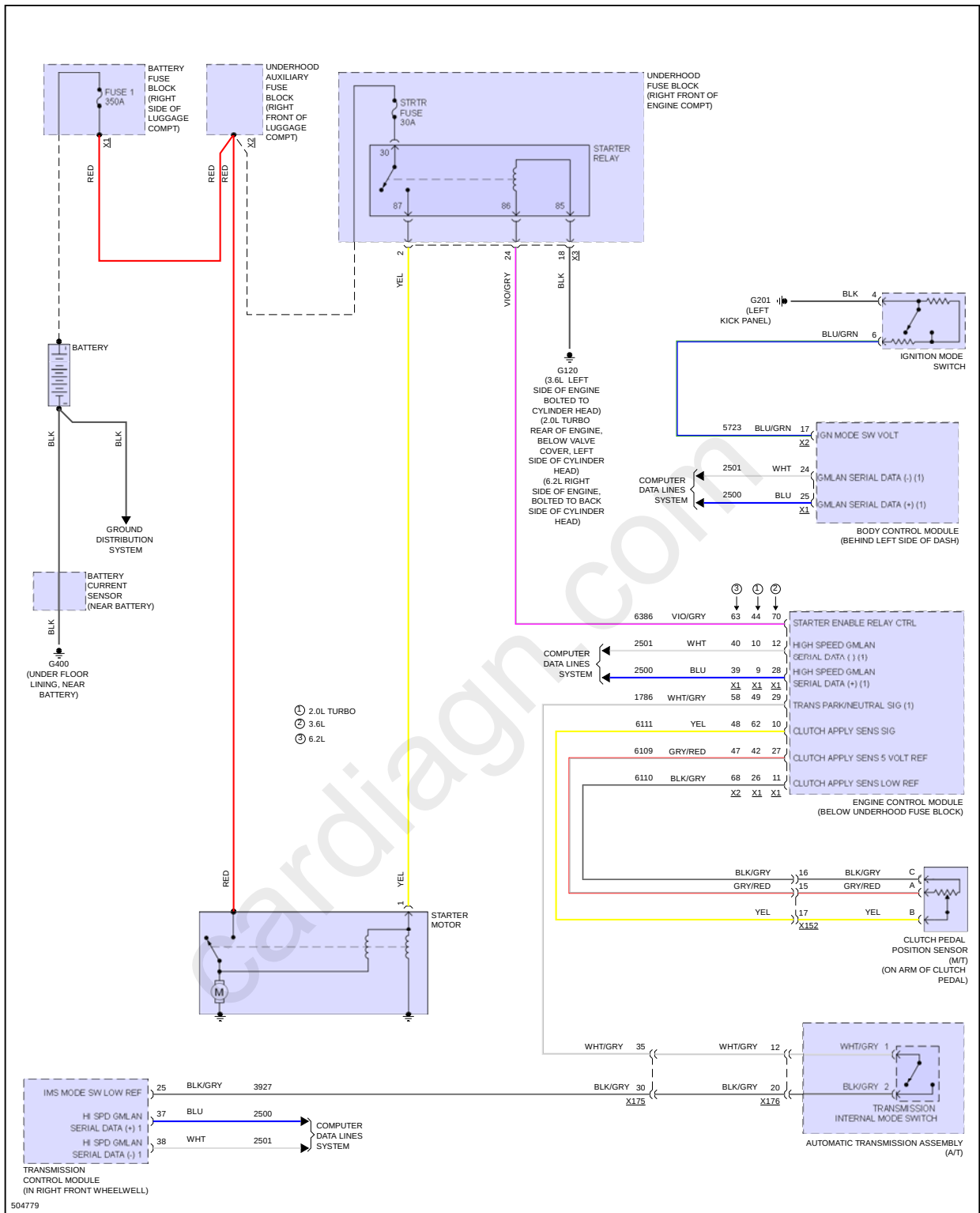
Fig 2: Starting Circuit
