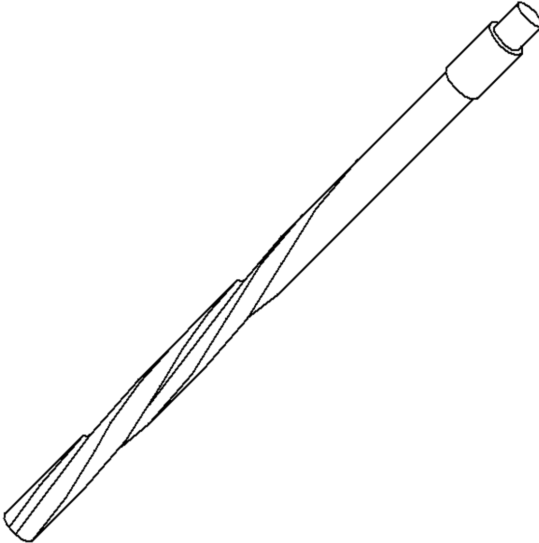
J 42096 Valve Guide Reamer
