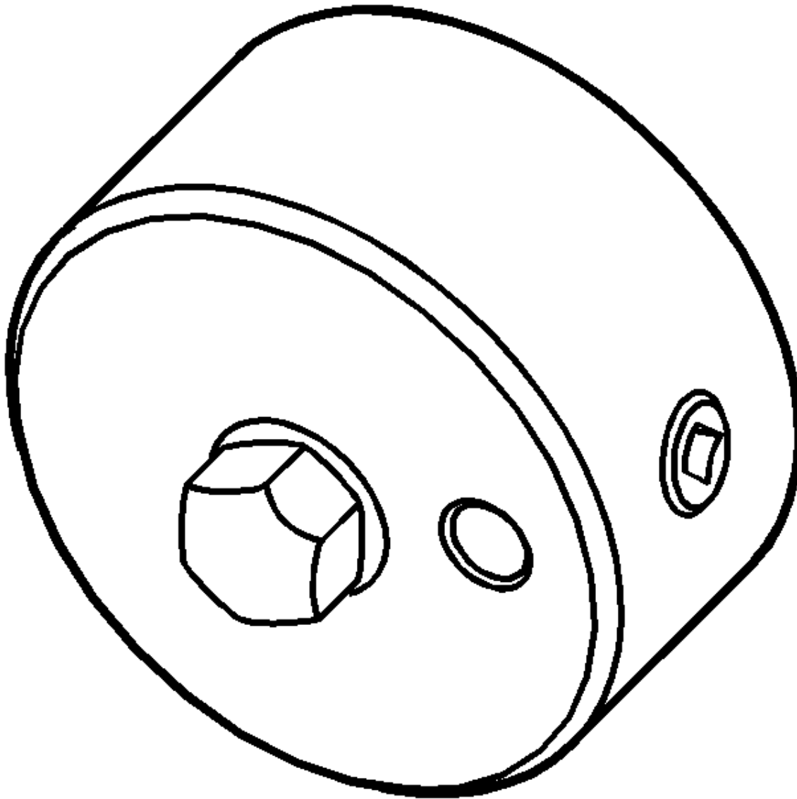
EN 47971 Oil Pressure Gauge Adapter
