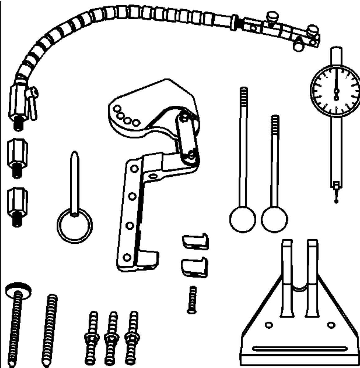
J 43690-A Rod Bearing Clearance Check Tool
