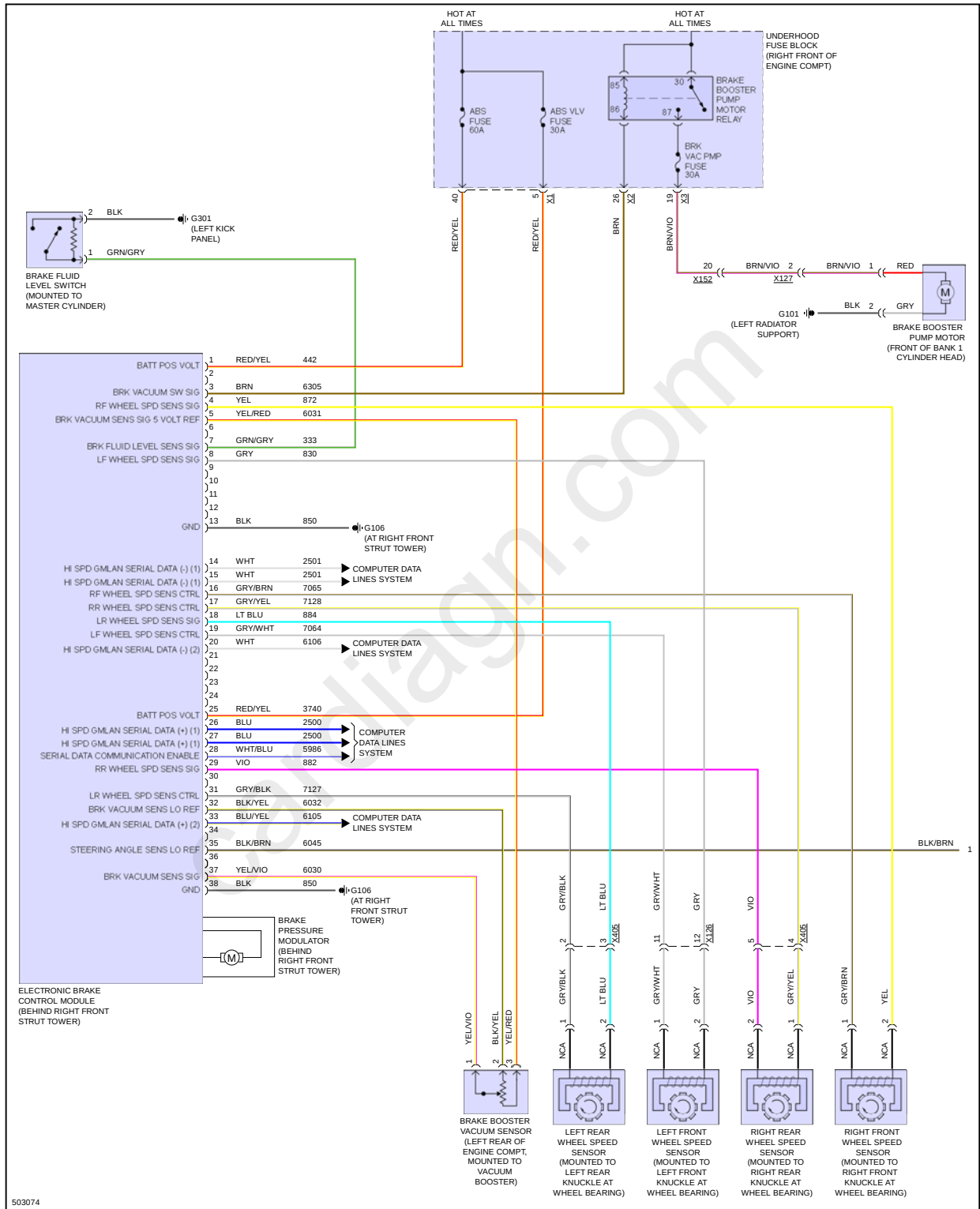
Fig 1: 6.2L VIN 7, Anti-lock Brakes Circuit (1 of 2)
