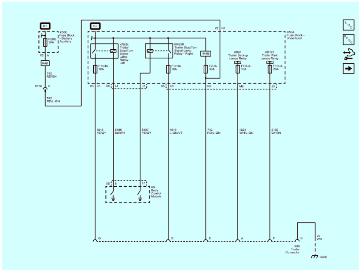
Fig. 1: Trailer Connector Pins: A, B, D, E, F, G (Z82 without 8S3 or UY2)
