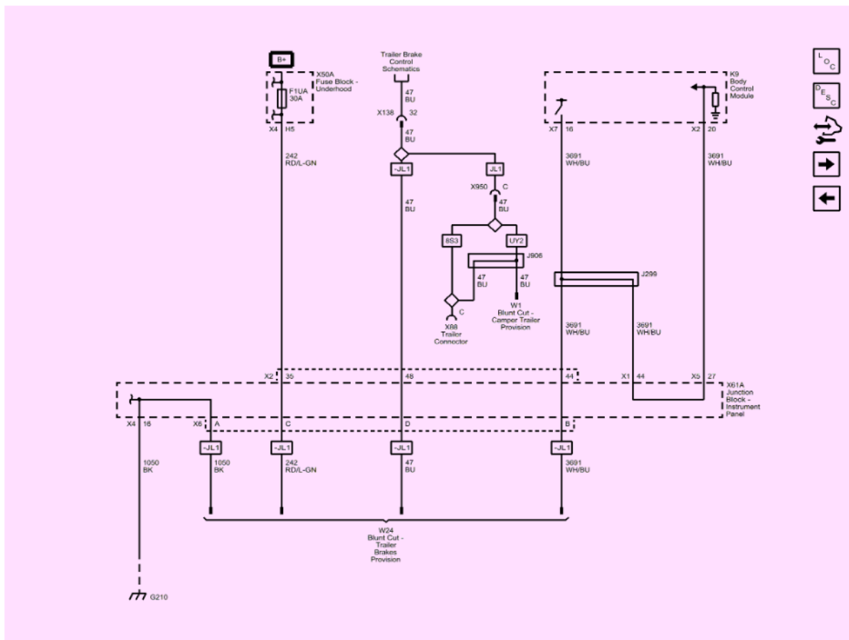
Fig. 4: Trailer Connector Pin: C (Z82 with 8S3 or UY2 except E29)
