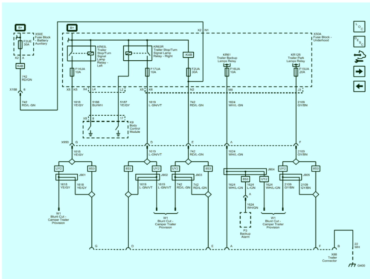
Fig. 2: Trailer Connector Pins: A, B, D, E, F, G (Z82 with 8S3 or UY2)
